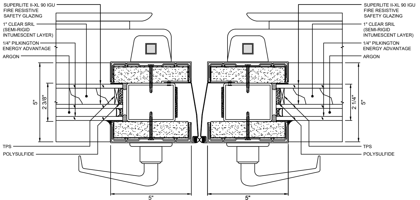
A MEETING STILES 6 WITH SUPERLITE II-XL 90 IGU
