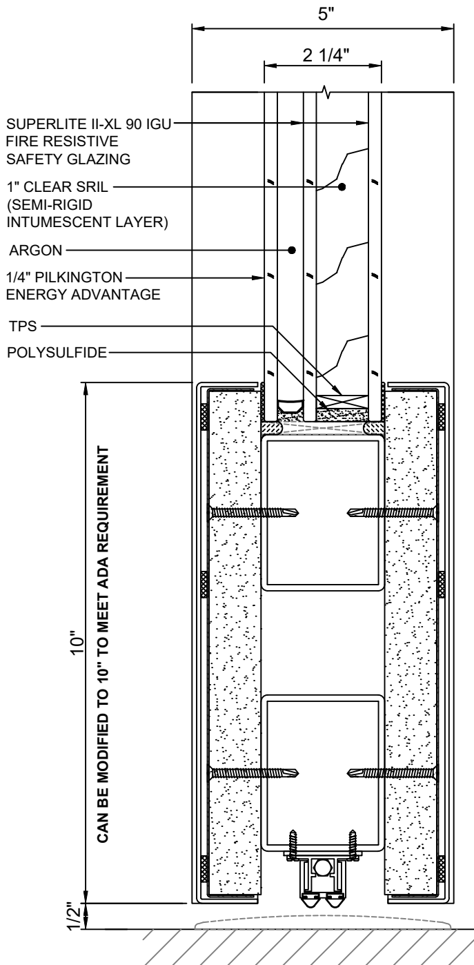
A 3 DOOR BOTTOM RAIL WITH DOOR BOTTOM WITH SUPERLITE II-XL 90 IGU
