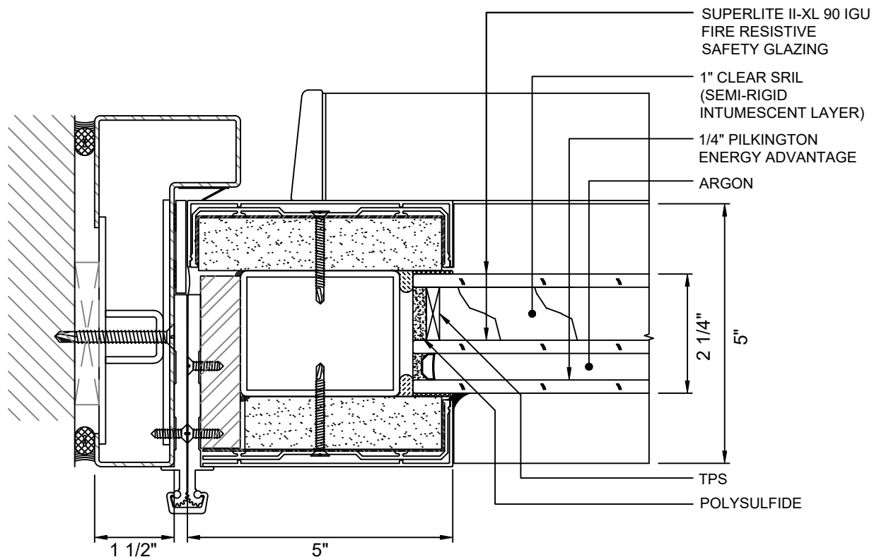
A 5 DOOR JAMB AT HINGE WITH SUPERLITE II-XL 90 IGU
