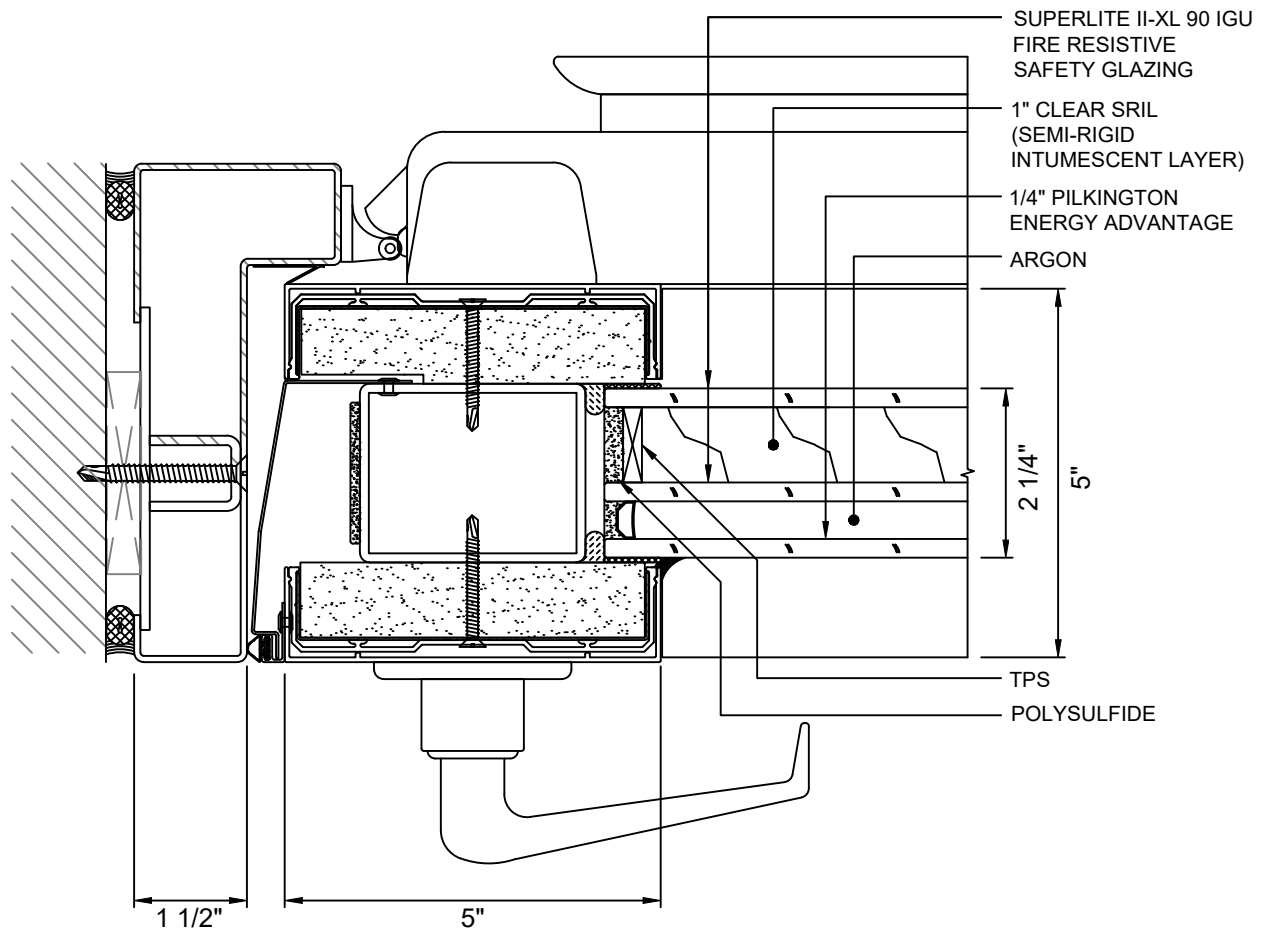
A 4 DOOR JAMB AT LOCK WITH SUPERLITE II-XL 90 IGU
