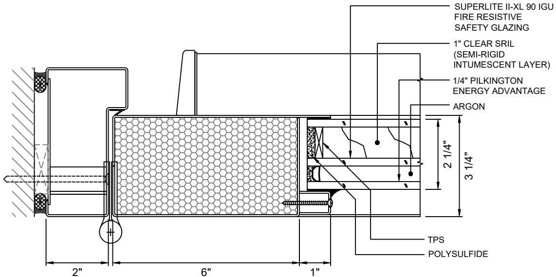
A 5 DOOR JAMB AT HINGE - STANDARD WITH SUPERLITE II-XL90 IGU
