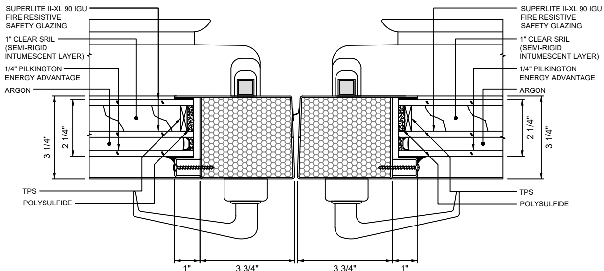
B MEETING STILES - NARROW STYLE 6 WITH SUPERLITE II-XL 90 IGU
