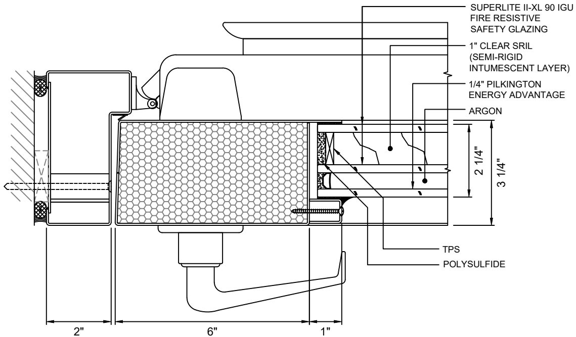
A 4 DOOR JAMB AT LOCK - STANDARD WITH SUPERLITE II-XL 90 IGU
