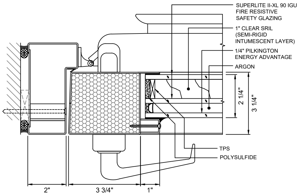
B 4 DOOR JAMB AT LOCK - NARROW STYLE WITH SUPERLITE II-XL 90 IGU
