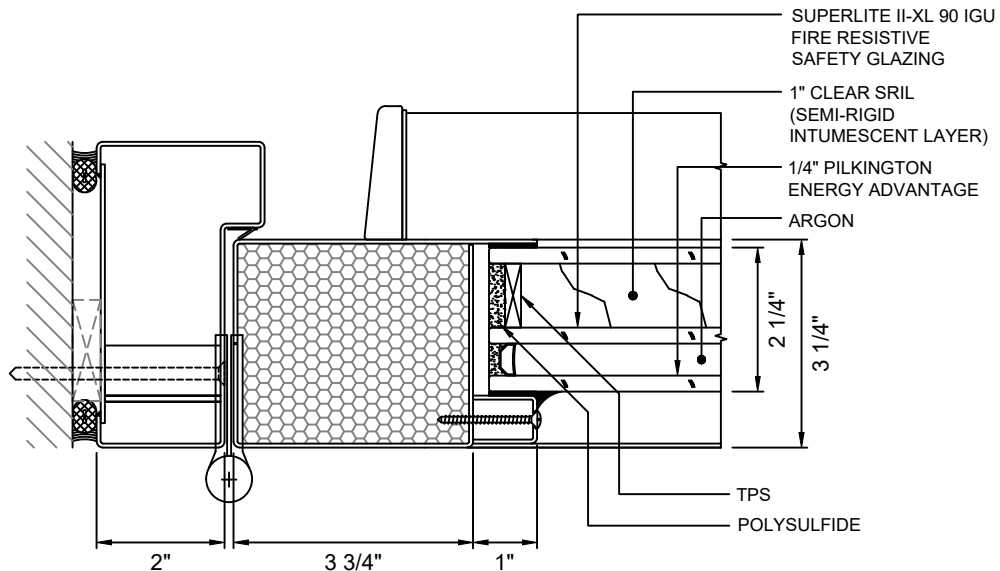
B 5 DOOR JAMB AT HINGE - NARROW STYLE WITH SUPERLITE II-XL90 IGU
