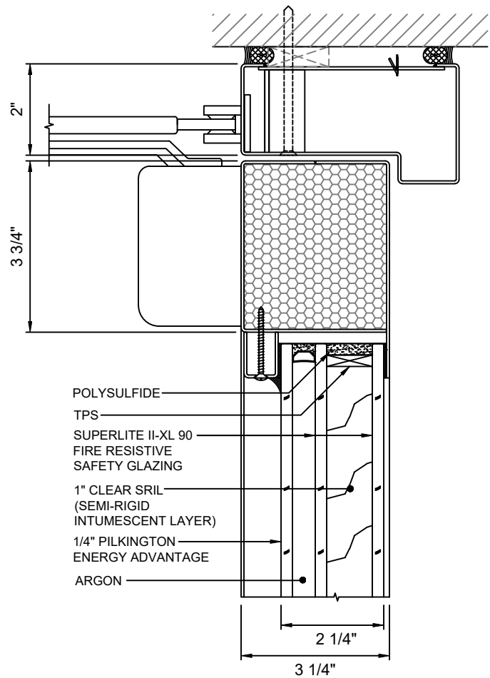
B DOOR TOP RAIL - NARROW STYLE WITH SUPERLITE II-XL 90 IGU
