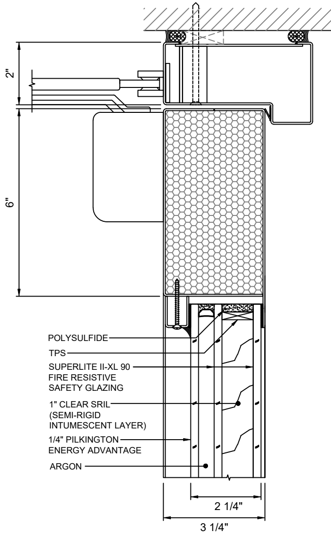
A DOOR TOP RAIL - STANDARD WITH SUPERLITE II-XL 90 IGU
