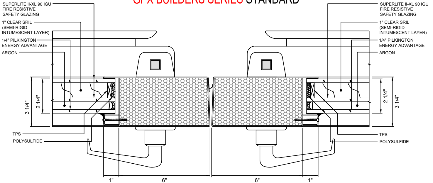
A MEETING STILES - STANDARD 6 WITH SUPERLITE II-XL 90 IGU
