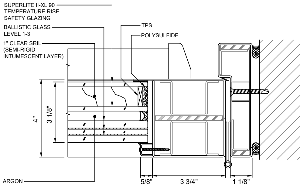
(B) 5 DOOR JAMB AT HINGE - NARROW STYLE WITH SUPERLITE II-XL 90 WITH LEVEL 1-3 BALLISTIC GLASS
