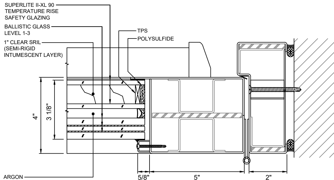
(A) 5 DOOR JAMB AT HINGE - STANDARD WITH SUPERLITE II-XL 90 WITH LEVEL 1-3 BALLISTIC GLASS
