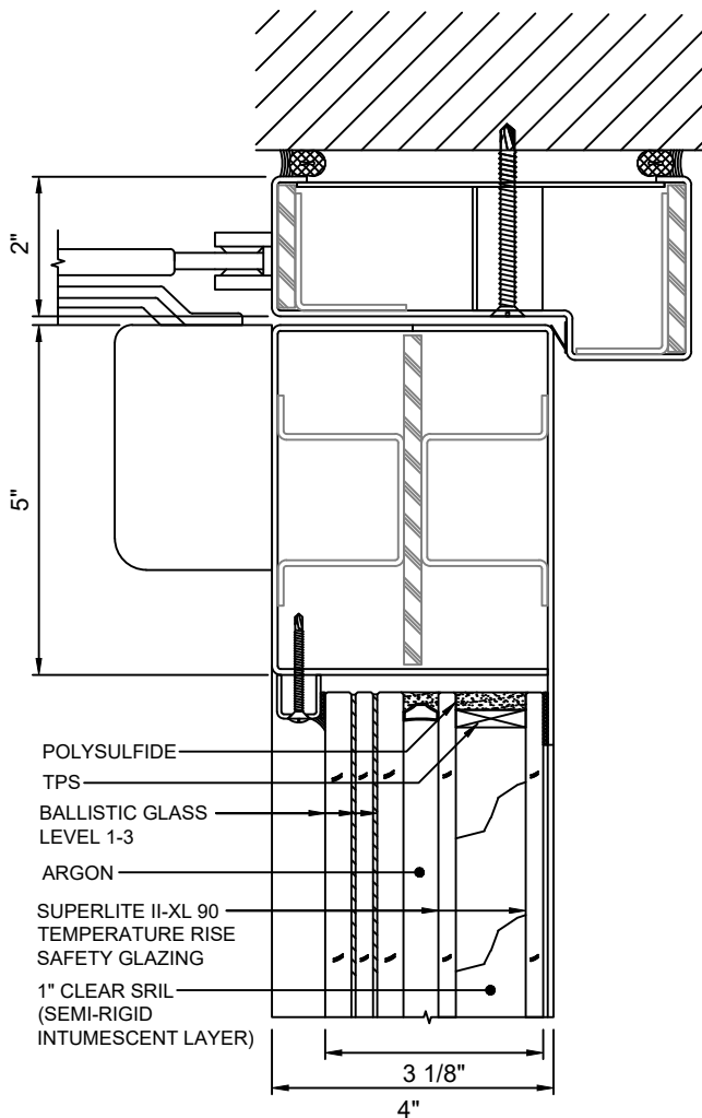
A 2 DOOR TOP RAIL - STANDARD WITH SUPERLITE II-XL 90 WITH LEVEL 1-3 BALLISTIC GLASS
