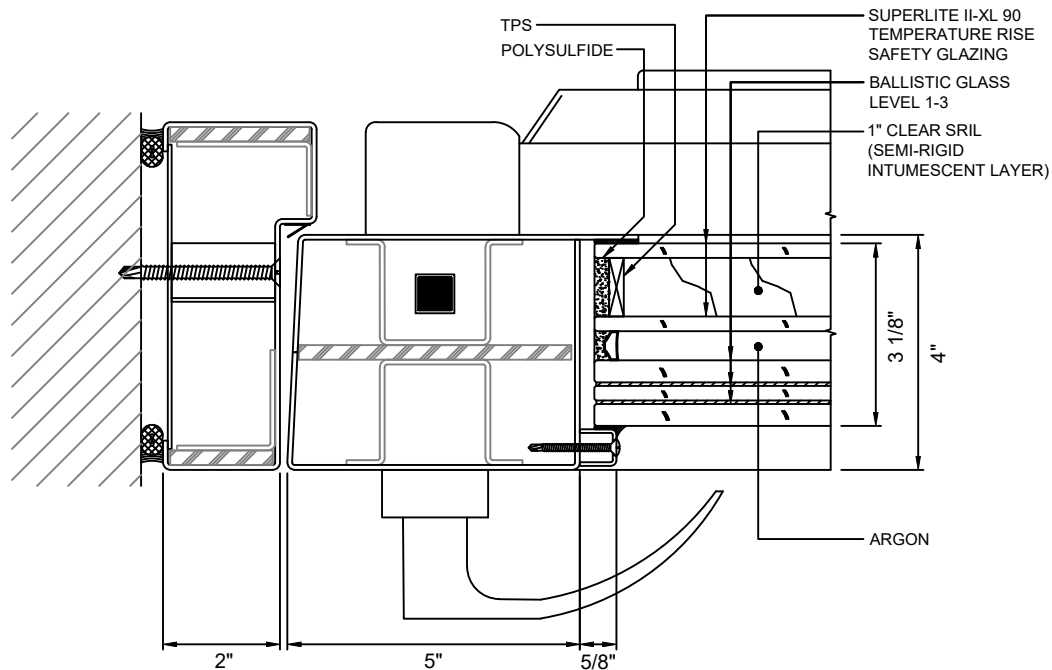
A DOOR JAMB AT LOCK - STANDARD WITH SUPERLITE II-XL 90 WITH LEVEL 1-3 BALLISTIC GLASS
