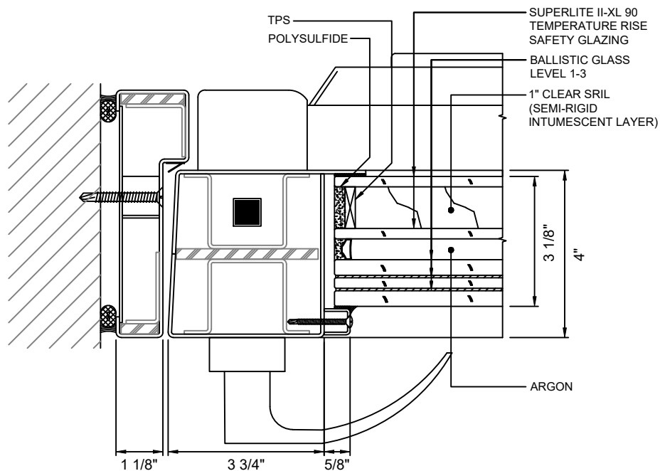
B DOOR JAMB AT LOCK - NARROW STYLE WITH SUPERLITE II-XL 90 WITH LEVEL 1-3 BALLISTIC GLASS
