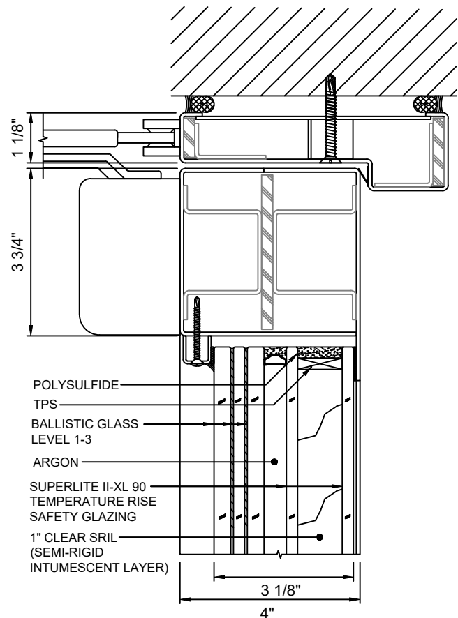
B 2 DOOR TOP RAIL - NARROW STYLE WITH SUPERLITE II-XL 90 WITH LEVEL 1-3 BALLISTIC GLASS
