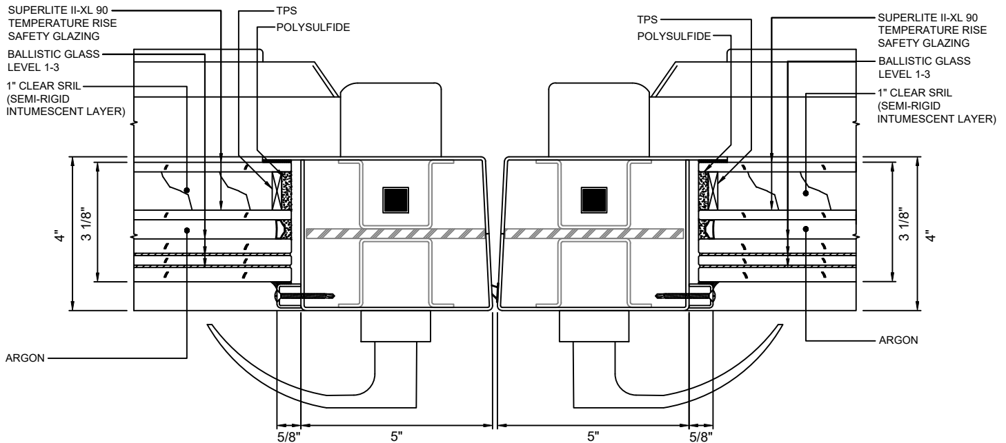
(A) MEETING STILES - STANDARD 6 WITH SUPERLITE II-XL 90 WITH LEVEL 1-3 BALLISTIC GLASS
