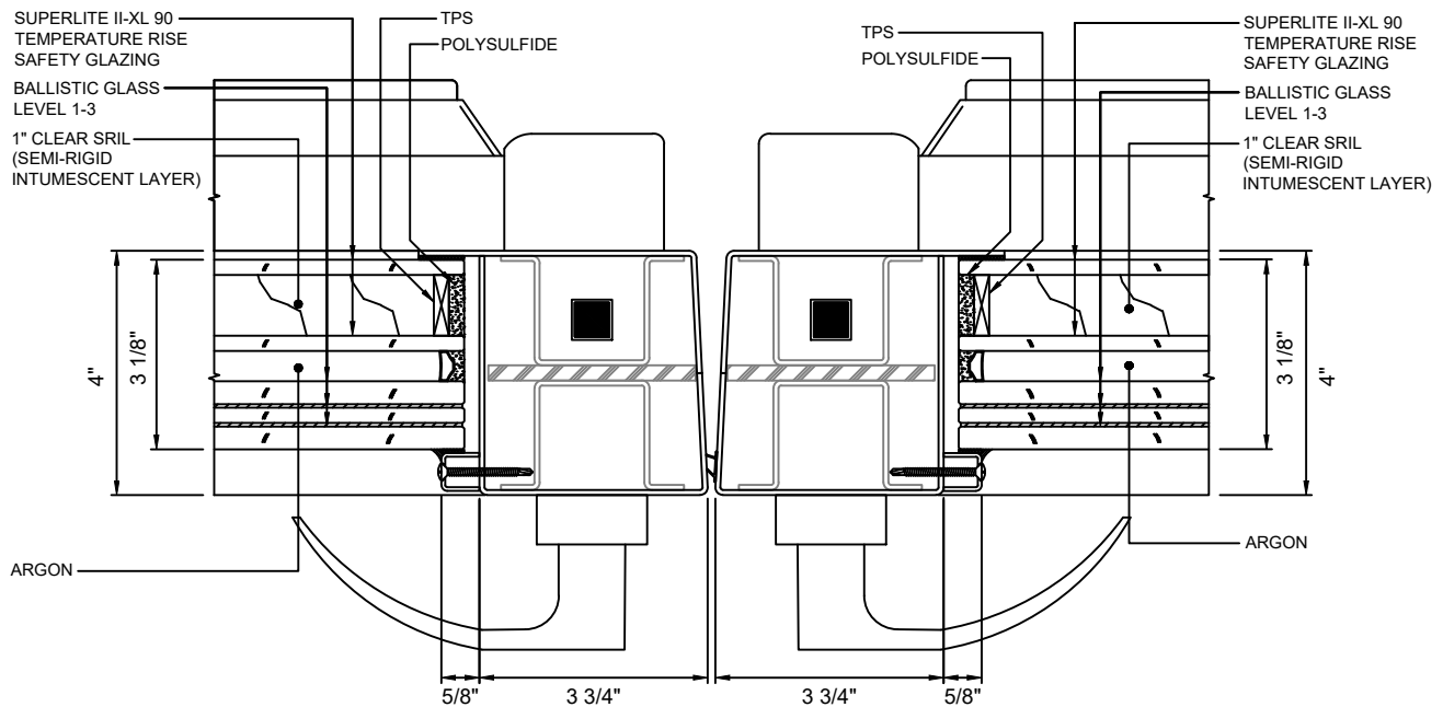
(B) MEETING STILES - NARROW STYLE 6 WITH SUPERLITE II-XL 90 WITH LEVEL 1-3 BALLISTIC GLASS
