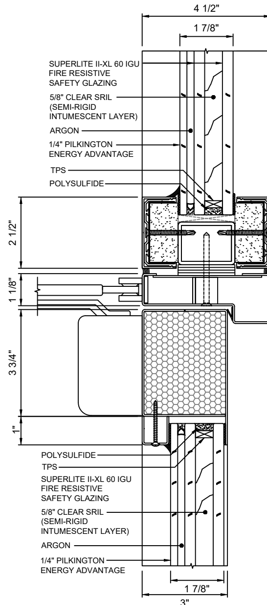
E 13 DOOR TOP RAIL - NARROW STYLE WITH SUPERLITE II-XL 60 IGU
