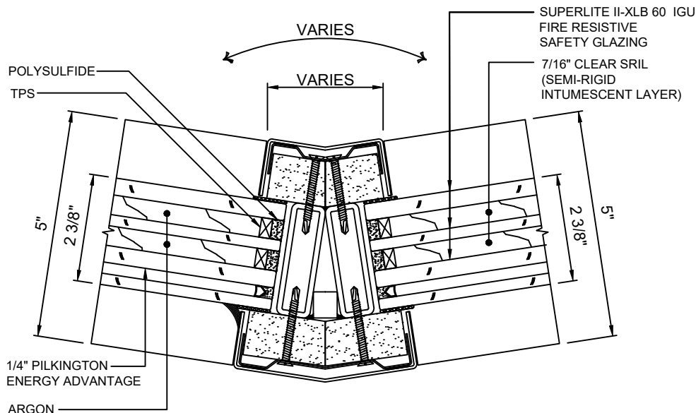
B 11 SEGMENTED VERTICAL WITH SUPERLITE II-XLB 60 IGU
