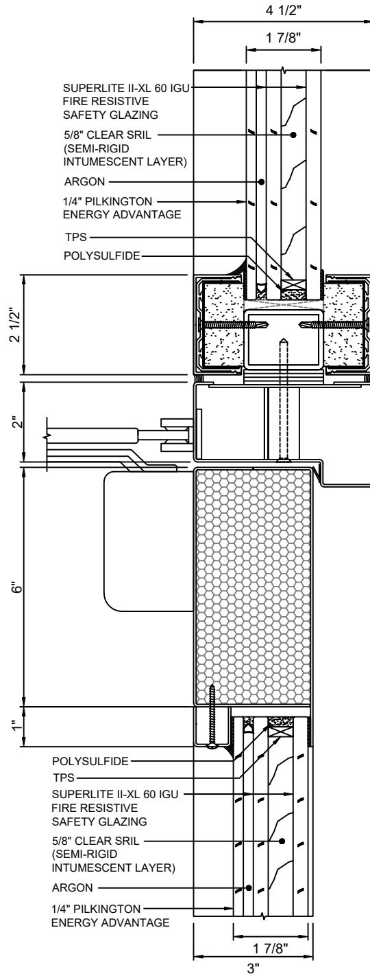
D 13 DOOR TOP RAIL - STANDARD WITH SUPERLITE II-XL 60 IGU
