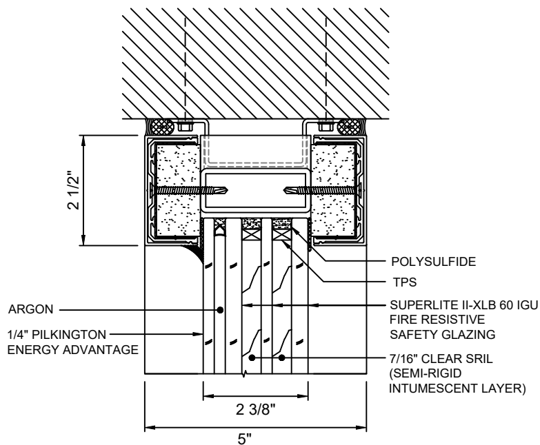
B 5 HEAD DETAIL WITH SUPERLITE II-XLB 60 IGU
