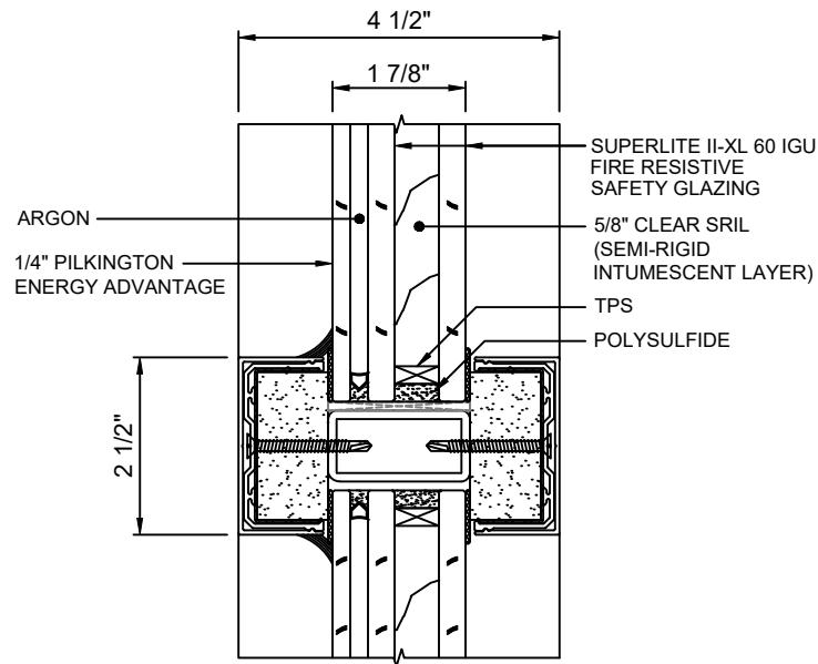
A 6 HORIZONTAL MULLION WITH SUPERLITE II-XL 60 IGU
