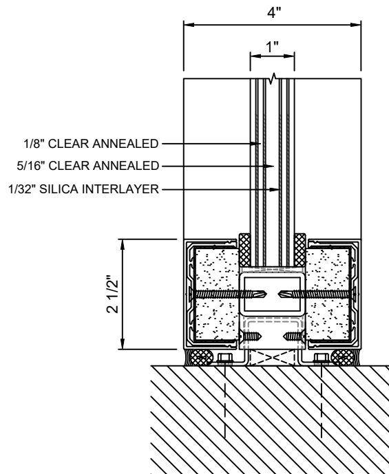
C 7 SILL DETAIL WITH SUPERLITE II-XLM 60
