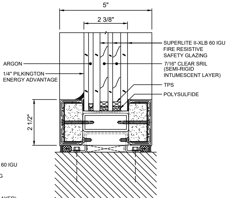
B 7 SILL DETAIL WITH SUPERLITE II-XLB 60
