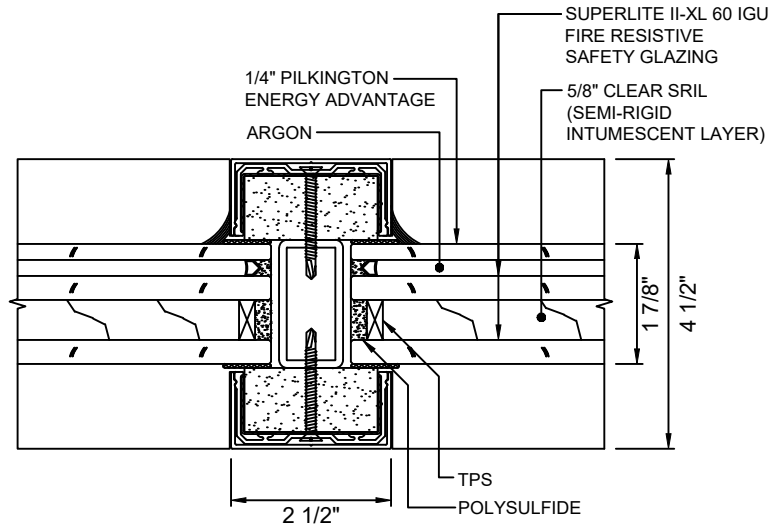
(A) 9 VERTICAL MULLION DETAIL WITH SUPERLITE II-XL 60 IGU
