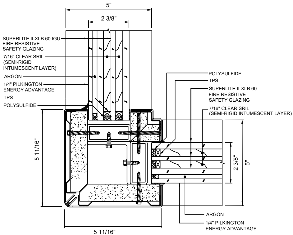
B 90° CORNER DETAIL 10 WITH SUPERLITE II-XLB 60 IGU
