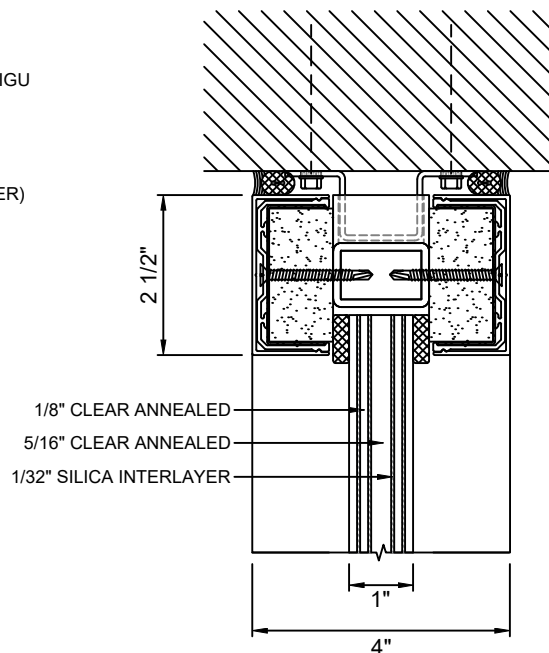
C 5 HEAD DETAIL WITH SUPERLITE II-XLM 60
