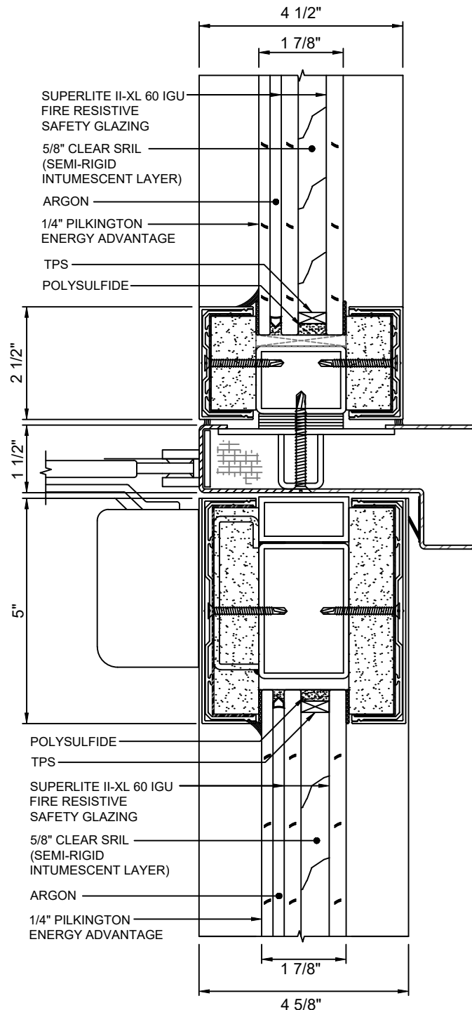
A DOOR TOP RAIL 18 WITH SUPERLITE II-XL 60 IGU
