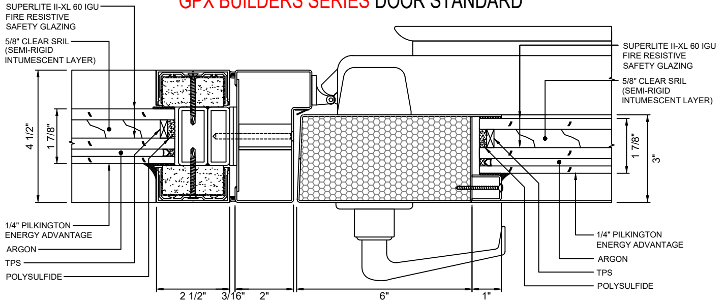
D DOOR JAMB AT LOCK - STANDARD 15 WITH SUPERLITE II-XL 60 IGU
