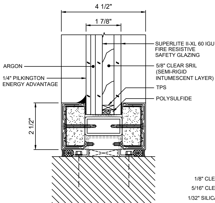
A 7 SILL DETAIL WITH SUPERLITE II-XL 60 IGU
