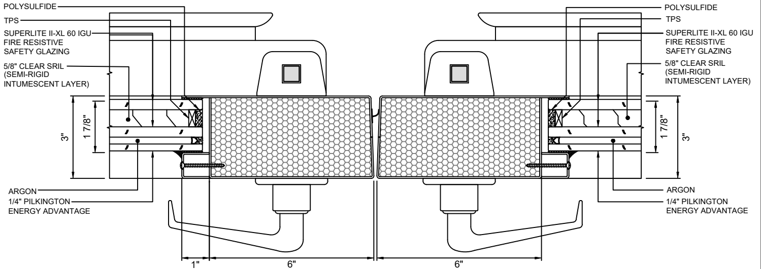
D MEETING STILES - STANDARD WITH SUPERLITE II-XL 60 IGU
