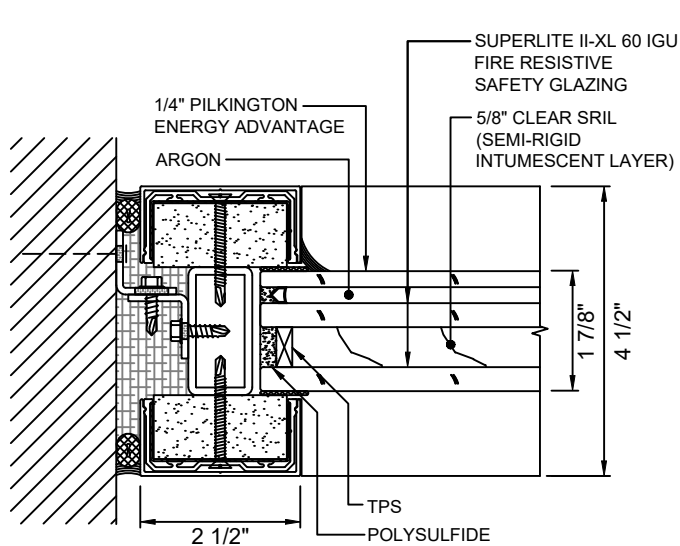
A 8 JAMB DETAIL WITH SUPERLITE II-XL 60 IGU
