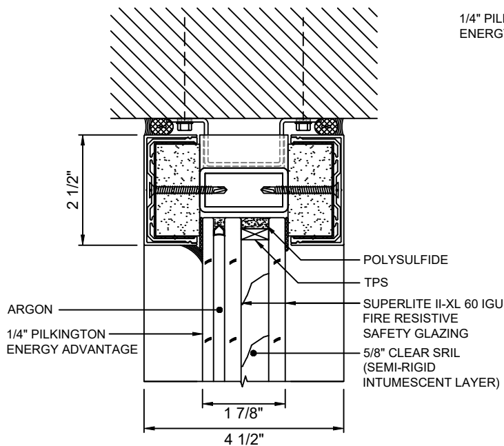
A 5 HEAD DETAIL WITH SUPERLITE II-XL 60 IGU
