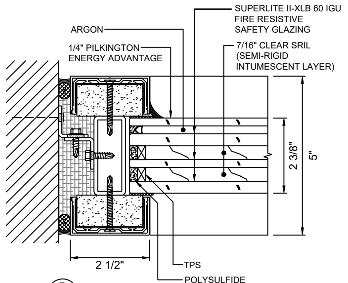
B 8 JAMB DETAIL WITH SUPERLITE II-XLB 60 IGU
