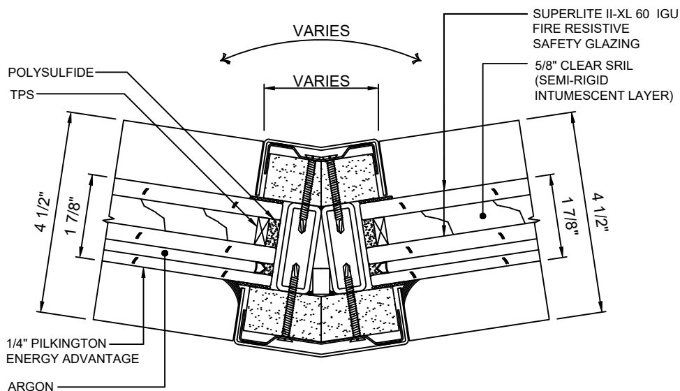
A 11 SEGMENTED VERTICAL WITH SUPERLITE II-XL 60 IGU
