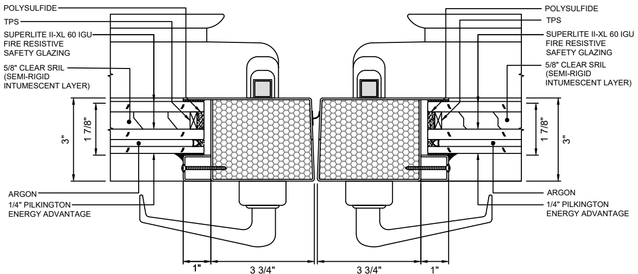
E MEETING STILES - NARROW STYLE WITH SUPERLITE II-XL 60 IGU
