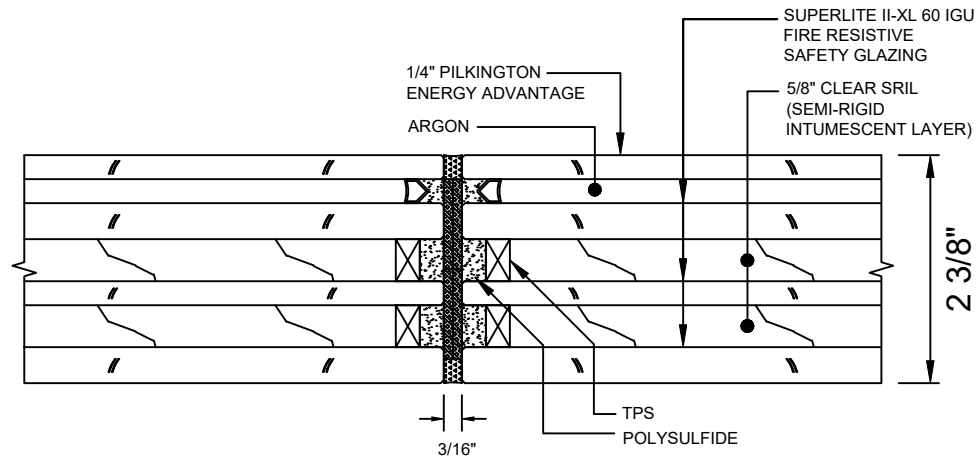
B 12 VERTICAL BUTT JOINT WITH SUPERLITE II-XLB 60 IGU
