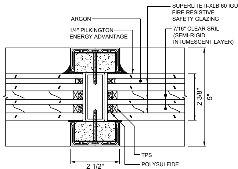
(B) 9 VERTICAL MULLION DETAIL WITH SUPERLITE II-XLB 60 IGU
