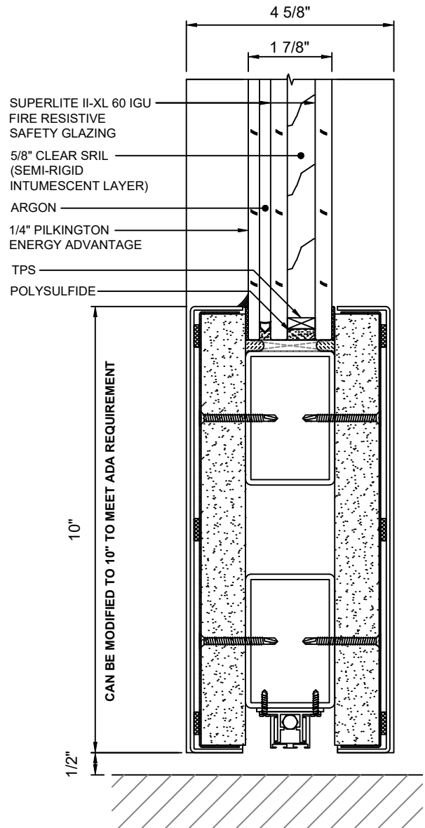
A 19 DOOR BOTTOM RAIL WITH DOOR BOTTOM WITH SUPERLITE II-XL 60 IGU
