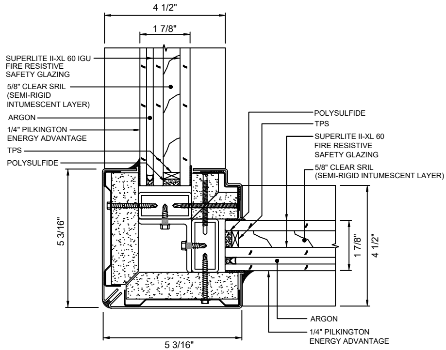
A 90° CORNER DETAIL 10 WITH SUPERLITE II-XL 60 IGU
