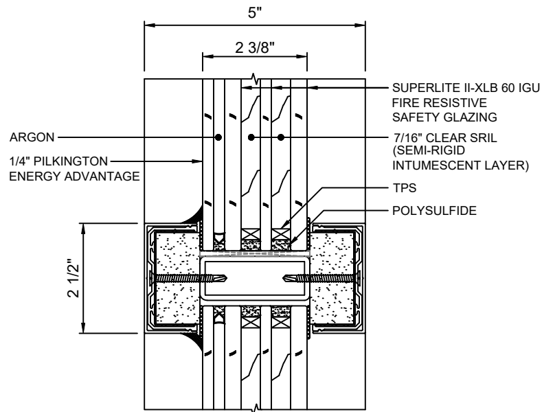
B 6 HORIZONTAL MULLION WITH SUPERLITE II-XLB 60 IGU
