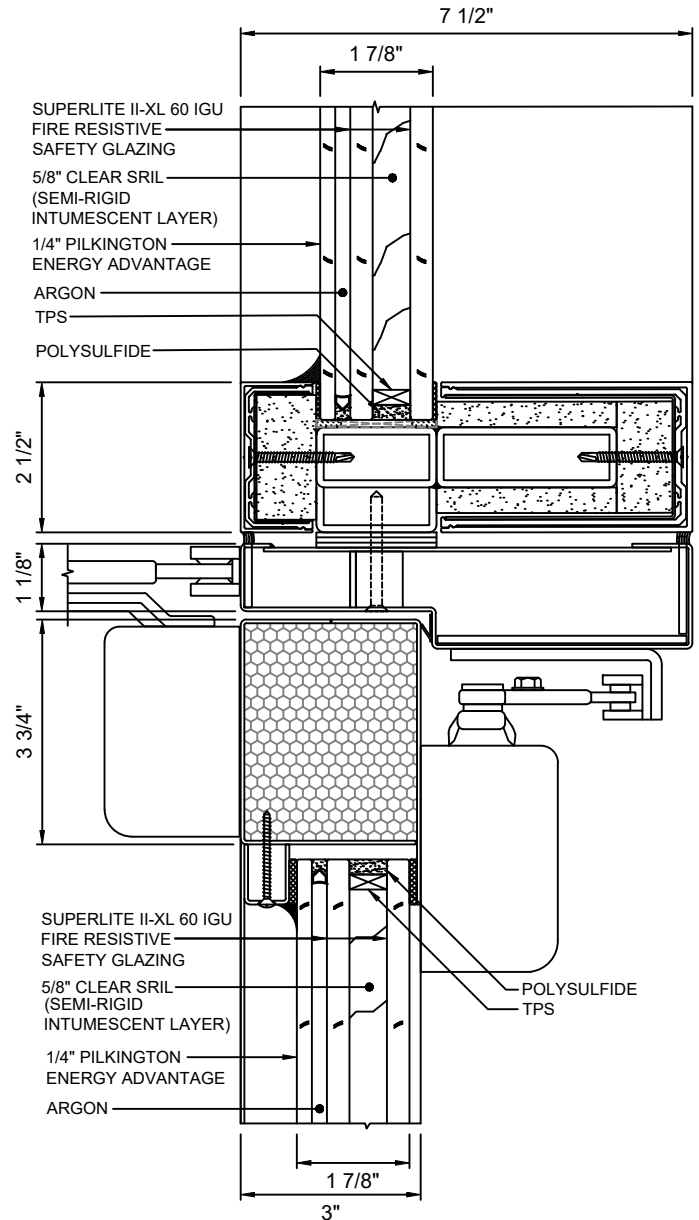
E DOOR TOP RAIL - NARROW STYLE 9 WITH SUPERLITE II-XL 60 IGU
