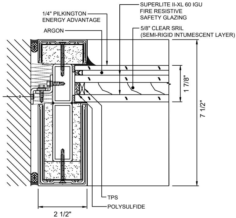
A JAMB DETAIL 6 WITH SUPERLITE II-XL 60 IGU
