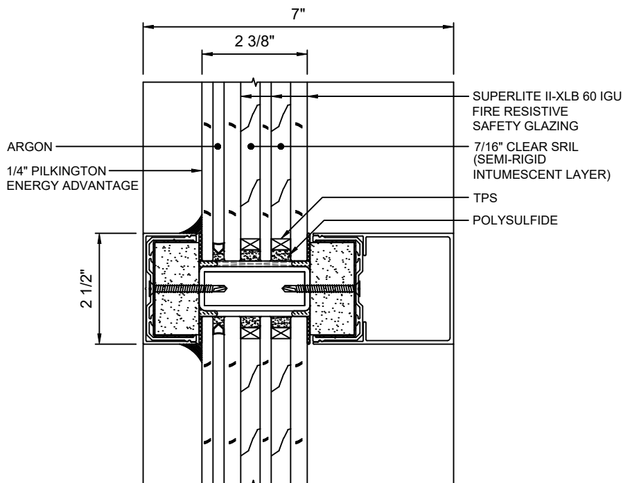
B 4 HORIZONTAL MULLION WITH SUPERLITE II-XLB 60 IGU
