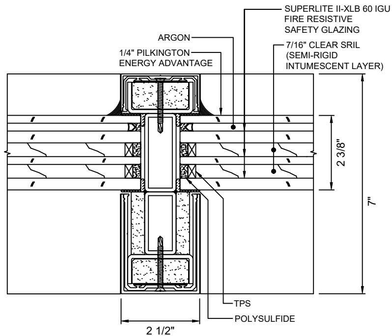
B 7 VERTICAL MULLION DETAIL WITH SUPERLITE II-XLB 60 IGU
