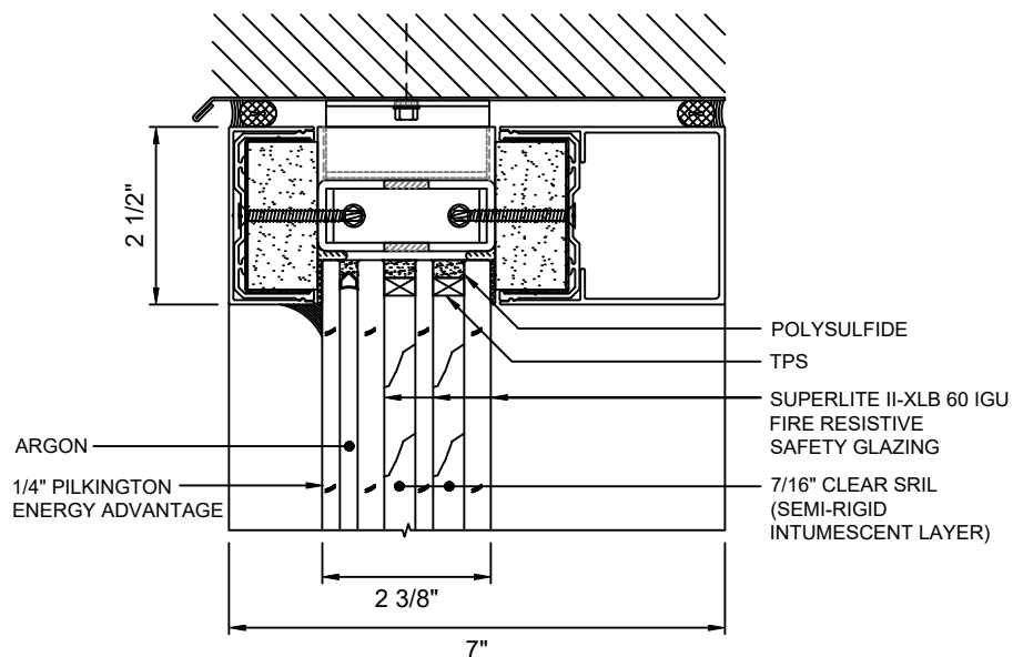
B 3 HEAD DETAIL WITH SUPERLITE II-XLB 60 IGU
