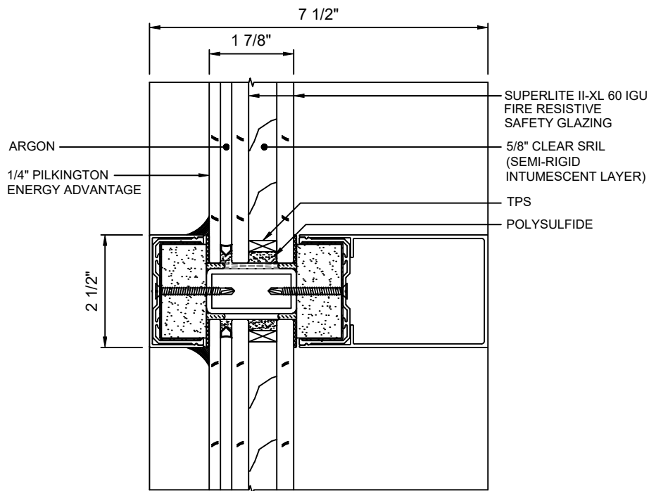
A 4 HORIZONTAL MULLION WITH SUPERLITE II-XL 60 IGU
