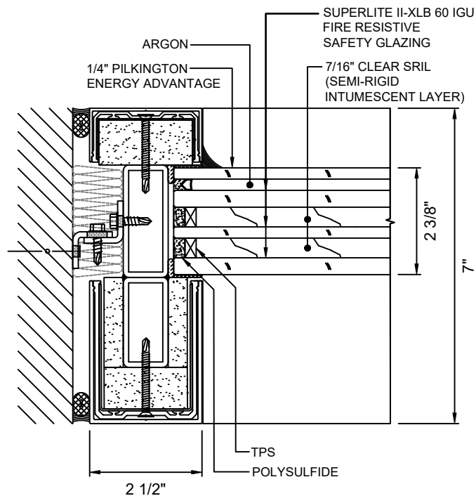
B JAMB DETAIL 6 WITH SUPERLITE II-XLB 60 IGU
