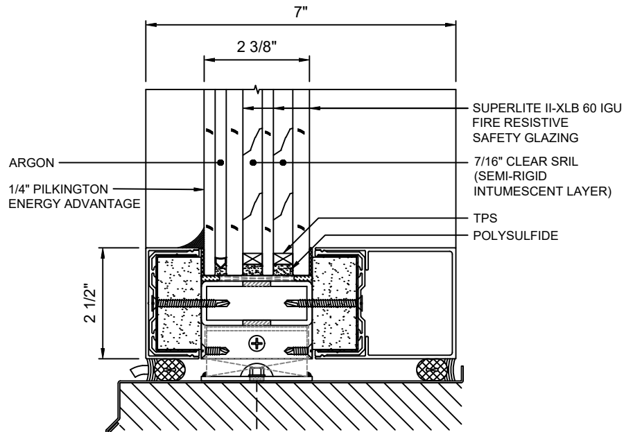
B SILL DETAIL 5 WITH SUPERLITE II-XLB 60 IGU
