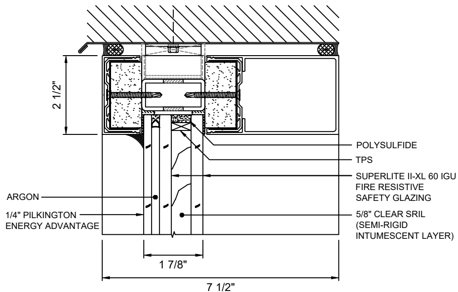
A 3 HEAD DETAIL WITH SUPERLITE II-XL 60 IGU
