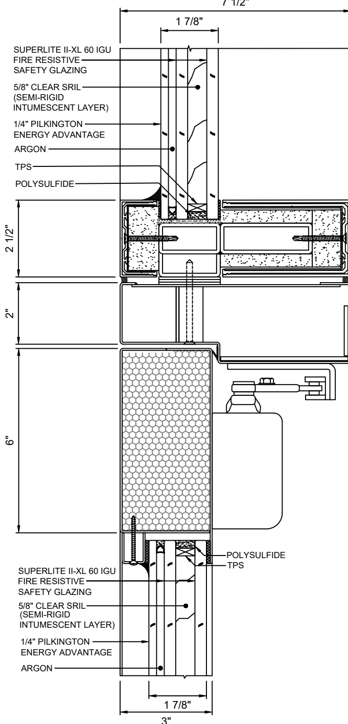
D DOOR TOP RAIL - STANDARD 9 WITH SUPERLITE II-XL 60 IGU
