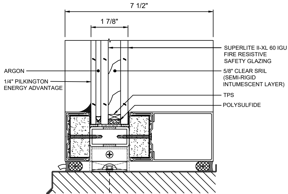
A SILL DETAIL 5 WITH SUPERLITE II-XL 60 IGU
