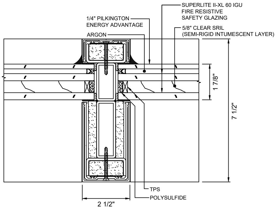
A 7 VERTICAL MULLION DETAIL WITH SUPERLITE II-XL 60 IGU
