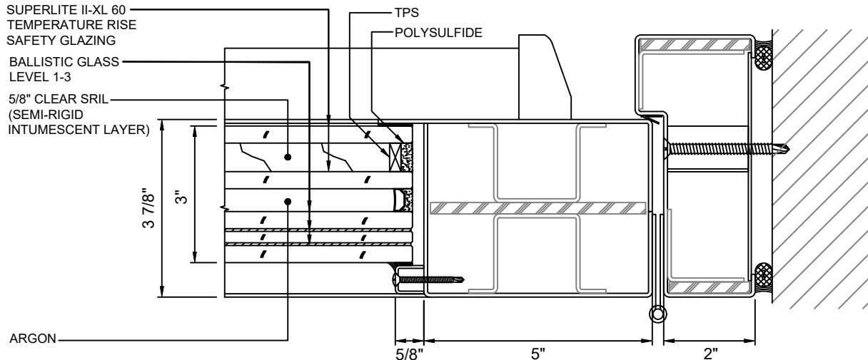
(A) 5 DOOR JAMB AT HINGE - STANDARD WITH SUPERLITE II-XL 60 WITH LEVEL 1-3 BALLISTIC GLASS
