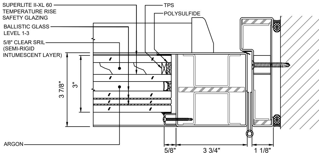
(B) 5 DOOR JAMB AT HINGE - NARROW STYLE WITH SUPERLITE II-XL 60 WITH LEVEL 1-3 BALLISTIC GLASS
