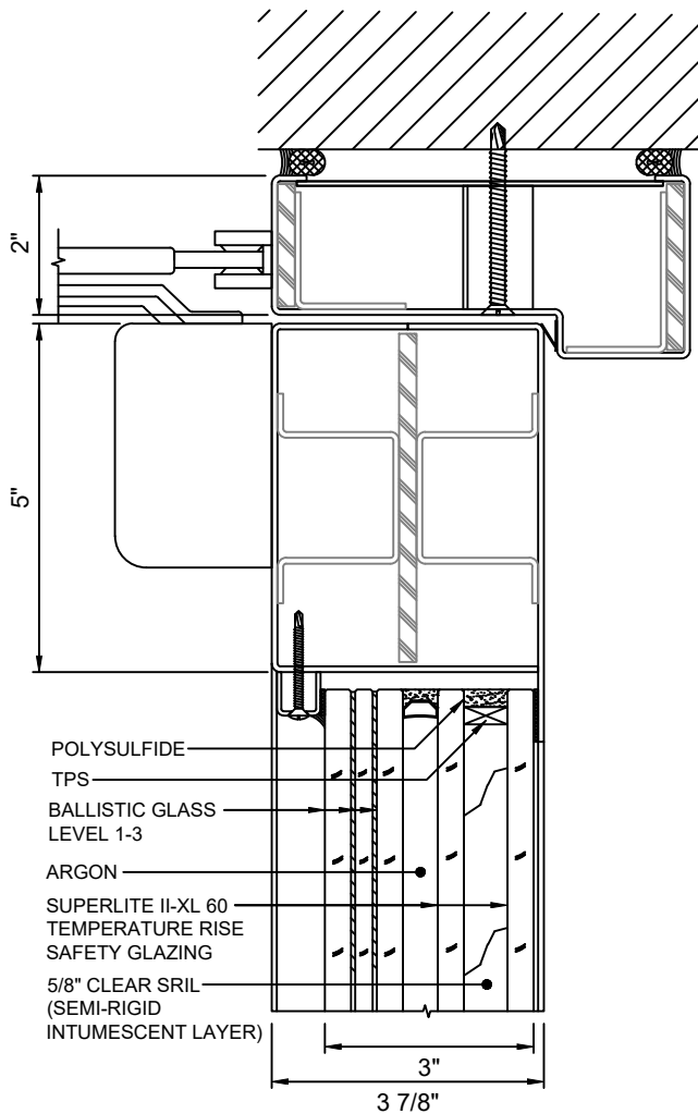
A 2 DOOR TOP RAIL - STANDARD WITH SUPERLITE II-XL 60 WITH LEVEL 1-3 BALLISTIC GLASS
