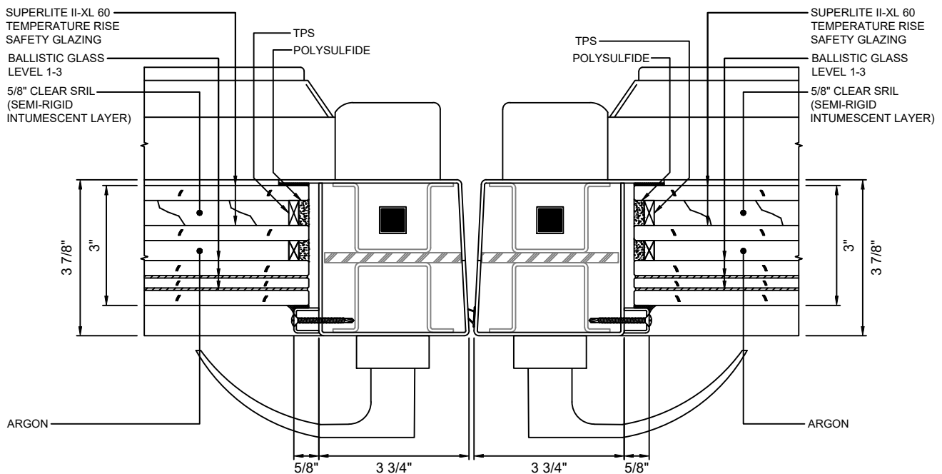
B MEETING STILES - NARROW STYLE 6 WITH SUPERLITE II-XL 60 WITH LEVEL 1-3 BALLISTIC GLASS
