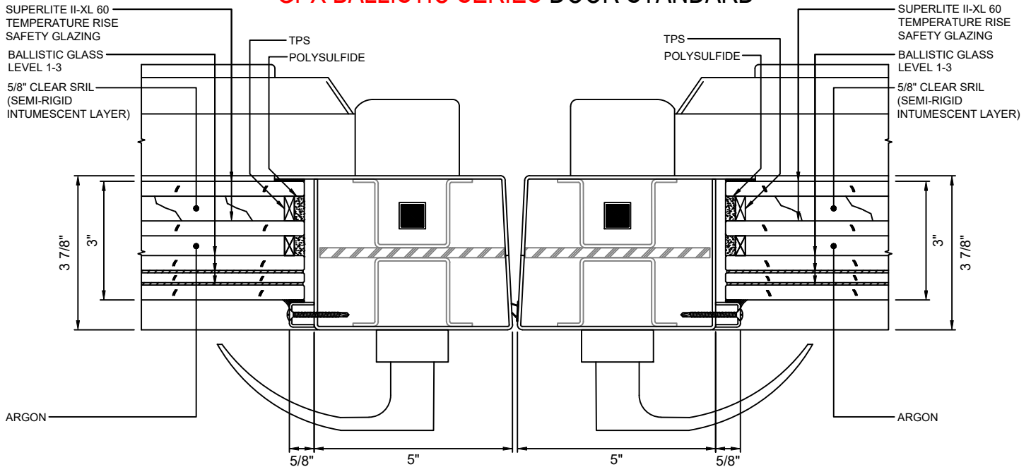
A MEETING STILES - STANDARD 6 WITH SUPERLITE II-XL 60 WITH LEVEL 1-3 BALLISTIC GLASS
