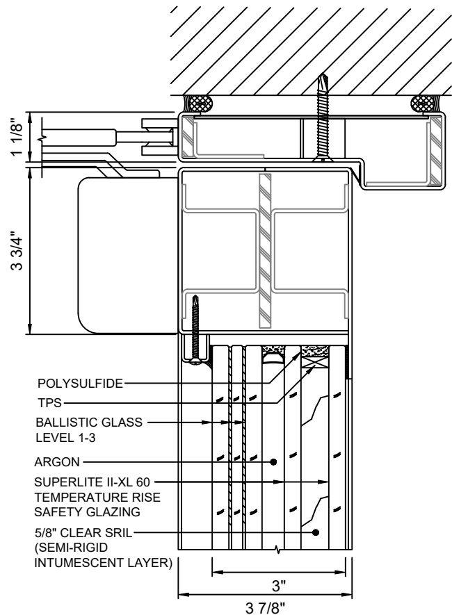
B 2 DOOR TOP RAIL - NARROW STYLE WITH SUPERLITE II-XL 60 WITH LEVEL 1-3 BALLISTIC GLASS
