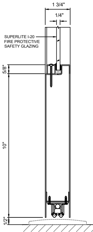
D 11 DOOR BOTTOM RAIL - STANDARD WITH DOOR BOTTOM WITH SUPERLITE I-20
