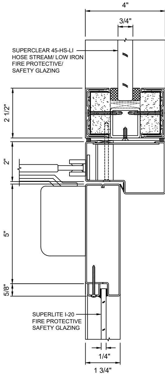
D DOOR TOP RAIL - STANDARD 10 WITH SUPERCLEAR 45-HS-LI & SUPERLITE I-20
