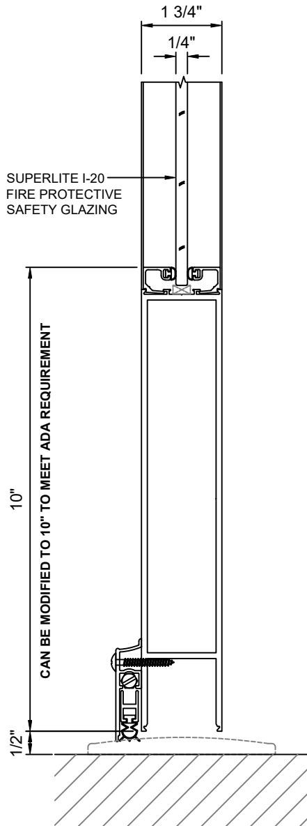
16 DOOR BOTTOM RAIL WITHOUT DOOR BOTTOM WITH SUPERLITE I-20
