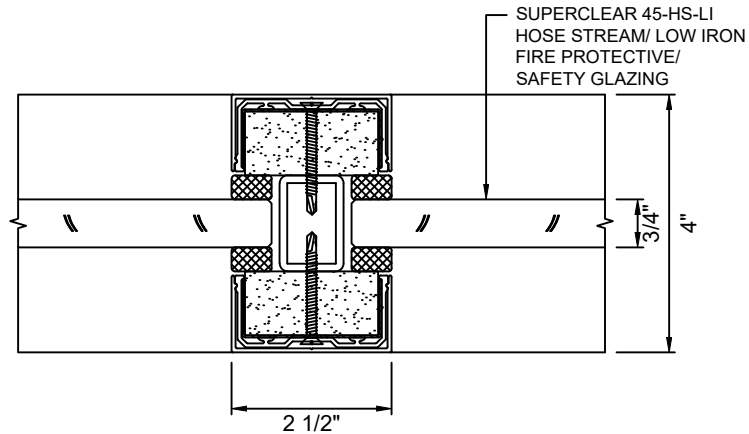
A 9 VERTICAL MULLION WITH SUPERCLEAR 45-HS-LI
