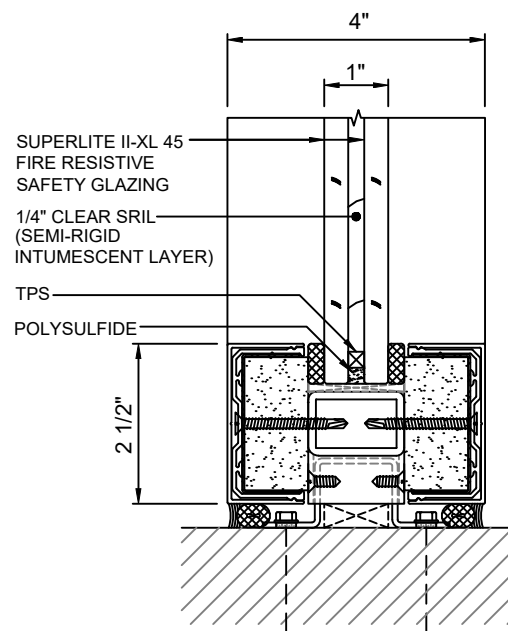
B 7 SILL DETAIL WITH SUPERLITE II-XL 45
