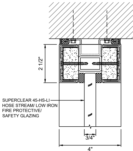
A 5 HEAD DETAIL WITH SUPERCLEAR 45-HS-LI
