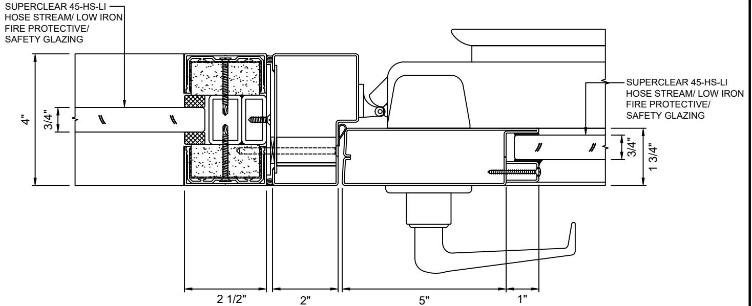
D DOOR JAMB AT LOCK - STANDARD 22 WITH SUPERCLEAR 45-HS-LI
