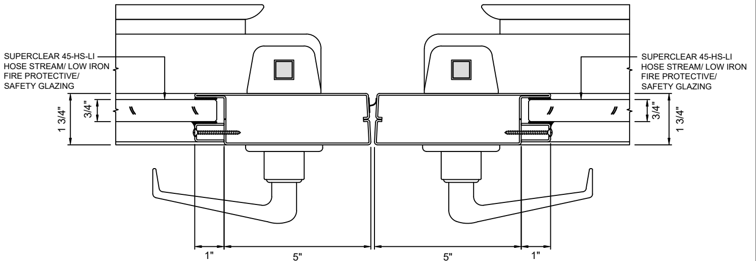
D MEETING STILES - STANDARD 24 WITH SUPERCLEAR 45-HS-LI
