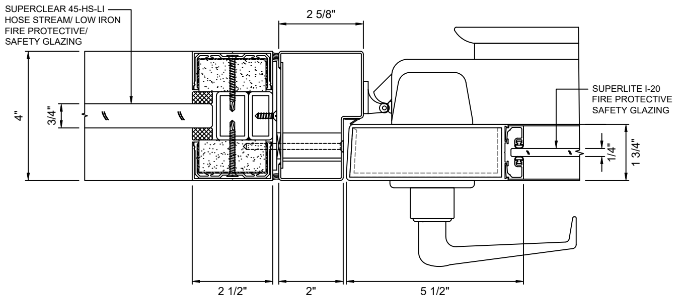
17 DOOR JAMB AT LOCK WITH SUPERCLEAR 45-HS-LI & SUPERLITE I-20
