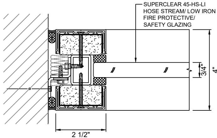
A 8 JAMB DETAIL WITH SUPERCLEAR 45-HS-LI
