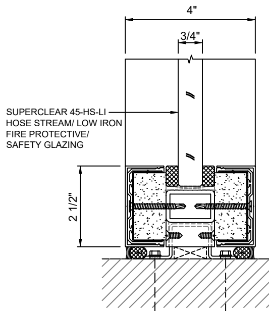
A 7 SILL DETAIL WITH SUPERCLEAR 45-HS-LI
