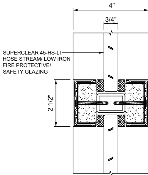
A 6 HORIZONTAL MULLION WITH SUPERCLEAR 45-HS-LI
