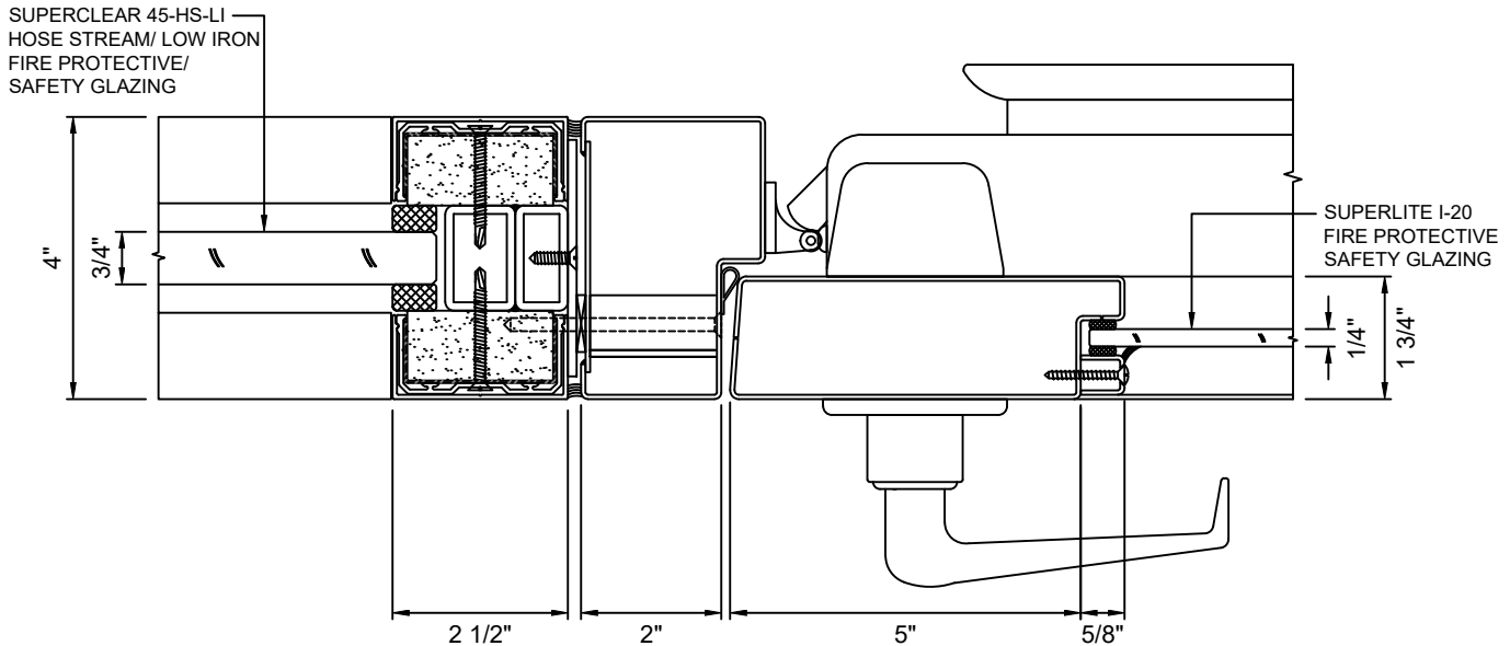
D DOOR JAMB AT LOCK - STANDARD WITH SUPERCLEAR 45-HS-LI & SUPERLITE I-20
