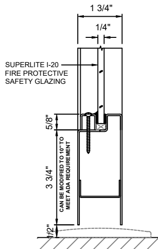
E 11 DOOR BOTTOM RAIL - NARROW STYLE WITHOUT DOOR BOTTOM WITH SUPERLITE I-20
