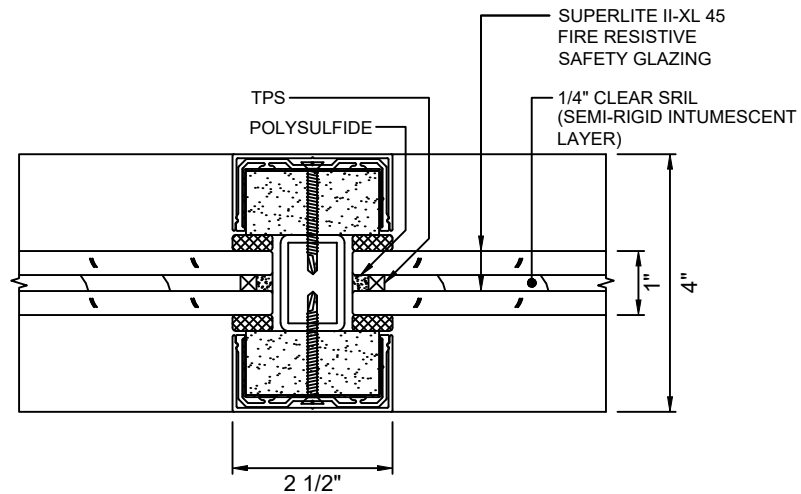
B 9 VERTICAL MULLION WITH SUPERLITE II-XL 45
