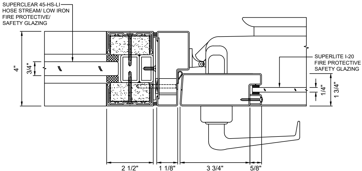
E DOOR JAMB AT LOCK - NARROW STYLE WITH SUPERCLEAR 45-HS-LI & SUPERLITE I-20
