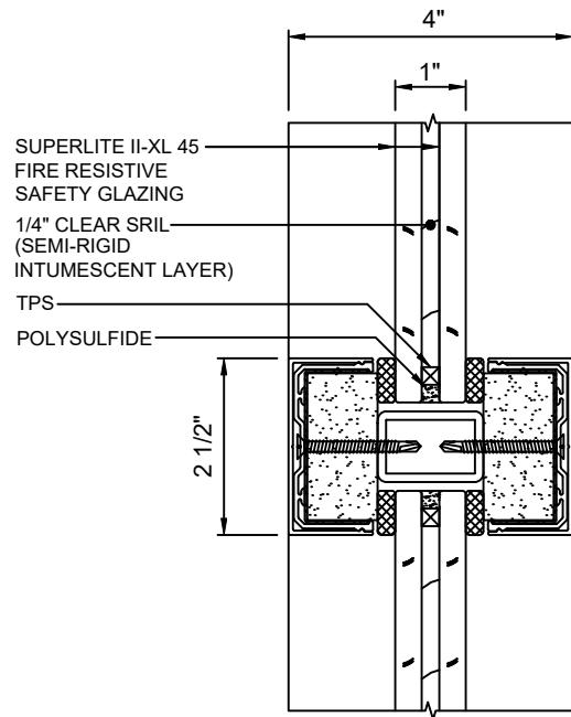
B 6 HORIZONTAL MULLION WITH SUPERLITE II-XL 45
