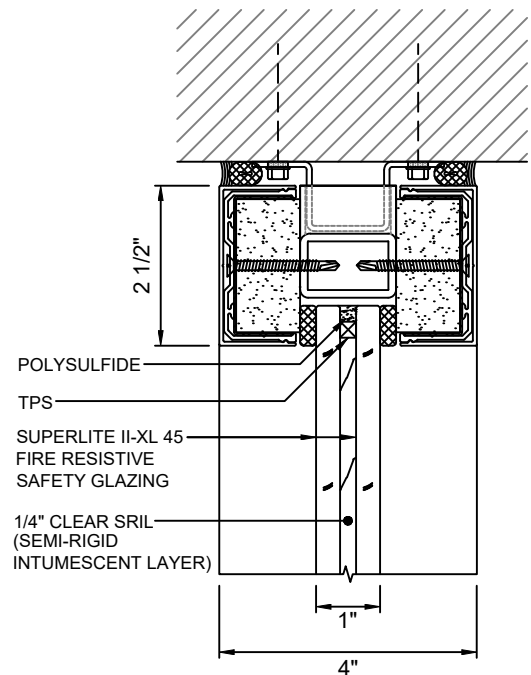
B 5 HEAD DETAIL WITH SUPERLITE II-XL 45
