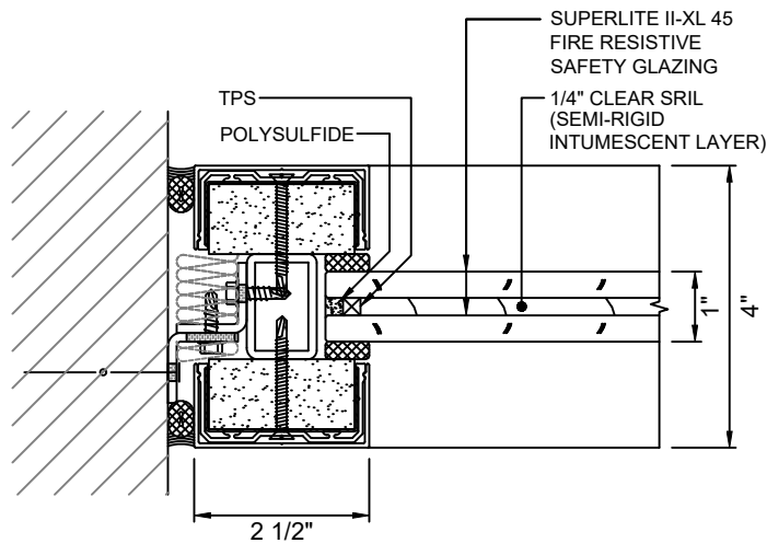
B 8 JAMB DETAIL WITH SUPERLITE II-XL 45
