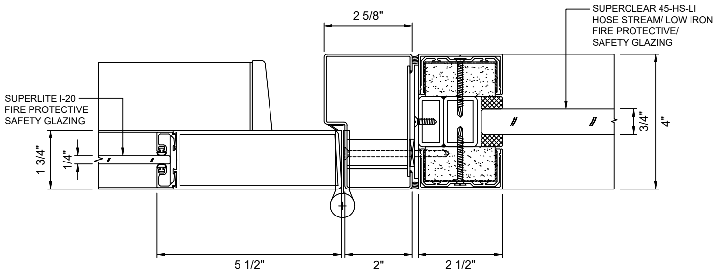
18 DOOR JAMB AT HINGE WITH SUPERCLEAR 45-HS-LI & SUPERLITE I-20
