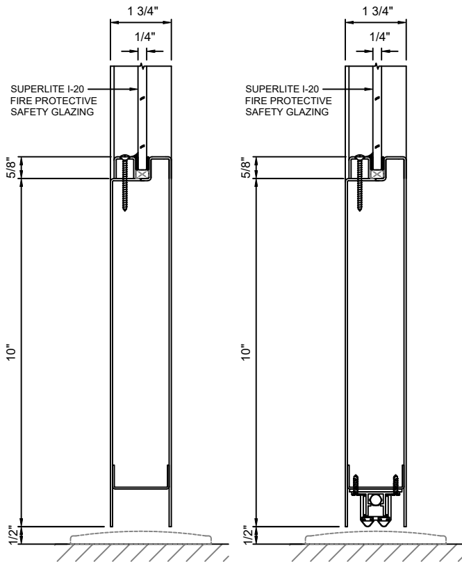
D 11 DOOR BOTTOM RAIL - STANDARD WITHOUT DOOR BOTTOM WITH SUPERLITE I-20
