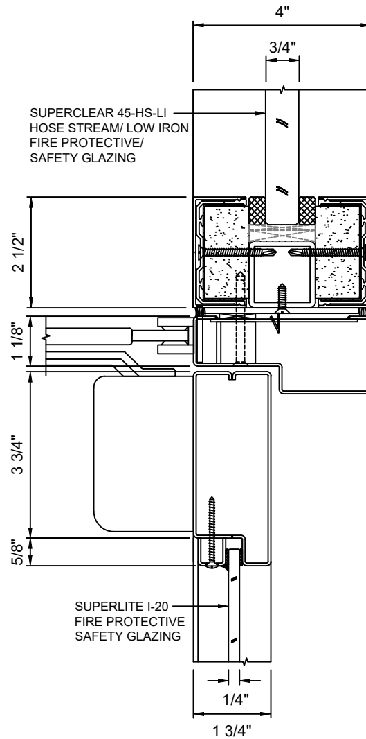
E DOOR TOP RAIL - NARROW STYLE 10 WITH SUPERCLEAR 45-HS-LI & SUPERLITE I-20
