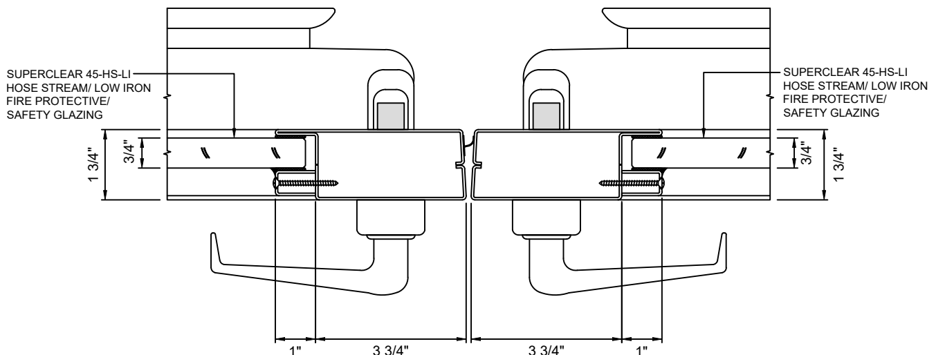
E MEETING STILES - NARROW STYLE 24 WITH SUPERCLEAR 45-HS-LI
