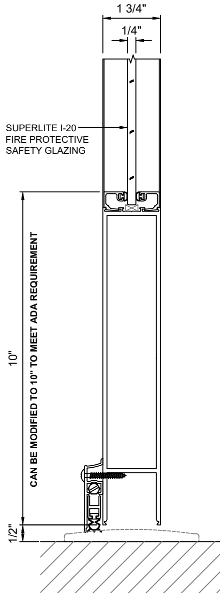
16 DOOR BOTTOM RAIL WITH DOOR BOTTOM WITH SUPERLITE I-20
