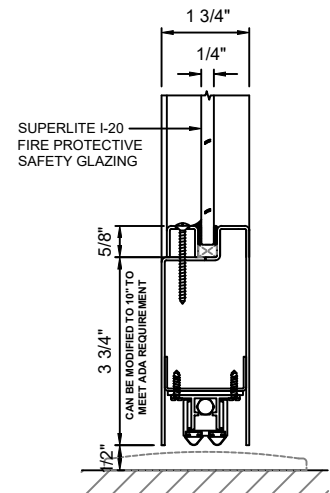
E 11 DOOR BOTTOM RAIL - NARROW STYLE WITH DOOR BOTTOM WITH SUPERLITE I-20
