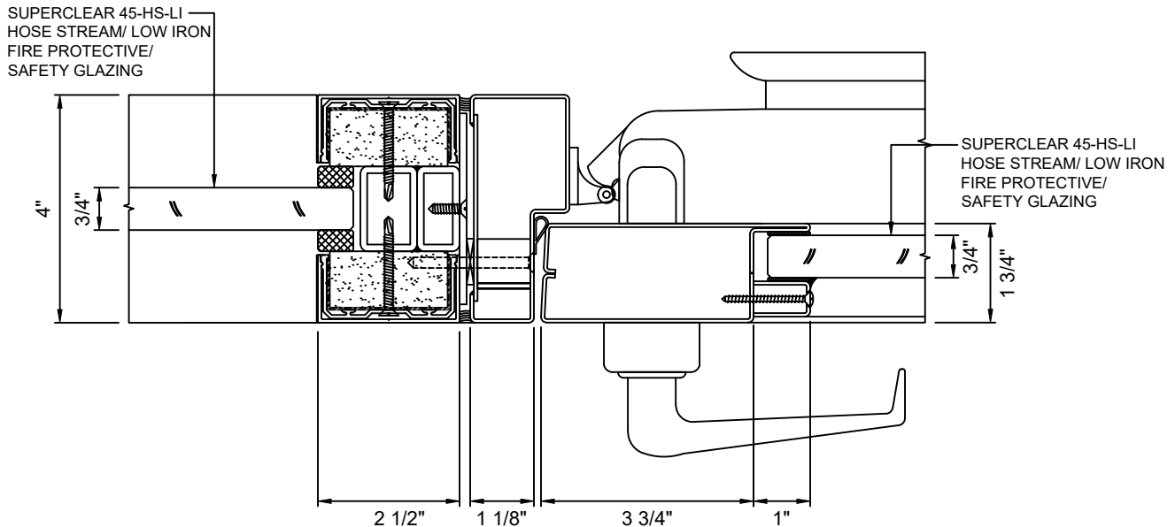
E DOOR JAMB AT LOCK - NARROW STYLE 22 WITH SUPERCLEAR 45-HS-LI
