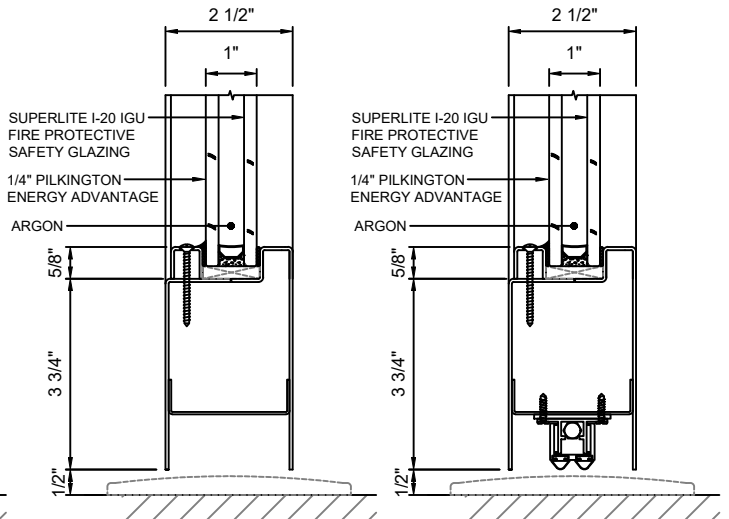
E 11 DOOR BOTTOM RAIL - NARROW WITHOUT DOOR BOTTOM WITH SUPERLITE I-20 IGU
