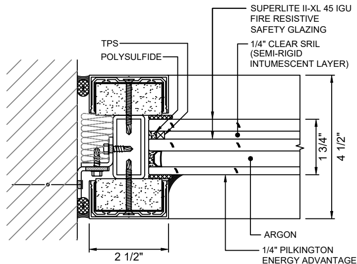
B JAMB DETAIL 8 WITH SUPERLITE II-XL 45 IGU
