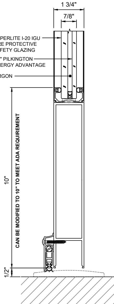
16 DOOR BOTTOM RAIL WITH DOOR BOTTOM WITH SUPERLITE I-20 IGU
