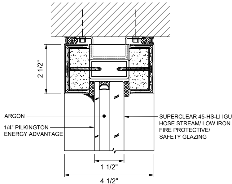
A 5 HEAD DETAIL WITH SUPERCLEAR 45-HS-LI IGU
