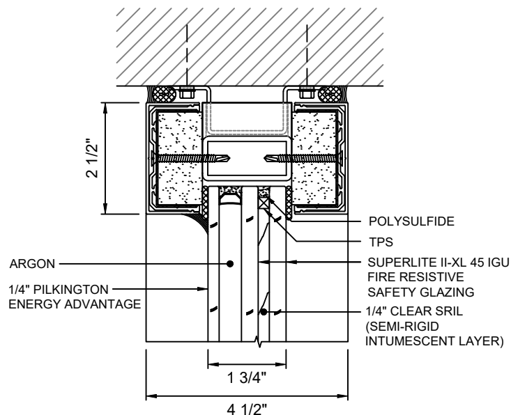
B 5 HEAD DETAIL WITH SUPERLITE II-XL 45 IGU
