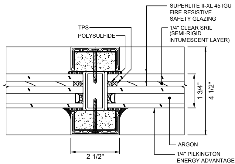
B 9 VERTICAL MULLION WITH SUPERLITE II-XL 45 IGU
