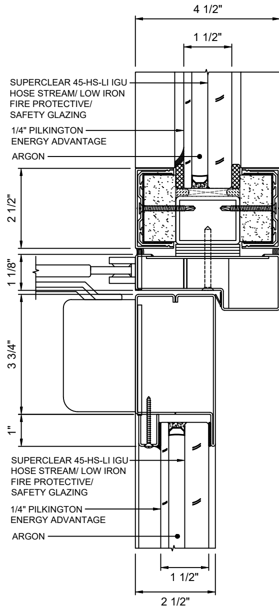
E DOOR TOP RAIL - NARROW STYLE 20 WITH SUPERCLEAR 45-HS-LI IGU
