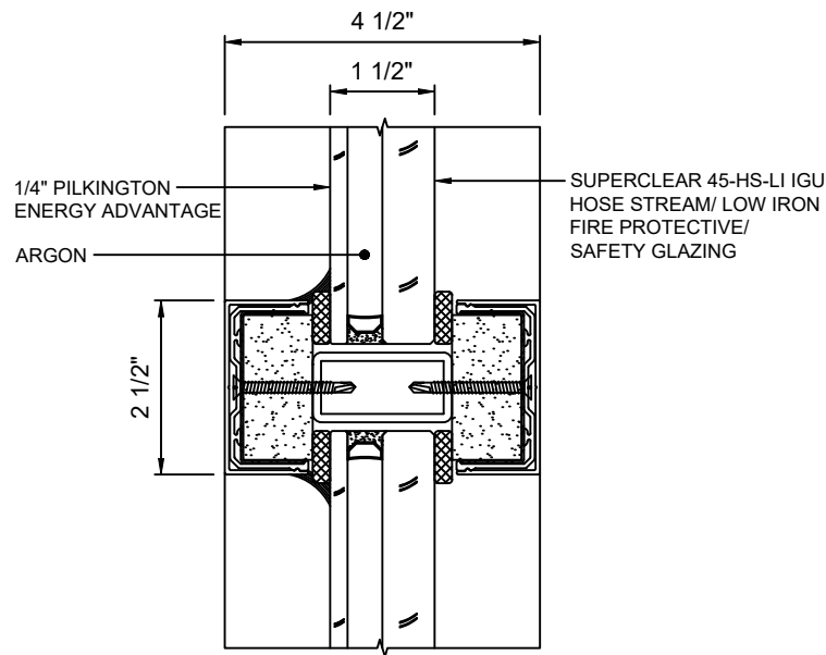
A 6 HORIZONTAL MULLION WITH SUPERCLEAR 45-HS-LI IGU
