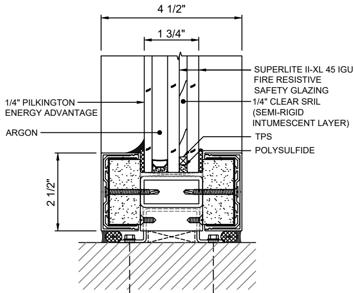
B 7 SILL DETAIL WITH SUPERLITE II-XL 45 IGU
