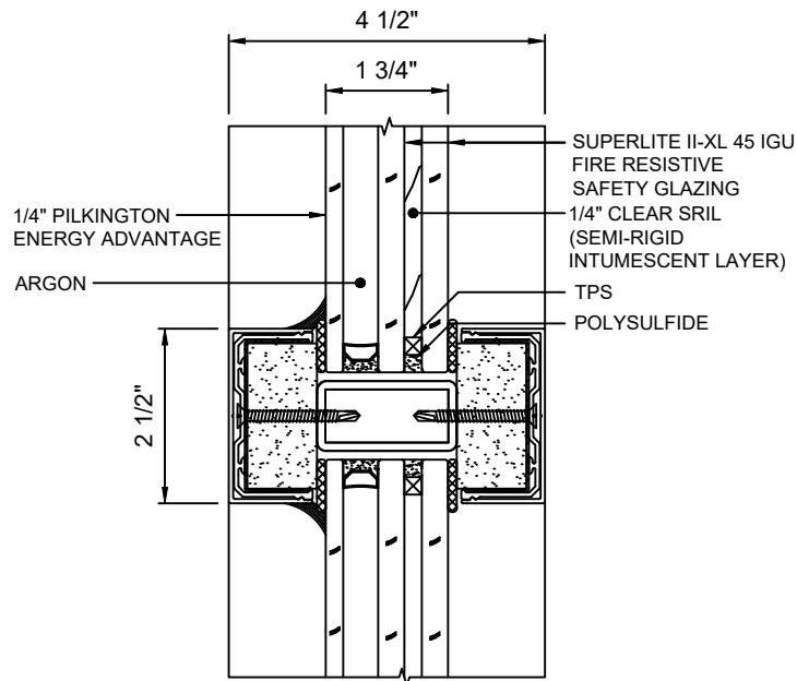
B 6 HORIZONTAL MULLION WITH SUPERLITE II-XL 45 IGU
