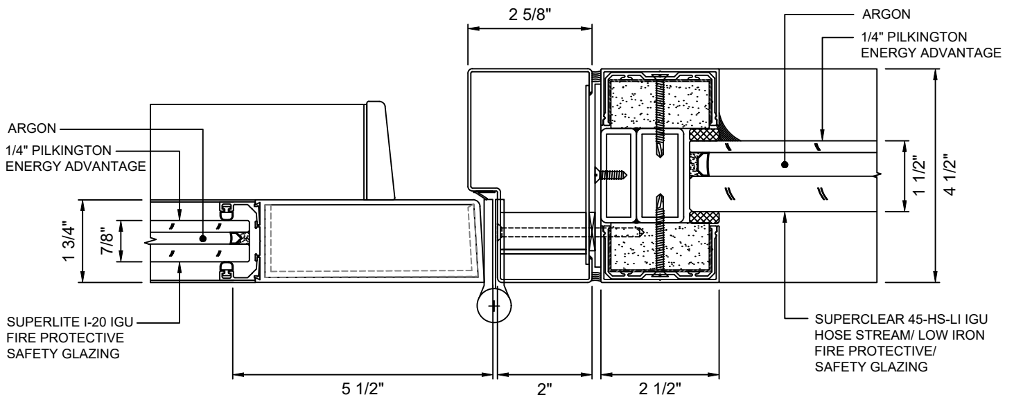
18 DOOR JAMB AT HINGE WITH SUPERCLEAR 45-HS-LI IGU & SUPERLITE I-20 IGU
