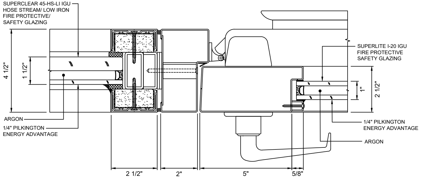
D DOOR JAMB AT LOCK - STANDARD WITH SUPERCLEAR 45-HS-LI IGU & SUPERLITE I-20 IGU
