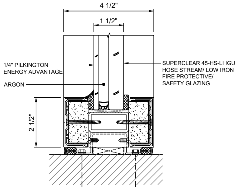
A 7 SILL DETAIL WITH SUPERCLEAR 45-HS-LI IGU
