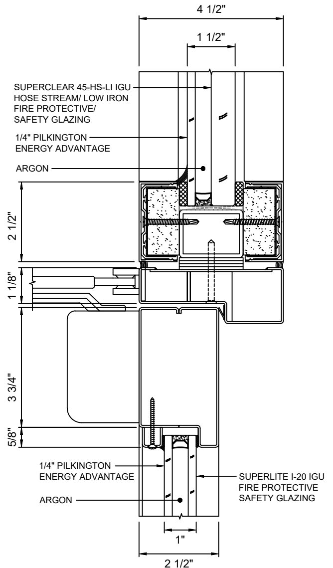
E DOOR TOP RAIL - NARROW STYLE 10 WITH SUPERCLEAR 45-HS-LI IGU & SUPERLITE I-20 IGU
