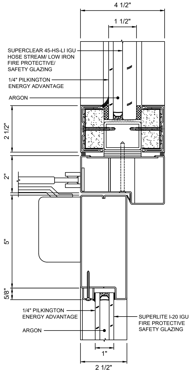
D DOOR TOP RAIL - STANDARD 10 WITH SUPERCLEAR 45-HS-LI IGU & SUPERLITE I-20 IGU
