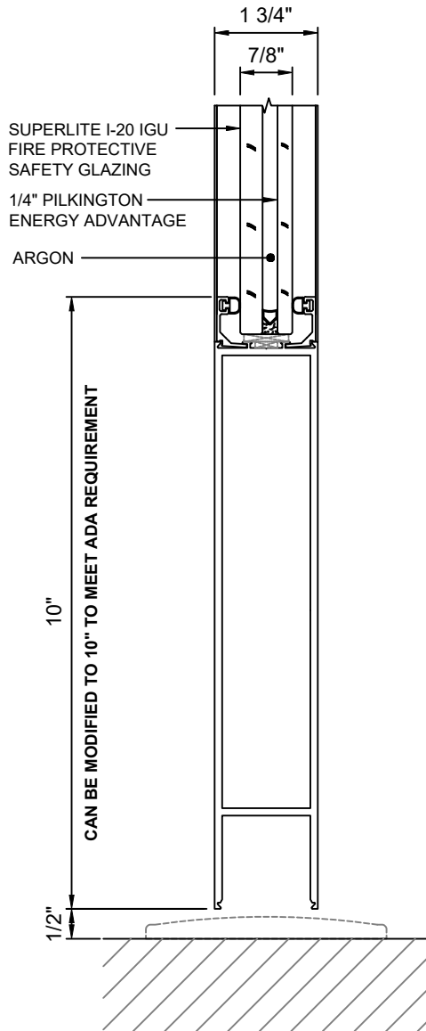
16 DOOR BOTTOM RAIL WITHOUT DOOR BOTTOM WITH SUPERLITE I-20 IGU
