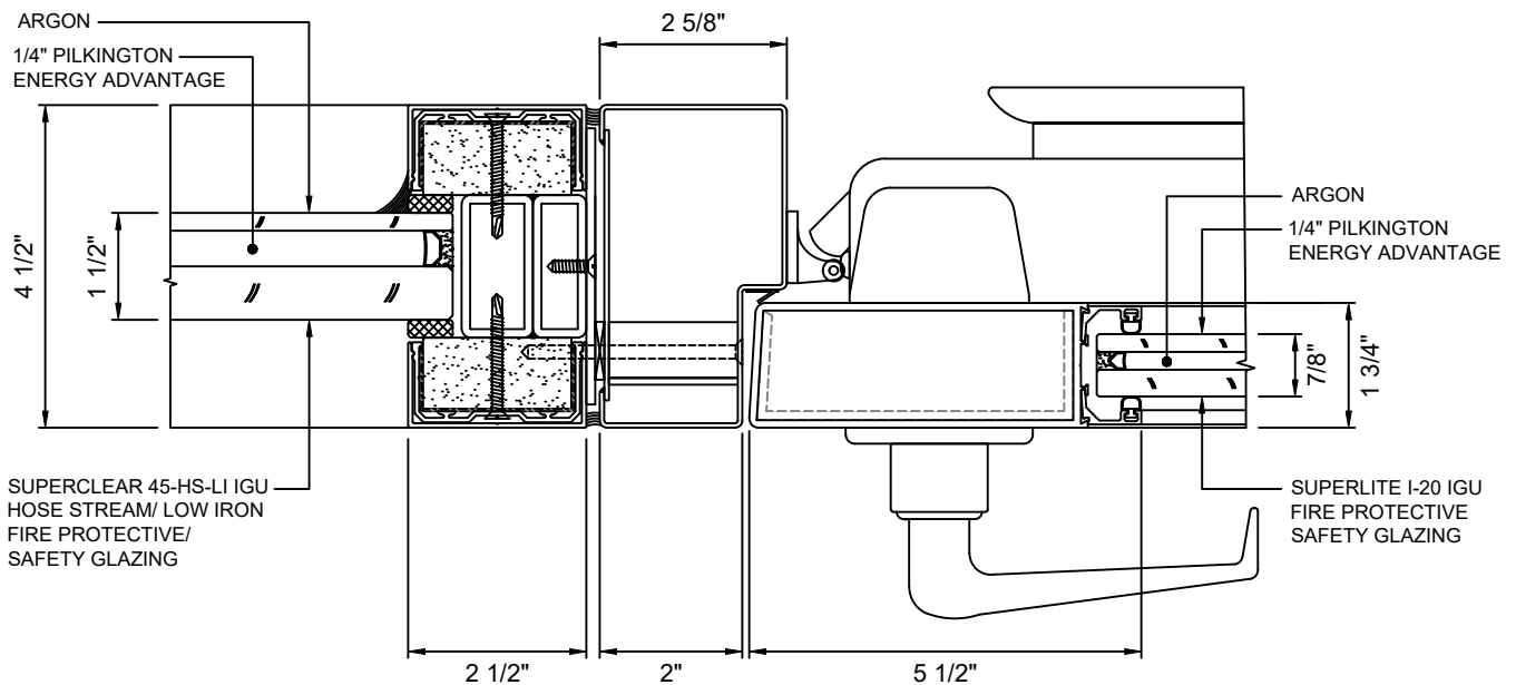
17 DOOR JAMB AT LOCK WITH SUPERCLEAR 45-HS-LI IGU & SUPERLITE I-20 IGU
