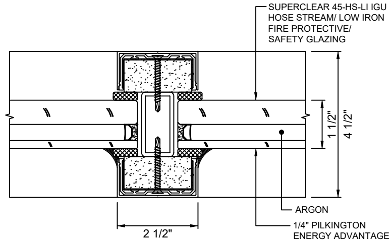
A 9 VERTICAL MULLION WITH SUPERCLEAR 45-HS-LI IGU
