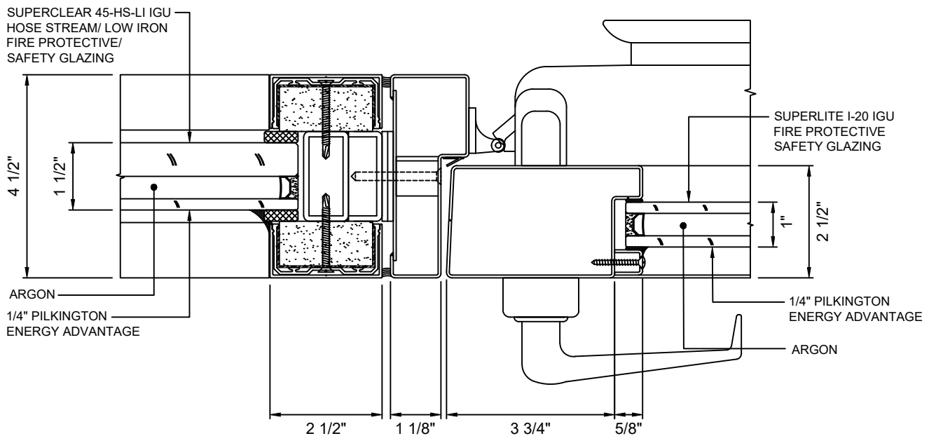
E DOOR JAMB AT LOCK - NARROW STYLE WITH SUPERCLEAR 45-HS-LI IGU & SUPERLITE I-20 IGU
