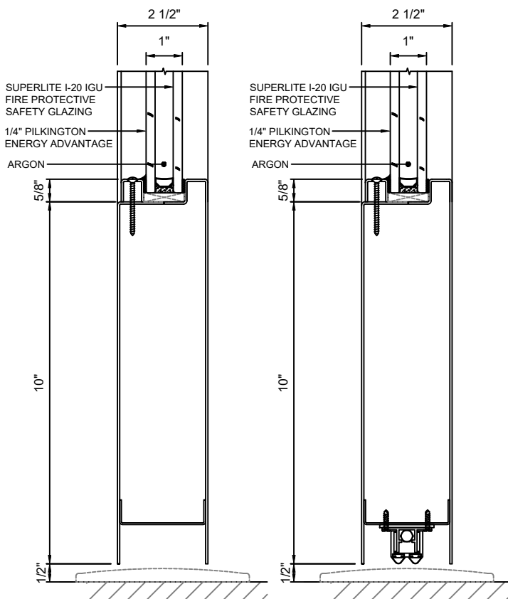
D 11 DOOR BOTTOM RAIL - STANDARD WITHOUT DOOR BOTTOM WITH SUPERLITE I-20 IGU
