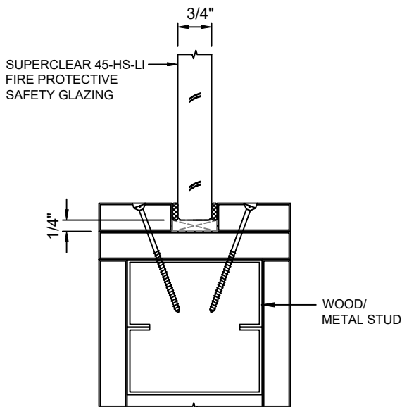
A 2.1 SILL DETAIL ON WOOD OR METAL STUD WITH SUPERCLEAR 45-HS-LI
