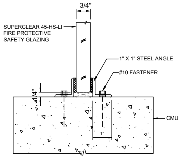
A 2.3 SILL DETAIL WITH STEEL ANGLES WITH SUPERCLEAR 45-HS-LI
