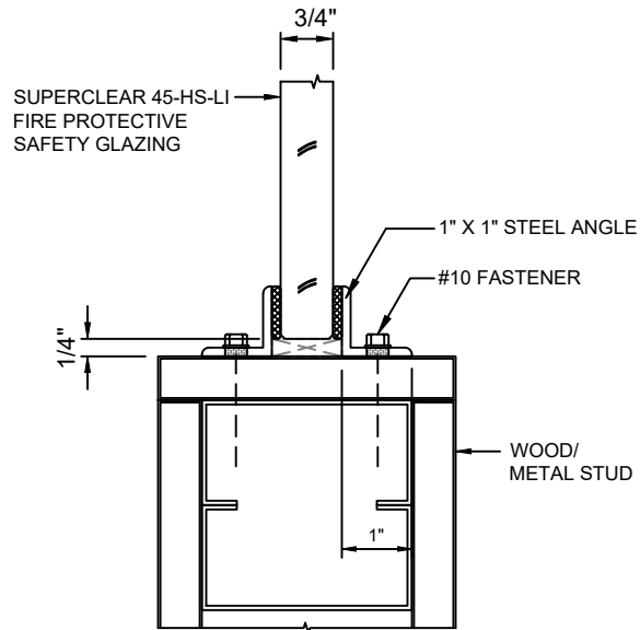
A 2.2 SILL DETAIL WITH STEEL ANGLES ON WOOD OR METAL STUD WITH SUPERCLEAR 45-HS-LI
