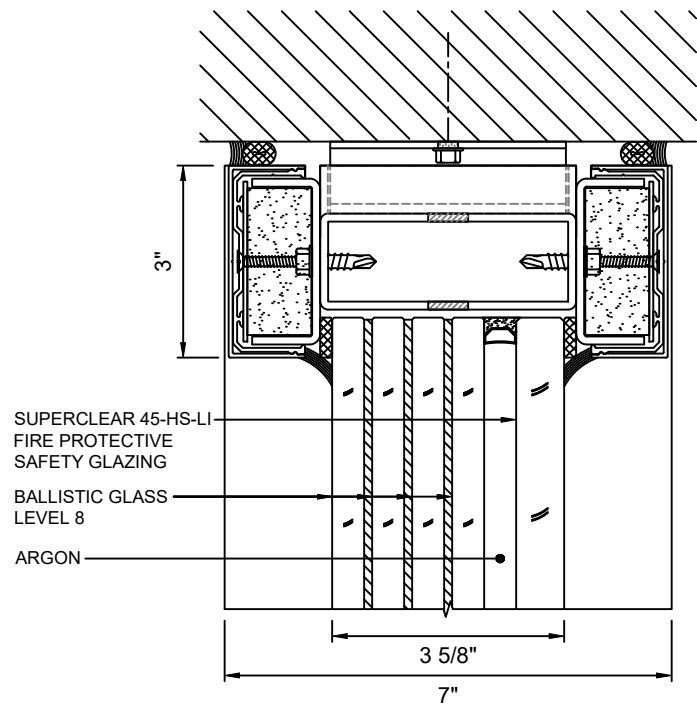
E 5 HEAD DETAIL WITH SUPERCLEAR 45-HS-LI WITH LEVEL 8 BALLISTIC GLASS
