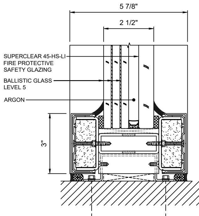
C 6 SILL DETAIL WITH SUPERCLEAR 45-HS-LI WITH LEVEL 5 BALLISTIC GLASS
