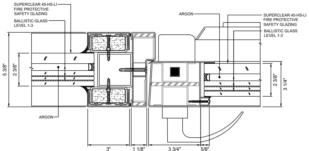
G 21 DOOR JAMB AT LOCK - NARROW STYLE WITH SUPERCLEAR 45-HS-LI WITH LEVEL 1-3 BALLISTIC GLASS
