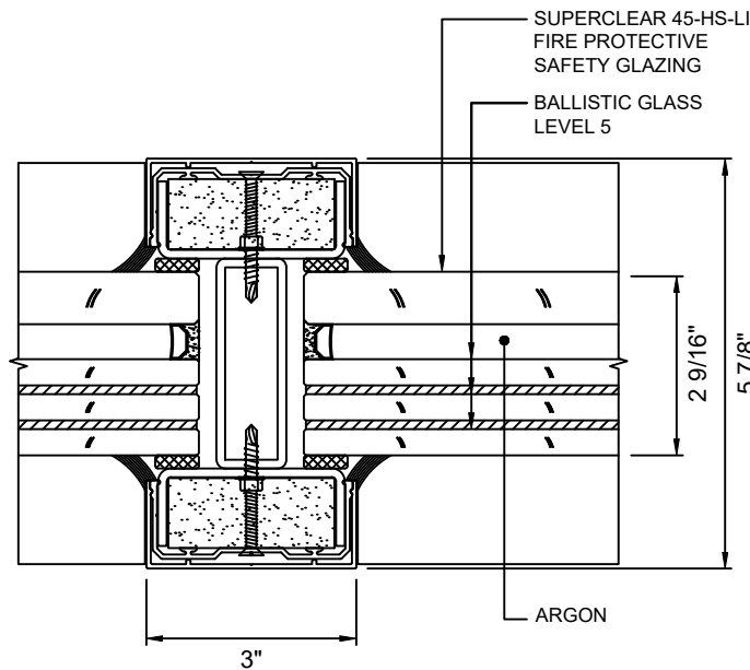
C 12 VERTICAL MULLION DETAIL WITH SUPERCLEAR 45-HS-LI WITH LEVEL 5 BALLISTIC GLASS
