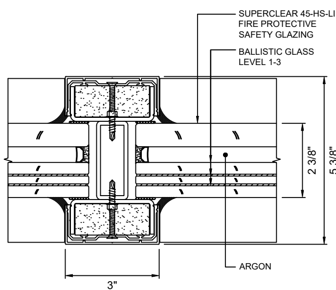
A 12 VERTICAL MULLION DETAIL WITH SUPERCLEAR 45-HS-LI WITH LEVEL 1-3 BALLISTIC GLASS
