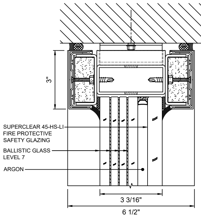
D 5 HEAD DETAIL WITH SUPERCLEAR 45-HS-LI WITH LEVEL 7 BALLISTIC GLASS
