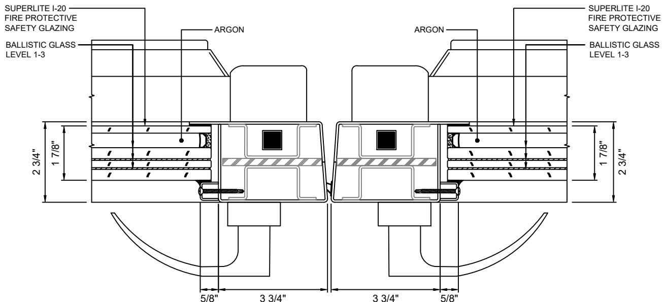
G 18 MEETING STILES - NARROW STYLE WITH SUPERLITE I-20 WITH LEVEL 1-3 BALLISTIC GLASS
