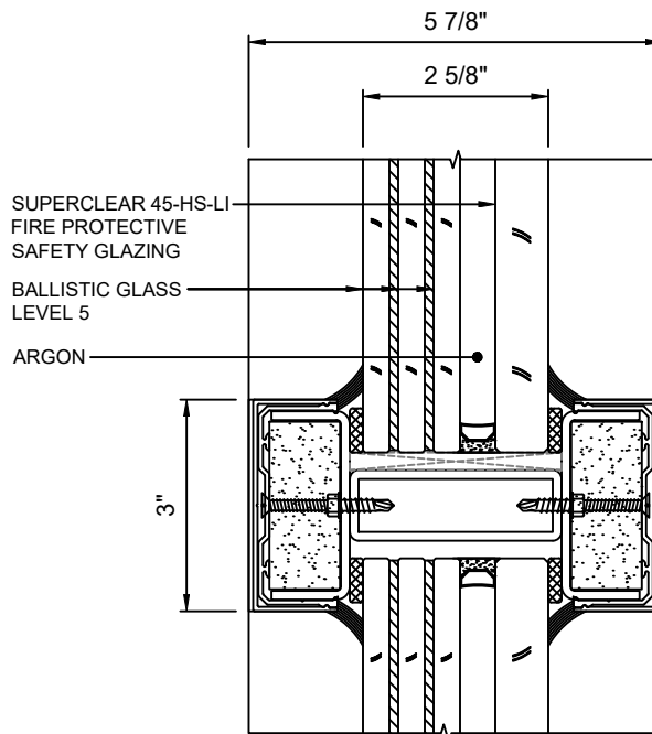
C 8 HORIZONTAL MULLION DETAIL WITH SUPERCLEAR 45-HS-LI WITH LEVEL 5 BALLISTIC GLASS
