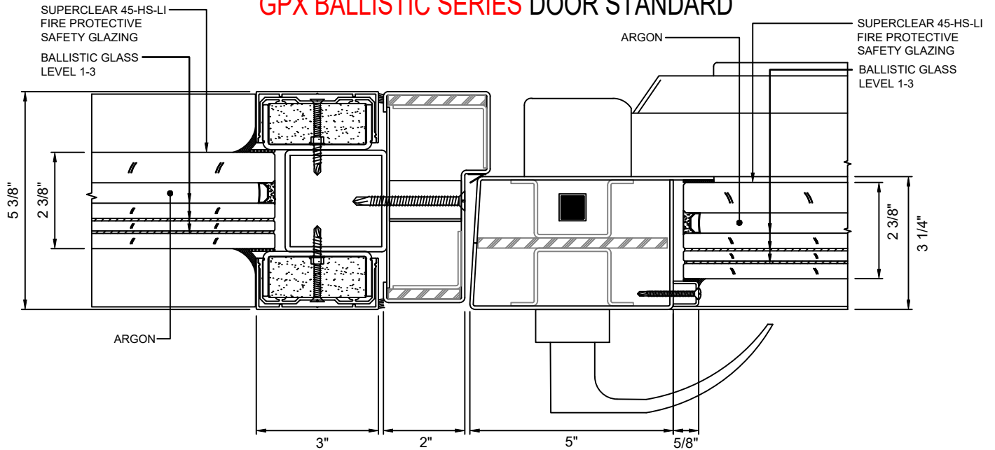
F 21 DOOR JAMB AT LOCK - STANDARD WITH SUPERCLEAR 45-HS-LI WITH LEVEL 1-3 BALLISTIC GLASS
