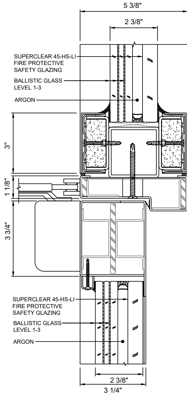
G 19 DOOR TOP RAIL - NARROW STYLE WITH SUPERCLEAR 45-HS-LI WITH LEVEL 1-3 BALLISTIC GLASS
