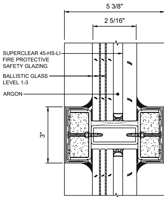
A 8 HORIZONTAL MULLION DETAIL WITH SUPERCLEAR 45-HS-LI WITH LEVEL 1-3 BALLISTIC GLASS
