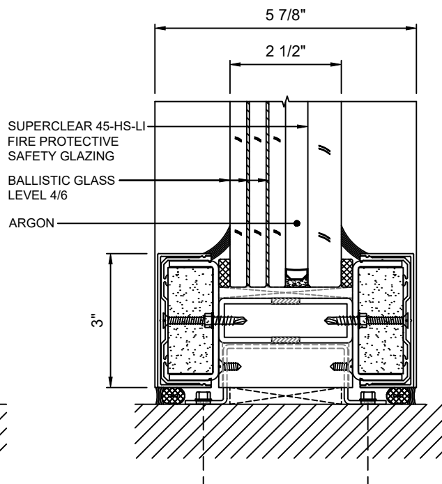
B 6 SILL DETAIL WITH SUPERCLEAR 45-HS-LI WITH LEVEL 4/6 BALLISTIC GLASS
