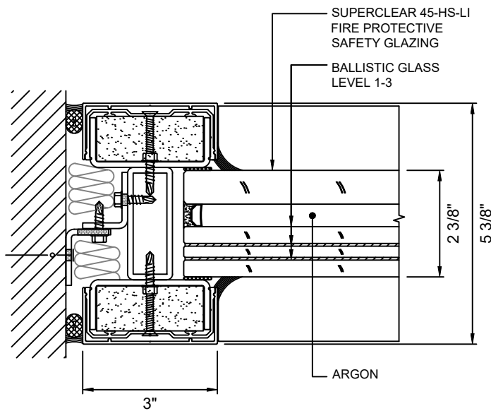
A 10 JAMB DETAIL WITH SUPERCLEAR 45-HS-LI WITH LEVEL 1-3 BALLISTIC GLASS
