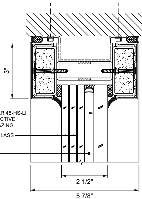
B 4 HEAD DETAIL WITH SUPERCLEAR 45-HS-LI WITH LEVEL 4/6 BALLISTIC GLASS
