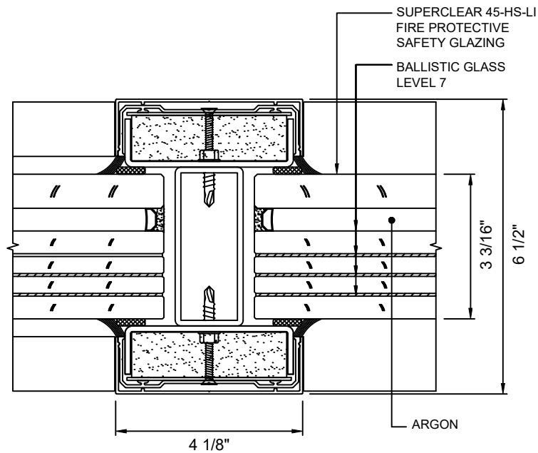
D 13 VERTICAL MULLION DETAIL WITH SUPERCLEAR 45-HS-LI WITH LEVEL 7 BALLISTIC GLASS
