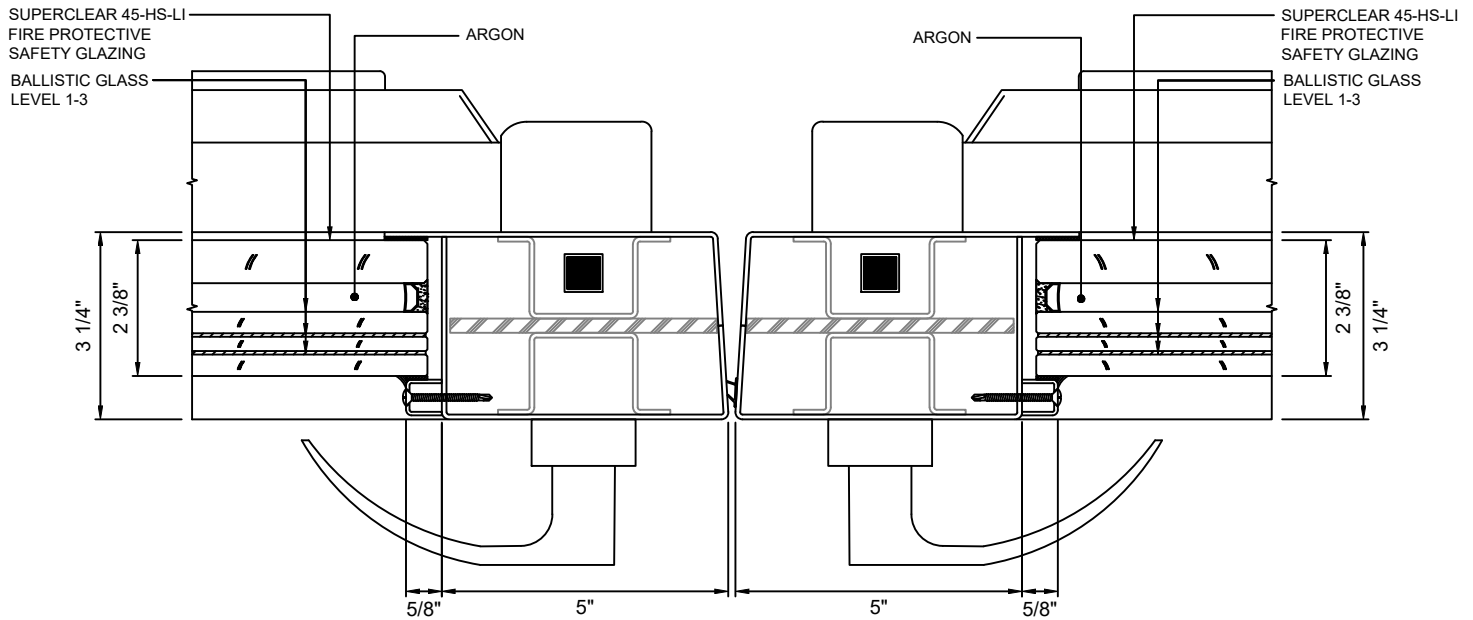
F 23 MEETING STILES - STANDARD WITH SUPERCLEAR 45-HS-LI WITH LEVEL 1-3 BALLISTIC GLASS
