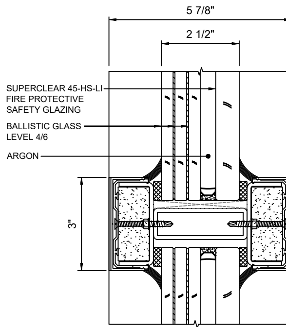
B 8 HORIZONTAL MULLION DETAIL WITH SUPERCLEAR 45-HS-LI WITH LEVEL 4/6 BALLISTIC GLASS
