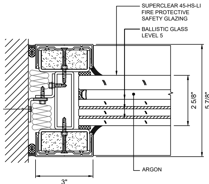
C 10 JAMB DETAIL WITH SUPERCLEAR 45-HS-LI WITH LEVEL 5 BALLISTIC GLASS
