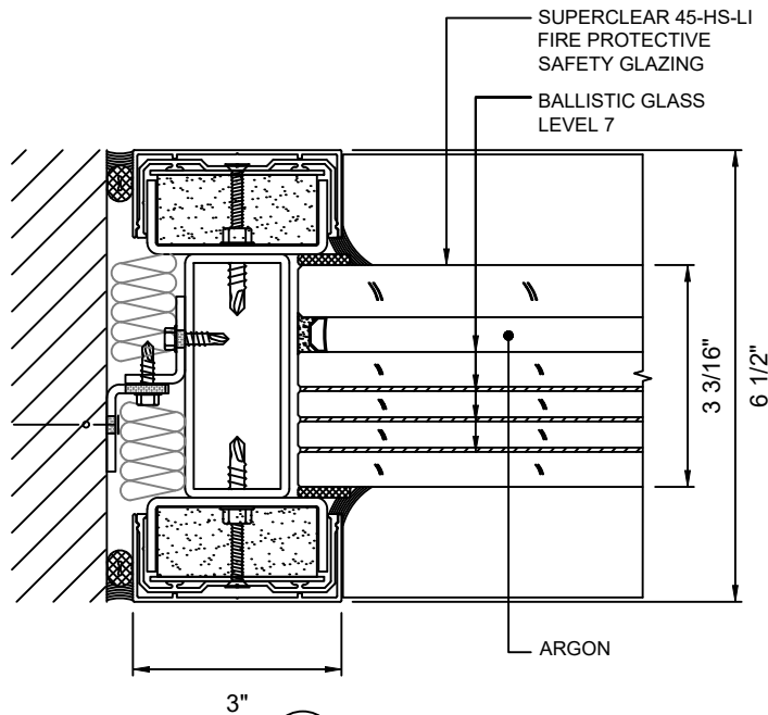
D 11 JAMB DETAIL WITH SUPERCLEAR 45-HS-LI WITH LEVEL 7 BALLISTIC GLASS
