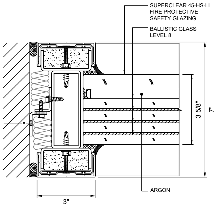
E 11 JAMB DETAIL WITH SUPERCLEAR 45-HS-LI WITH LEVEL 8 BALLISTIC GLASS
