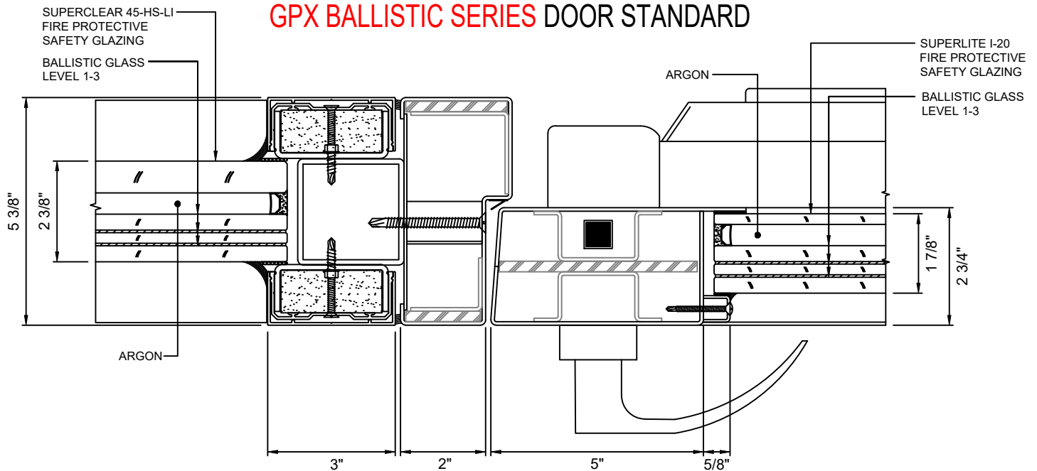
F 16 DOOR JAMB AT LOCK - STANDARD WITH SUPERLITE I-20 & SUPERCLEAR 45-HS-LI WITH LEVEL 1-3 BALLISTIC GLASS
