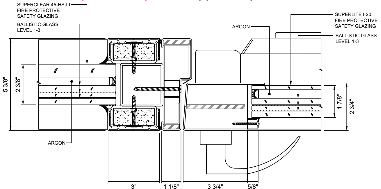
G 16 DOOR JAMB AT LOCK - NARROW STYLE WITH SUPERLITE I-20 & SUPERCLEAR 45-HS-LI WITH LEVEL 1-3 BALLISTIC GLASS
