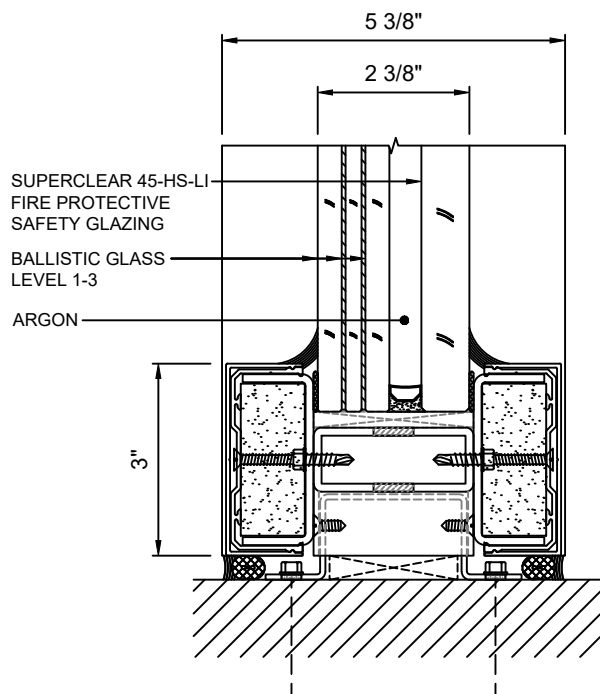
A 6 SILL DETAIL WITH SUPERCLEAR 45-HS-LI WITH LEVEL 1-3 BALLISTIC GLASS
