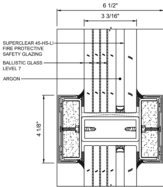
D 9 HORIZONTAL MULLION DETAIL WITH SUPERCLEAR 45-HS-LI WITH LEVEL 7 BALLISTIC GLASS
