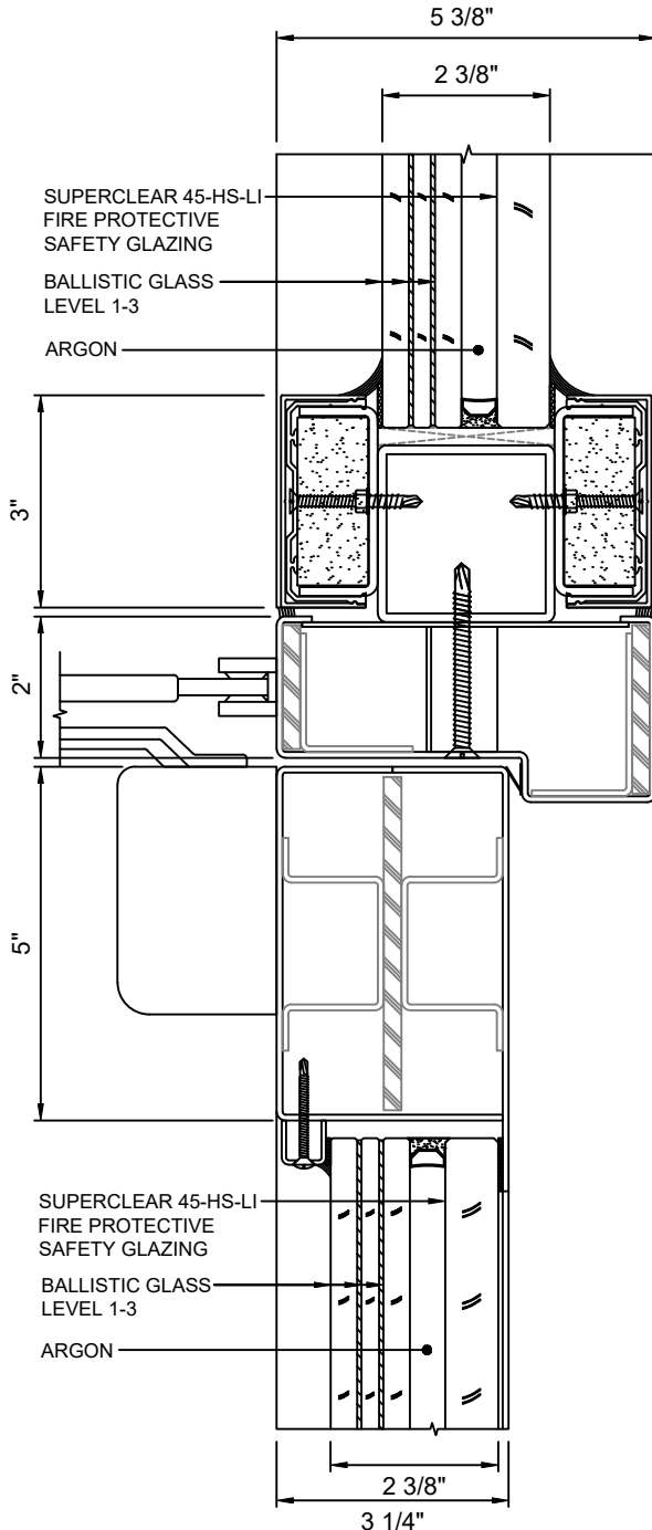
F 19 DOOR TOP RAIL - STANDARD WITH SUPERCLEAR 45-HS-LI WITH LEVEL 1-3 BALLISTIC GLASS
