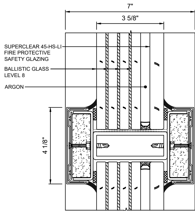
E 9 HORIZONTAL MULLION DETAIL WITH SUPERCLEAR 45-HS-LI WITH LEVEL 8 BALLISTIC GLASS
