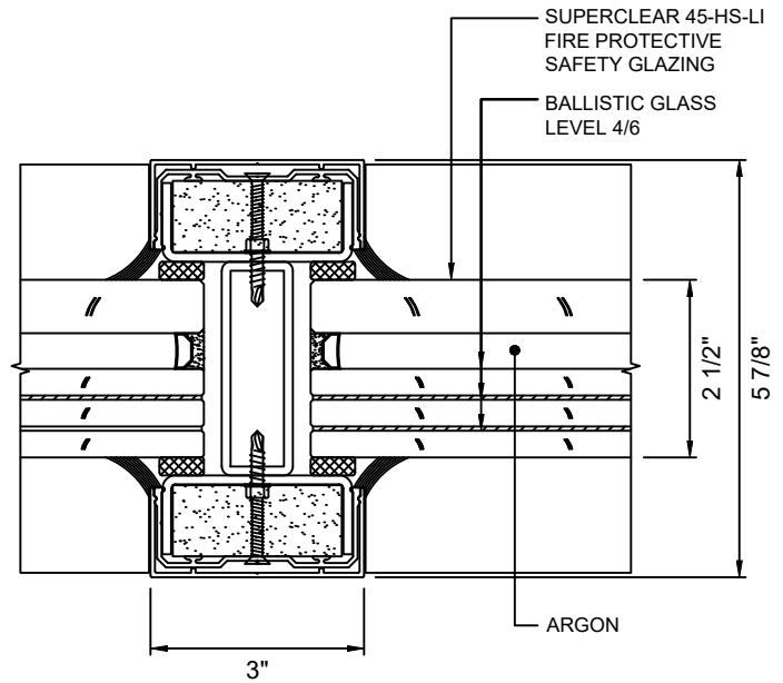
B 12 VERTICAL MULLION DETAIL WITH SUPERCLEAR 45-HS-LI WITH LEVEL 4/6 BALLISTIC GLASS
