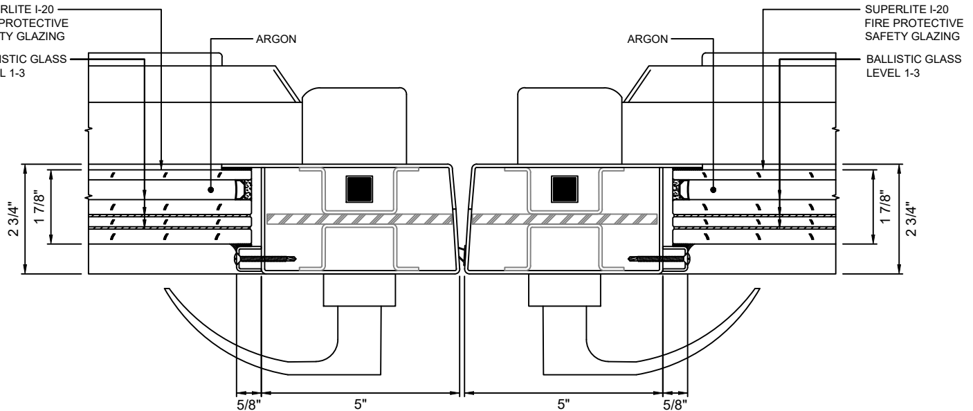
F 18 MEETING STILES - STANDARD WITH SUPERLITE I-20 WITH LEVEL 1-3 BALLISTIC GLASS
