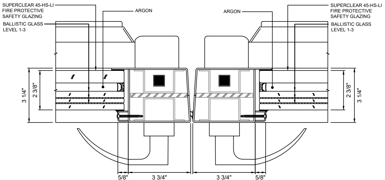
G 23 MEETING STILES - NARROW STYLE WITH SUPERCLEAR 45-HS-LI WITH LEVEL 1-3 BALLISTIC GLASS
