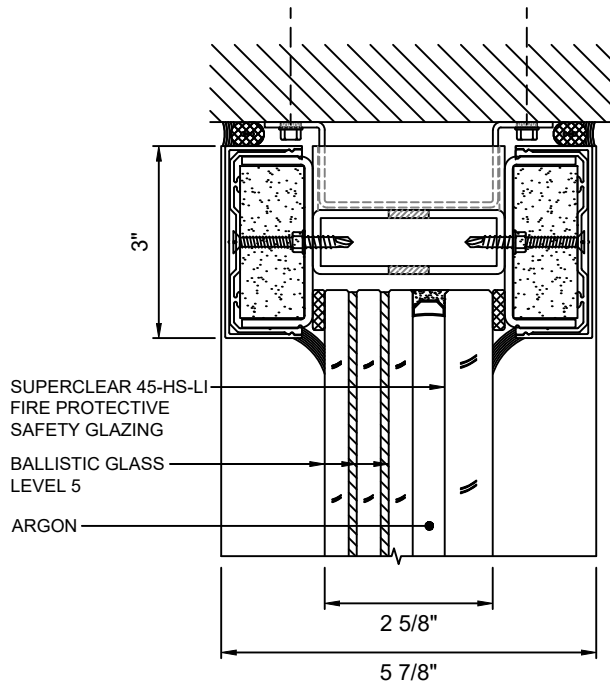
C 4 HEAD DETAIL WITH SUPERCLEAR 45-HS-LI WITH LEVEL 5 BALLISTIC GLASS
