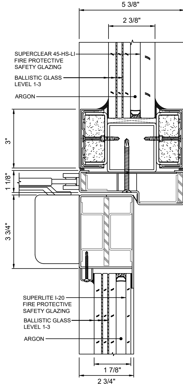
G 14 DOOR TOP RAIL - NARROW STYLE WITH SUPERLITE I-20 & SUPERCLEAR 45-HS-LI WITH LEVEL 1-3 BALLISTIC GLASS
