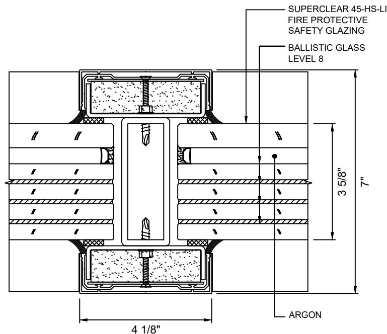
E 13 VERTICAL MULLION DETAIL WITH SUPERCLEAR 45-HS-LI WITH LEVEL 8 BALLISTIC GLASS
