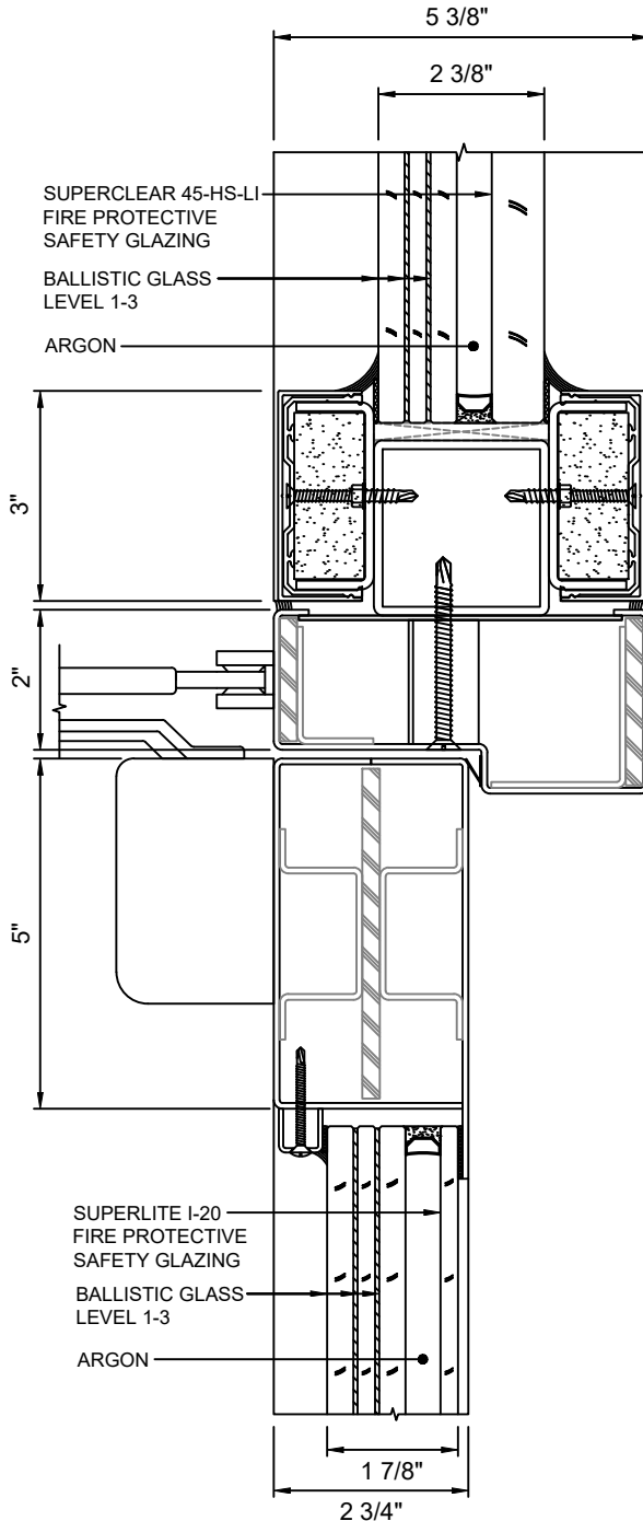
F 14 DOOR TOP RAIL - STANDARD WITH SUPERLITE I-20 & SUPERCLEAR 45-HS-LI WITH LEVEL 1-3 BALLISTIC GLASS
