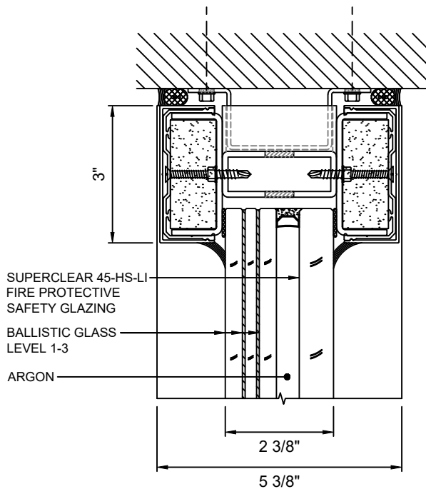
A 4 HEAD DETAIL WITH SUPERCLEAR 45-HS-LI WITH LEVEL 1-3 BALLISTIC GLASS
