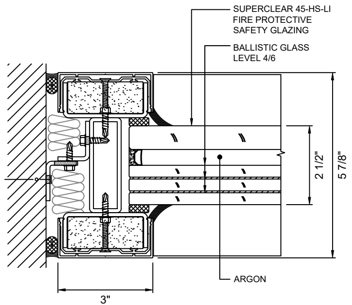
B 10 JAMB DETAIL WITH SUPERCLEAR 45-HS-LI WITH LEVEL 4/6 BALLISTIC GLASS
