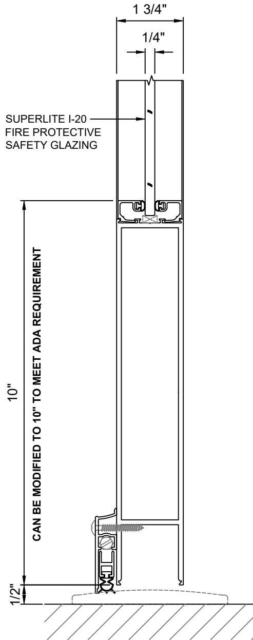
A 3 DOOR BOTTOM RAIL WITH DOOR BOTTOM WITH SUPERLITE I-20
