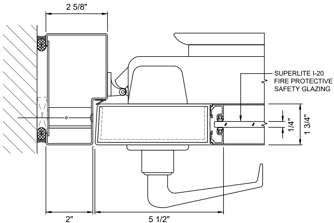
A 4 DOOR JAMB AT LOCK WITH SUPERLITE I-20
