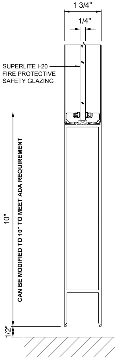
A 3 DOOR BOTTOM RAIL WITHOUT DOOR BOTTOM WITH SUPERLITE I-20
