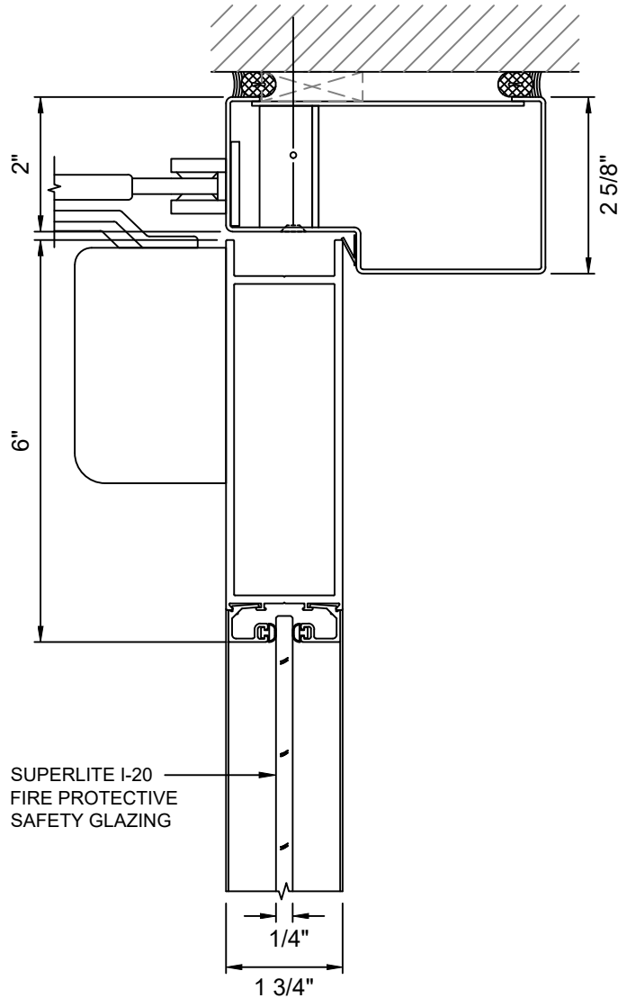
A 2 DOOR TOP RAIL WITH SUPERLITE I-20
