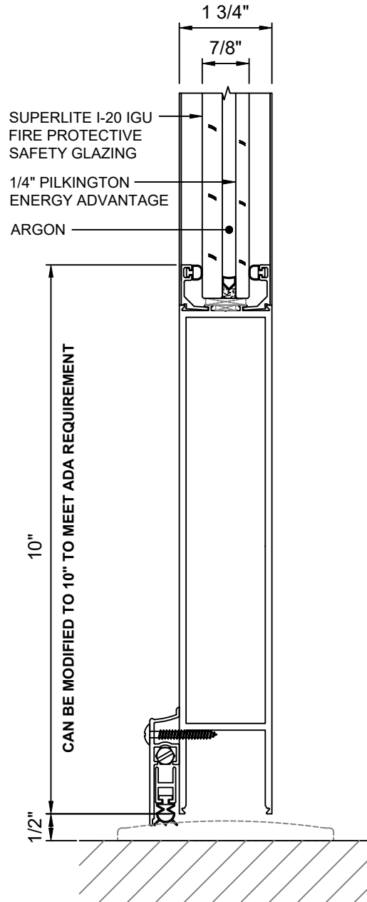
A 3 DOOR BOTTOM RAIL WITH DOOR BOTTOM WITH SUPERLITE I-20 IGU
