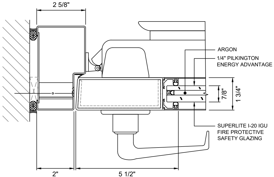
A 4 DOOR JAMB AT LOCK WITH SUPERLITE I-20 IGU
