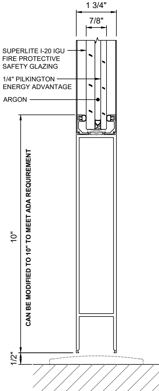
A 3 DOOR BOTTOM RAIL WITHOUT DOOR BOTTOM WITH SUPERLITE I-20 IGU
