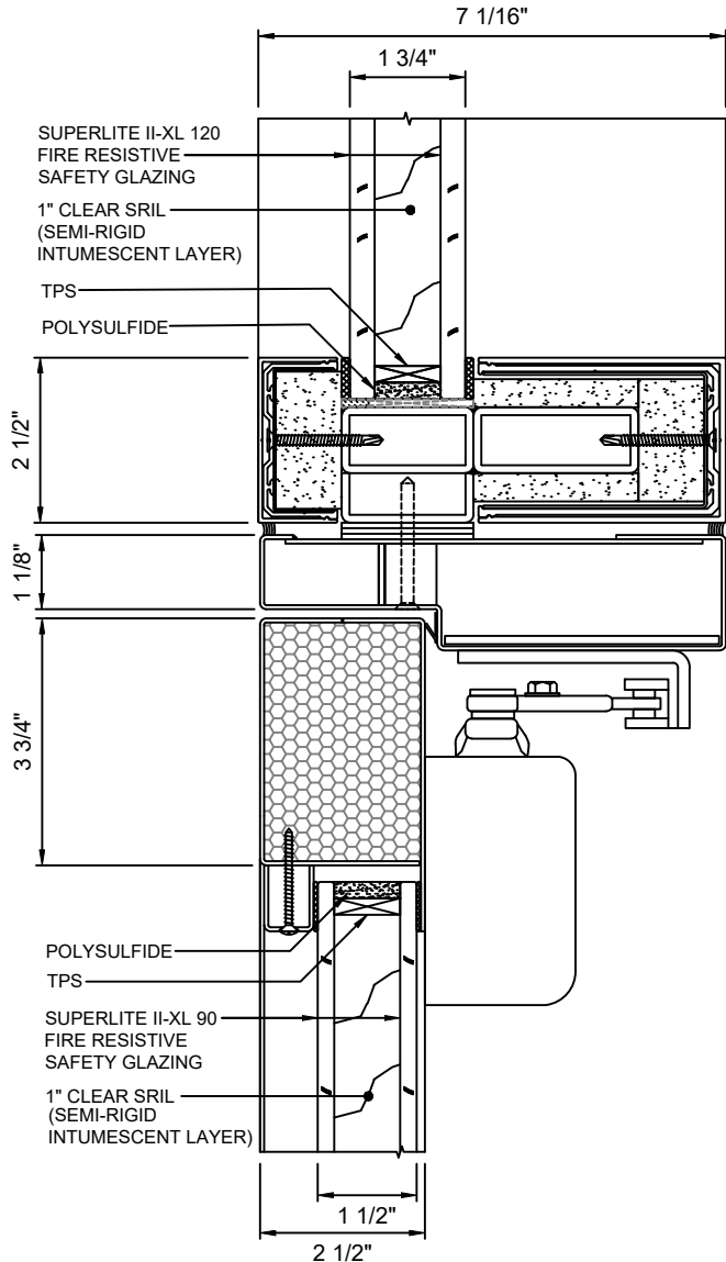
E DOOR TOP RAIL - NARROW STYLE 9 WITH SUPERLITE II-XL 90 & II-XL 120
