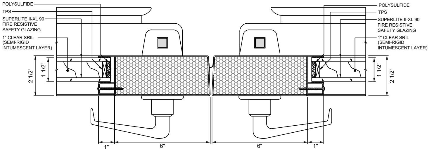
D MEETING STILES - STANDARD 13 WITH SUPERLITE II-XL 90
