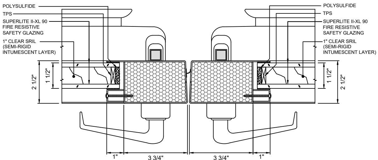
E MEETING STILES - NARROW STYLE 13 WITH SUPERLITE II-XL 90
