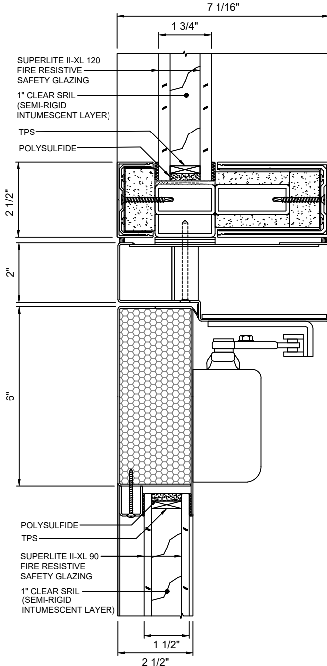
D DOOR TOP RAIL - STANDARD 9 WITH SUPERLITE II-XL 90 & II-XL 120
