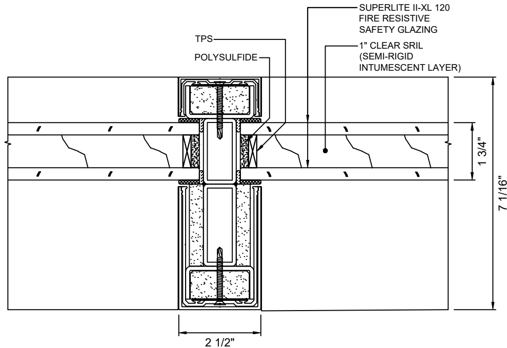
(A) 7 VERTICAL MULLION DETAIL WITH SUPERLITE II-XL 120
