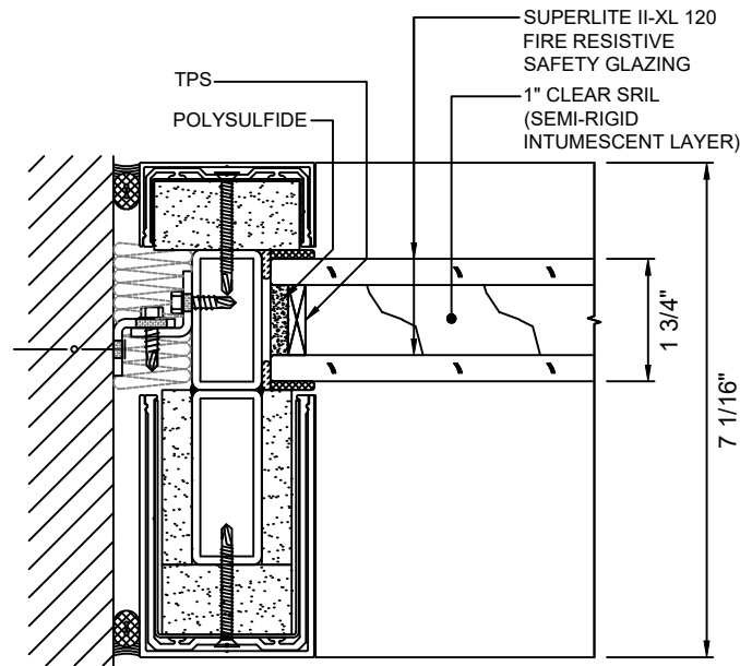
(A) JAMB DETAIL 6 WITH SUPERLITE II-XL 120
