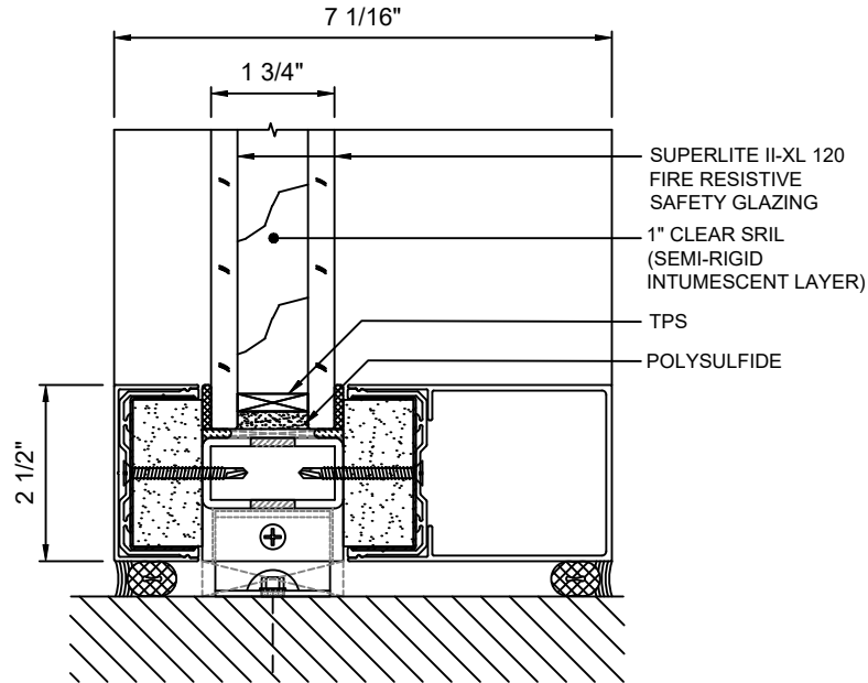
A SILL DETAIL 5 WITH SUPERLITE II-XL 120
