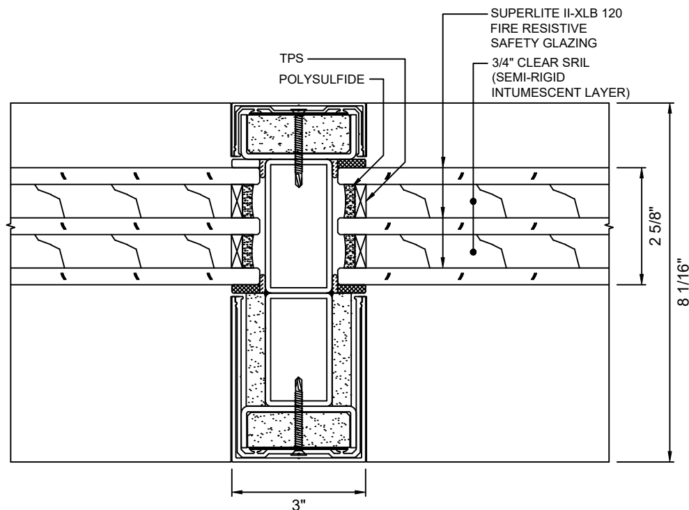
(B) 7 VERTICAL MULLION DETAIL WITH SUPERLITE II-XLB 120
