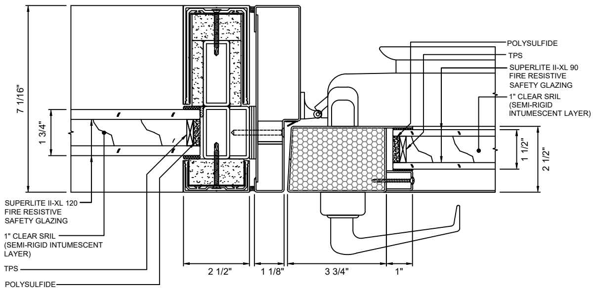
E DOOR JAMB AT LOCK - NARROW STYLE WITH SUPERLITE II-XL 90 & II-XL 120
