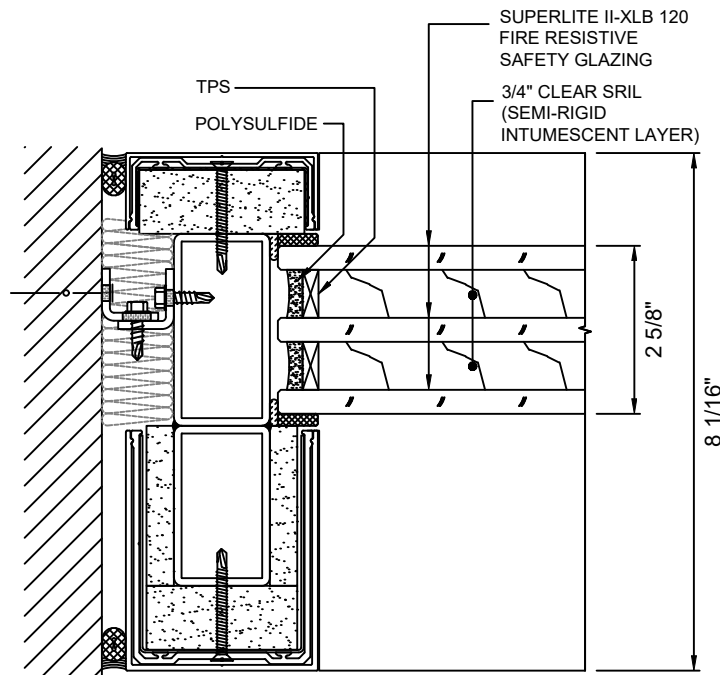
(B) JAMB DETAIL 6 WITH SUPERLITE II-XLB 120
