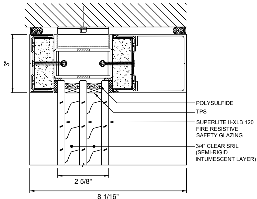
B HEAD DETAIL 3 WITH SUPERLITE II-XLB 120
