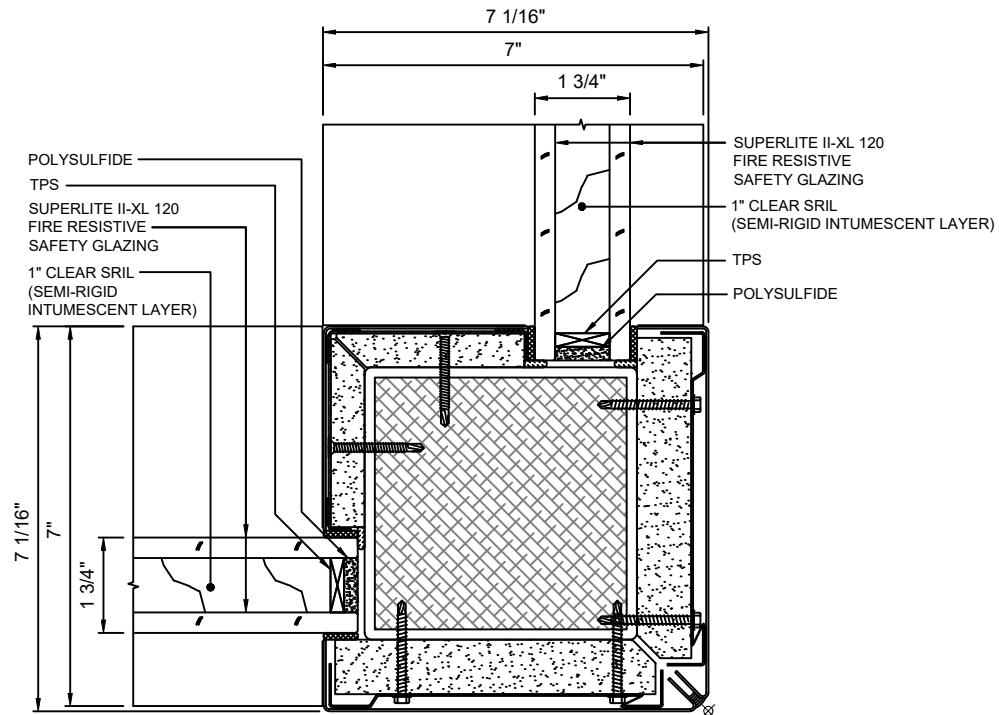
A 8 90° CORNER DETAIL WITH SUPERLITE II-XL 120
