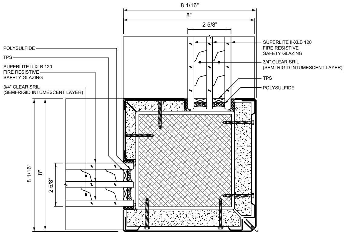
B 8 90° CORNER DETAIL WITH SUPERLITE II-XLB 120
