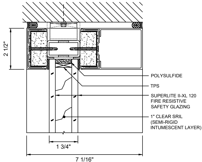
A HEAD DETAIL 3 WITH SUPERLITE II-XL 120
