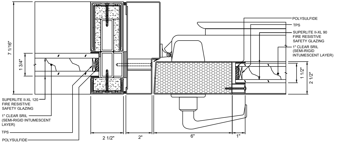
D DOOR JAMB AT LOCK - STANDARD WITH SUPERLITE II-XL 90 & II-XL 120
