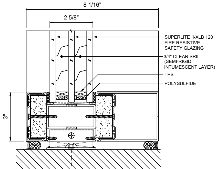
B SILL DETAIL 5 WITH SUPERLITE II-XLB 120
