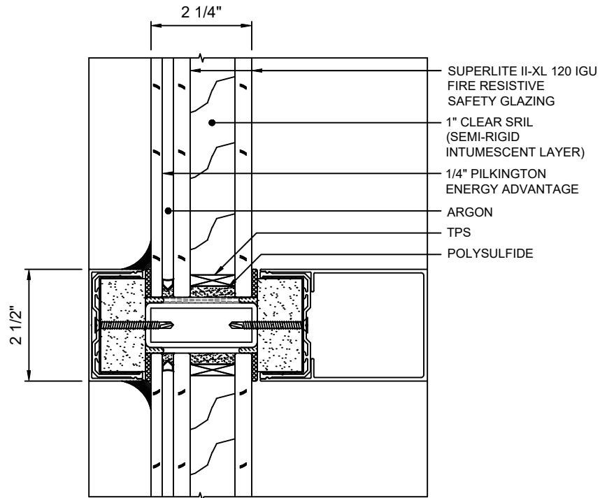
(A) 4 HORIZONTAL MULLION WITH SUPERLITE II-XL 120 IGU
