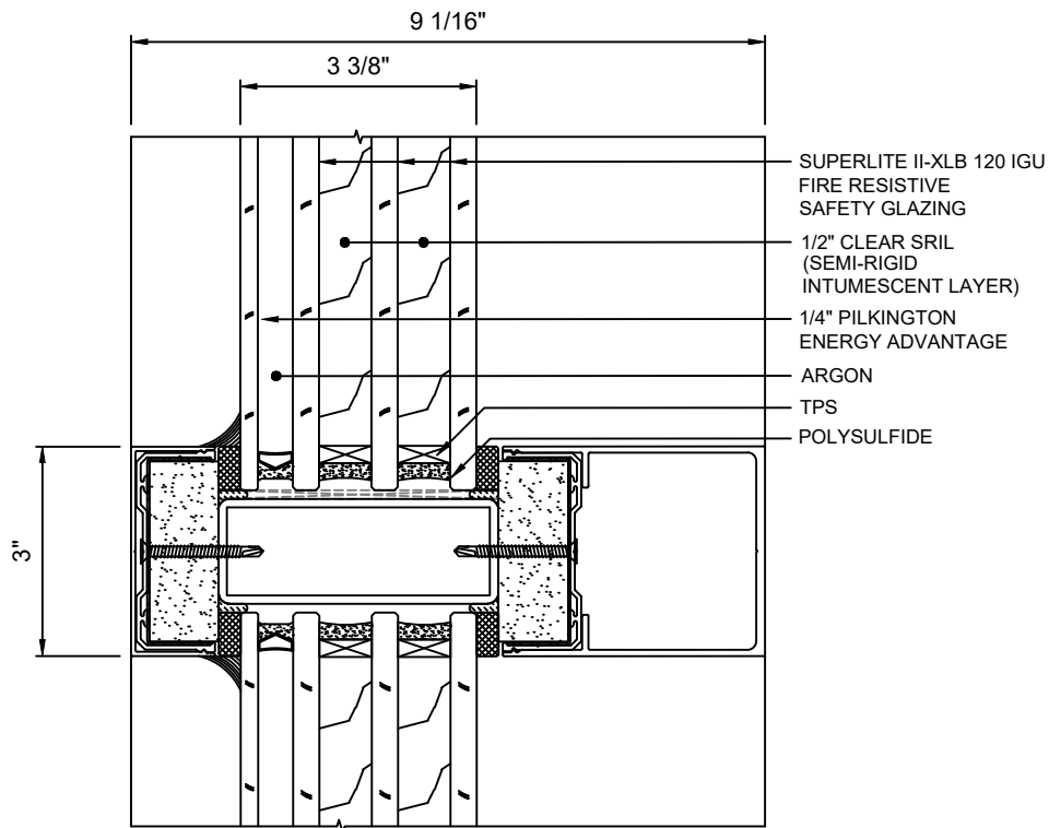
(B) 4 HORIZONTAL MULLION WITH SUPERLITE II-XLB 120 IGU
