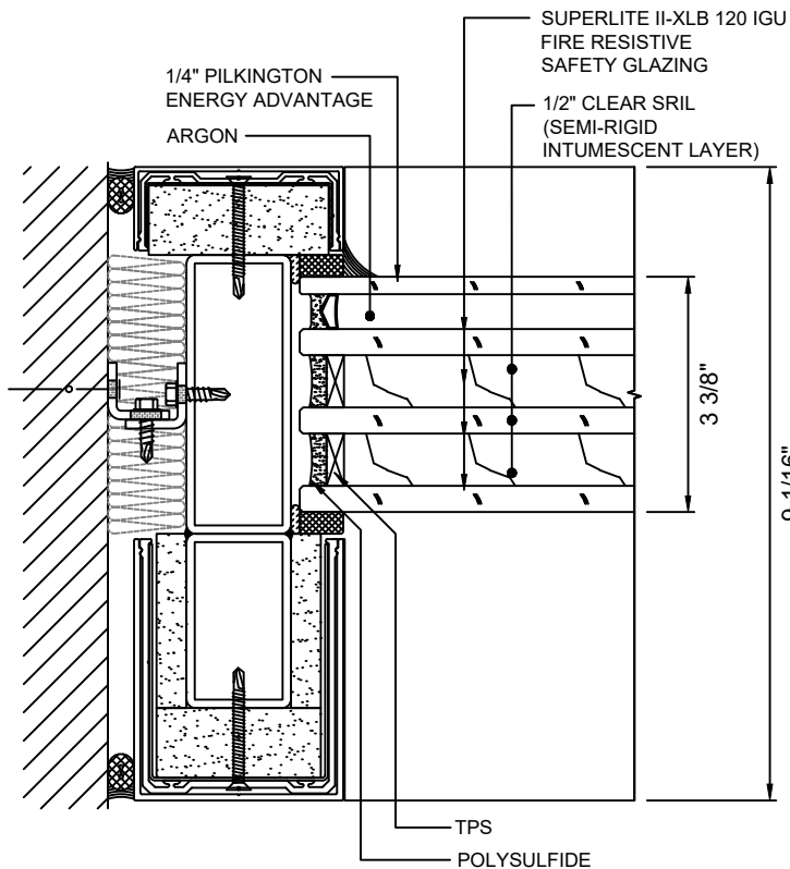
B 6 JAMB DETAIL WITH SUPERLITE II-XLB 120 IGU
