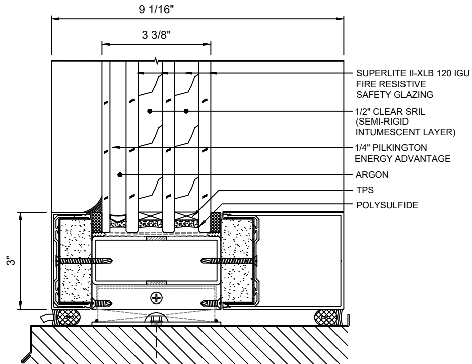
B 5 SILL DETAIL WITH SUPERLITE II-XLB 120 IGU
