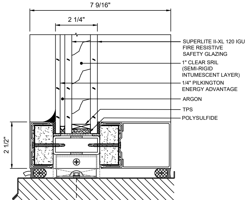
A 5 SILL DETAIL WITH SUPERLITE II-XL 120 IGU
