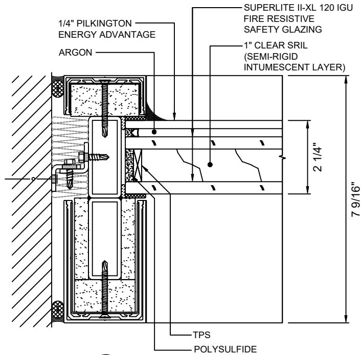
A 6 JAMB DETAIL WITH SUPERLITE II-XL 120 IGU
