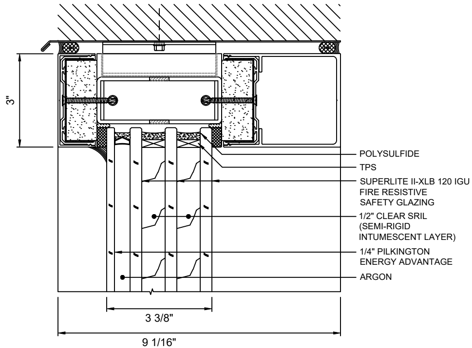
B 3 HEAD DETAIL WITH SUPERLITE II-XLB 120 IGU
