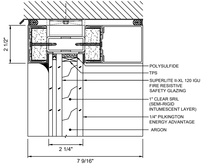
A 3 HEAD DETAIL WITH SUPERLITE II-XL 120 IGU
