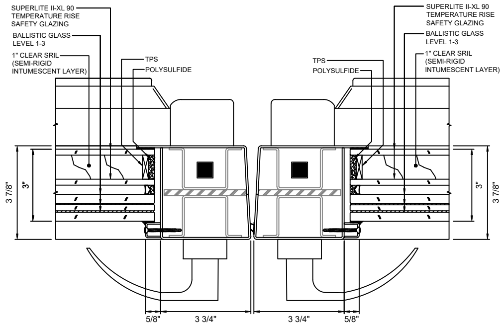
G 17 MEETING STILES - NARROW STYLE WITH SUPERLITE II-XL 90 WITH LEVEL 1-3 BALLISTIC GLASS
