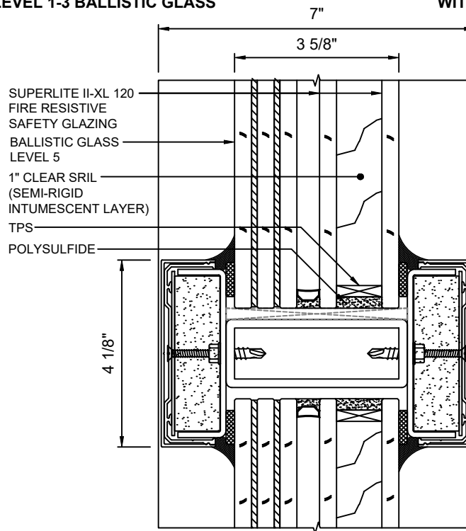
C 5 HORIZONTAL MULLION WITH SUPERLITE II-XL 120 WITH LEVEL 5 BALLISTIC GLASS
