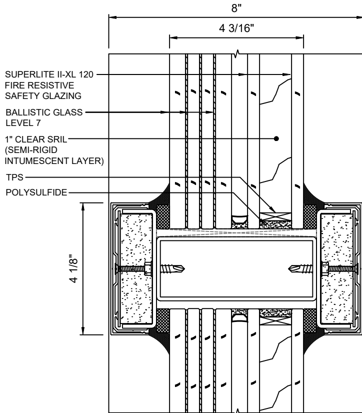
D 6 HORIZONTAL MULLION WITH SUPERLITE II-XL 120 WITH LEVEL 7 BALLISTIC GLASS
