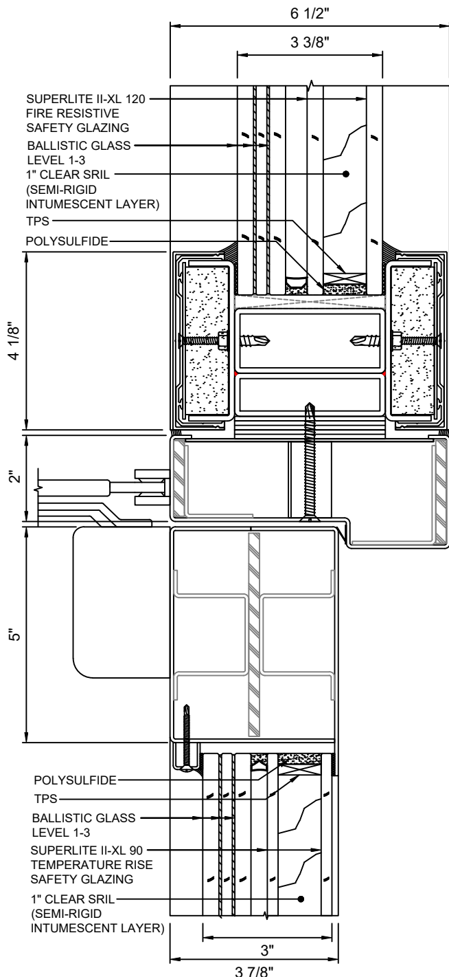
F 13 DOOR TOP RAIL - STANDARD WITH SUPERLITE II-XL 120 & SUPERLITE II-XL 90 WITH LEVEL 1-3 BALLISTIC GLASS
