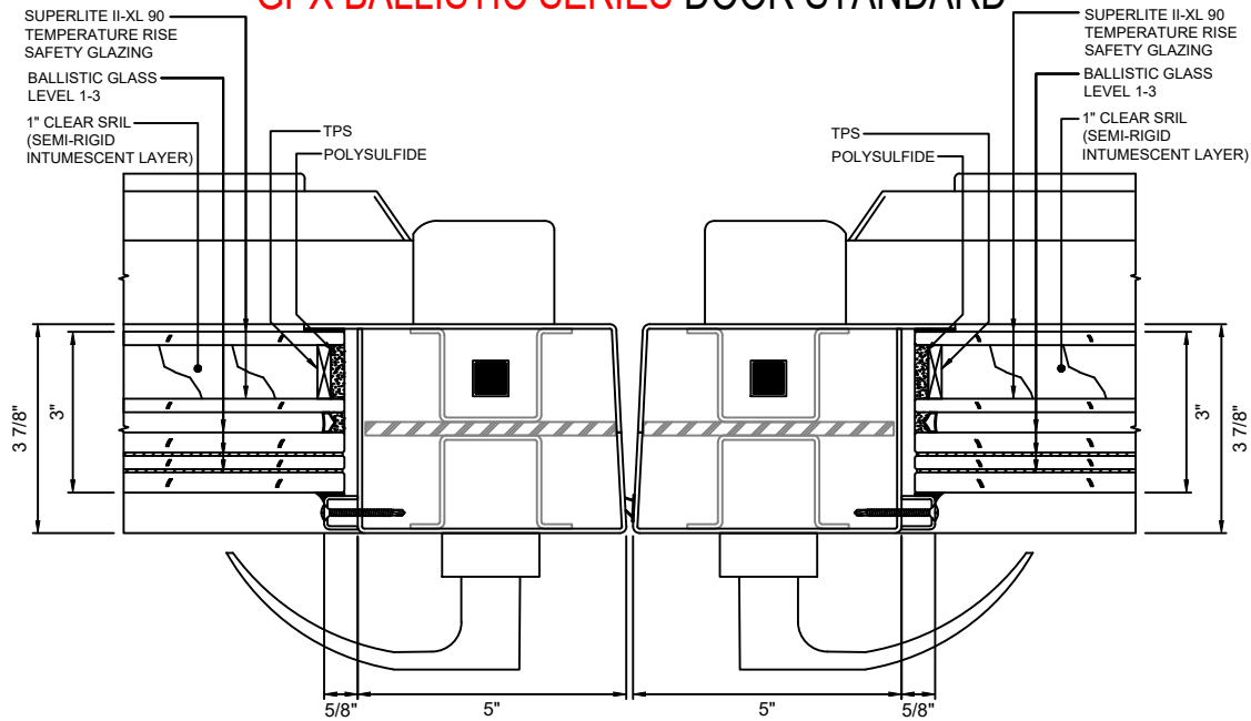
F 17 MEETING STILES - STANDARD WITH SUPERLITE II-XL 90 WITH LEVEL 1-3 BALLISTIC GLASS
