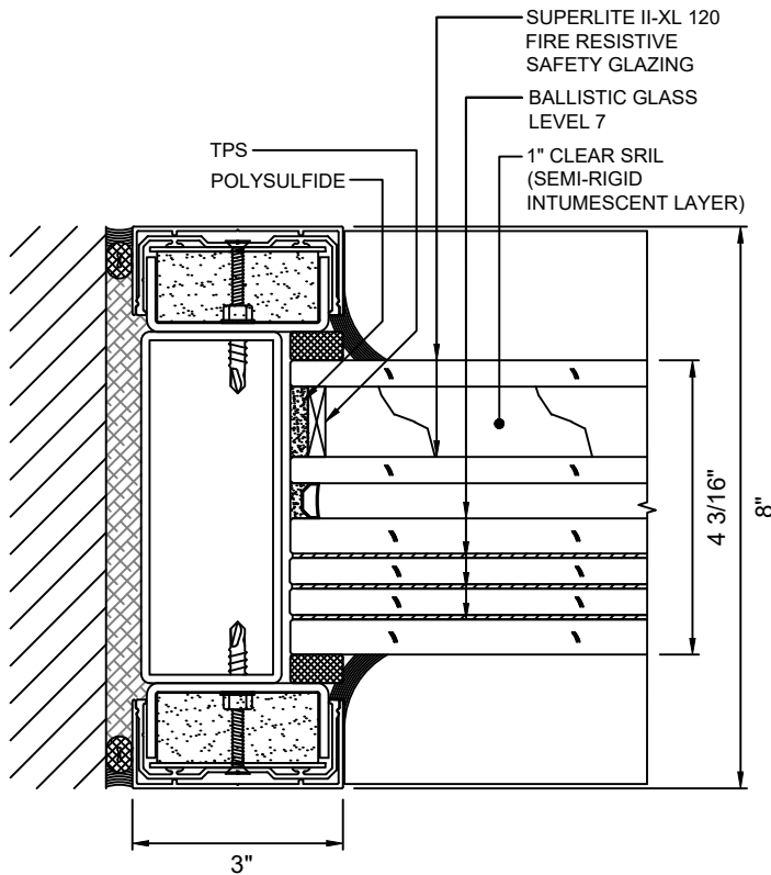
D 10 JAMB DETAIL WITH SUPERLITE II-XL 120 WITH LEVEL 7 BALLISTIC GLASS
