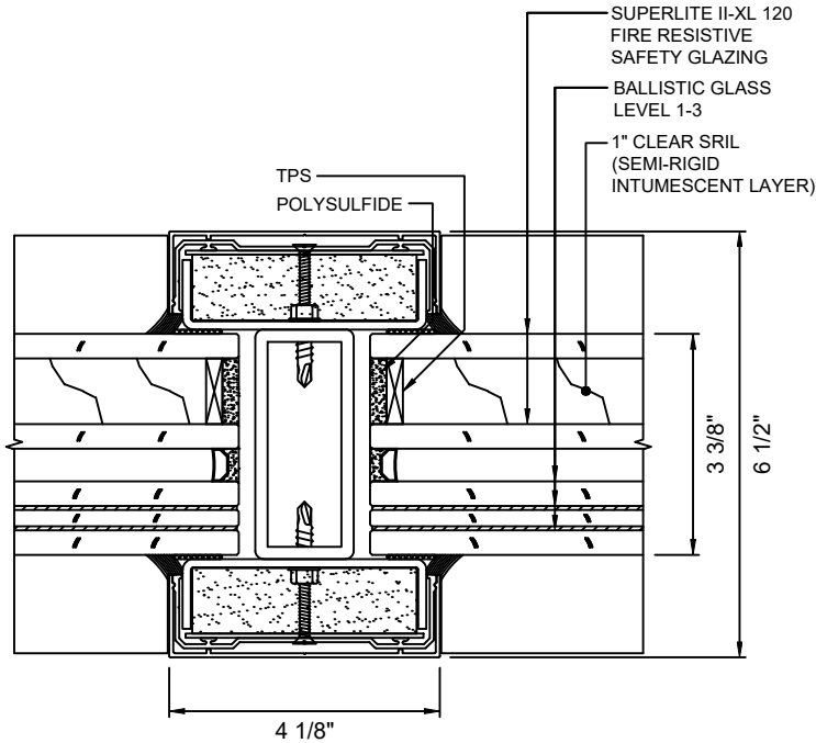
A 11 VERTICAL MULLION DETAIL WITH SUPERLITE II-XL 120 WITH LEVEL 1-3 BALLISTIC GLASS
