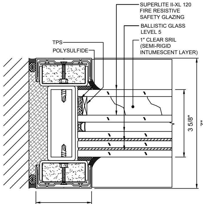
C 9 JAMB DETAIL WITH SUPERLITE II-XL 120 WITH LEVEL 5 BALLISTIC GLASS
