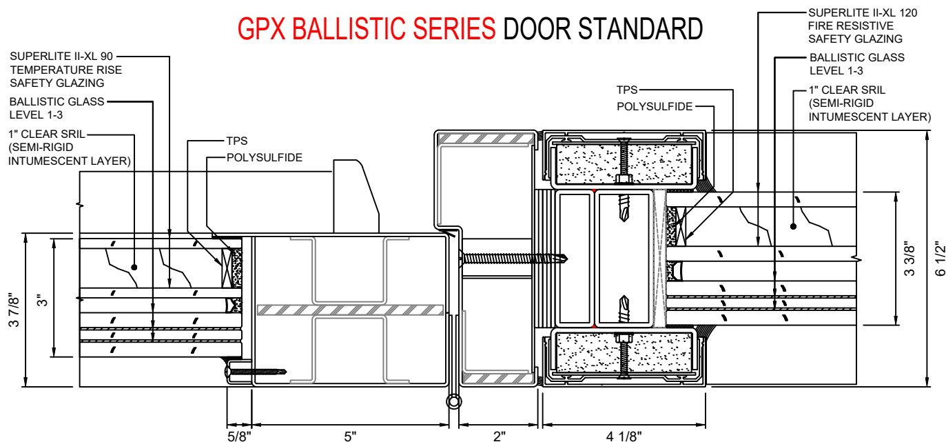
F 16 DOOR JAMB AT HINGE - STANDARD WITH SUPERLITE II-XL 120 & SUPERLITE II-XL 90 WITH LEVEL 1-3 BALLISTIC GLASS
