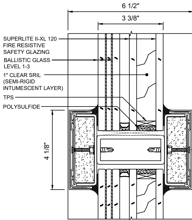
A 5 HORIZONTAL MULLION WITH SUPERLITE II-XL 120 WITH LEVEL 1-3 BALLISTIC GLASS
