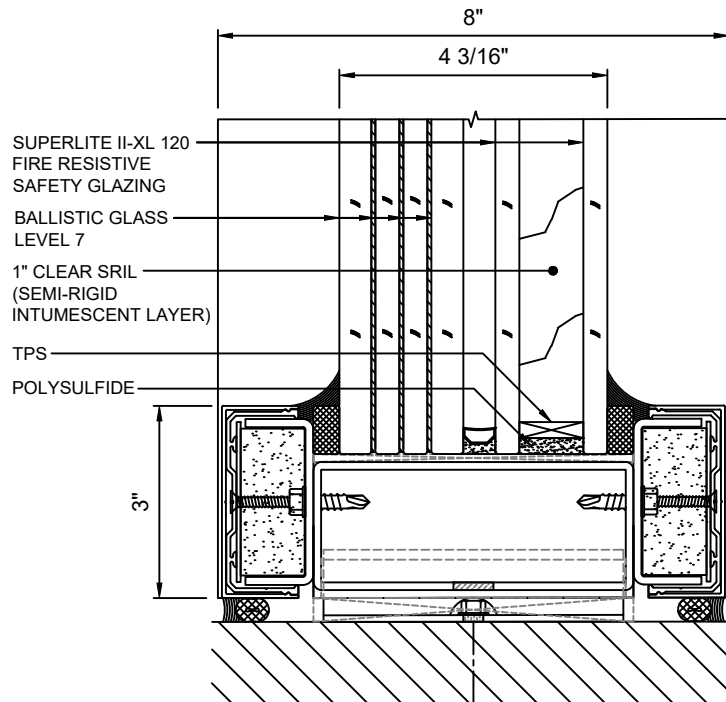
D 8 SILL DETAIL WITH SUPERLITE II-XL 120 WITH LEVEL 7 BALLISTIC GLASS
