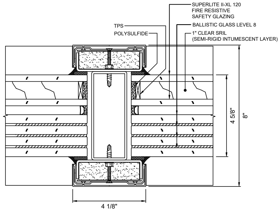
E 12 VERTICAL MULLION DETAIL WITH SUPERLITE II-XL 120 WITH LEVEL 8 BALLISTIC GLASS
