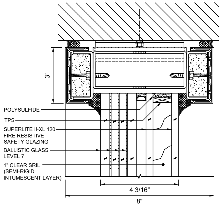
(D) 4 HEAD DETAIL WITH SUPERLITE II-XL 120 WITH LEVEL 7 BALLISTIC GLASS
