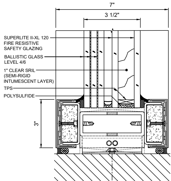
B 7 SILL DETAIL WITH SUPERLITE II-XL 120 WITH LEVEL 4/6 BALLISTIC GLASS
