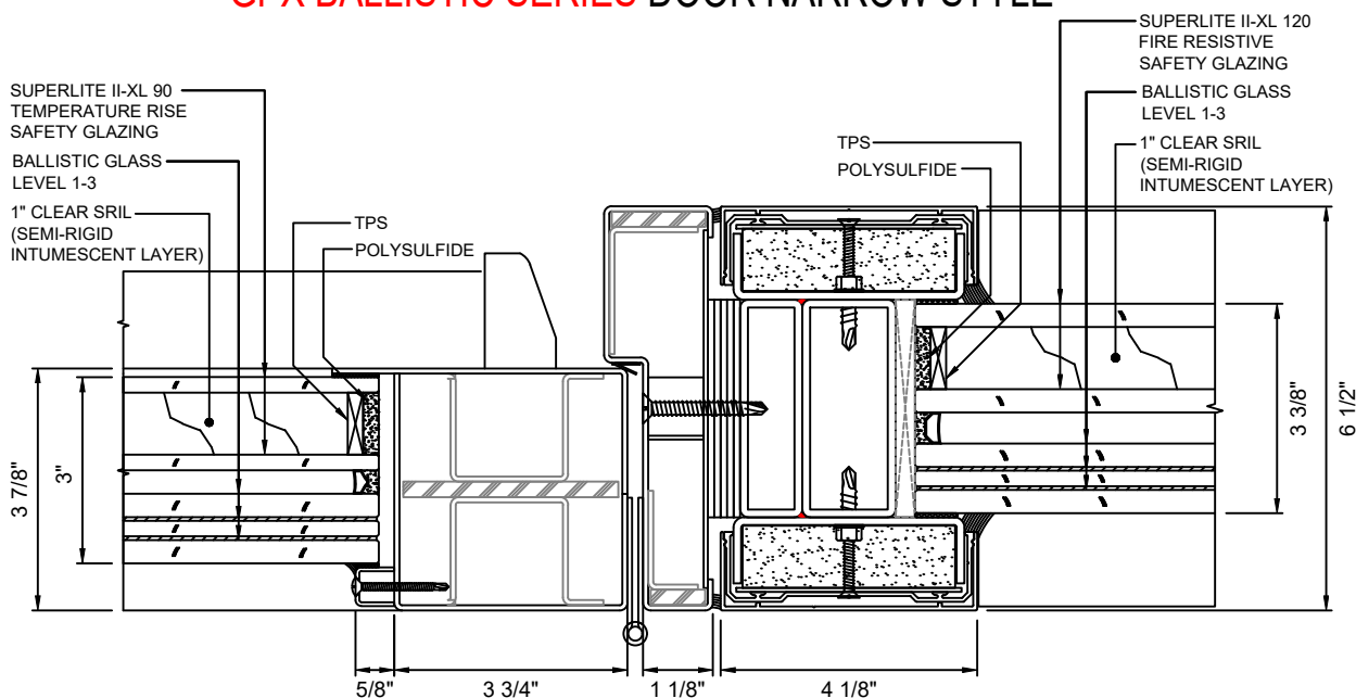
G 16 DOOR JAMB AT HINGE - NARROW STYLE WITH SUPERLITE II-XL 120 & SUPERLITE II-XL 90 WITH LEVEL 1-3 BALLISTIC GLASS
