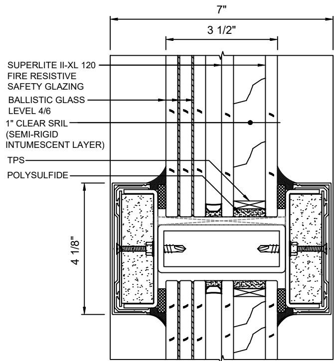
B 5 HORIZONTAL MULLION WITH SUPERLITE II-XL 120 WITH LEVEL 4/6 BALLISTIC GLASS
