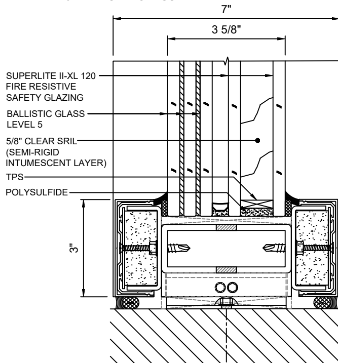
C 7 SILL DETAIL WITH SUPERLITE II-XL 120 WITH LEVEL 5 BALLISTIC GLASS
