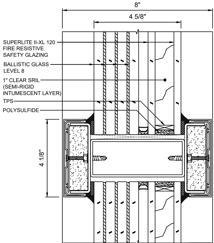
E 6 HORIZONTAL MULLION WITH SUPERLITE II-XL 120 WITH LEVEL 8 BALLISTIC GLASS
