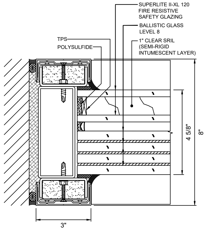
E 10 JAMB DETAIL WITH SUPERLITE II-XL 120 WITH LEVEL 8 BALLISTIC GLASS
