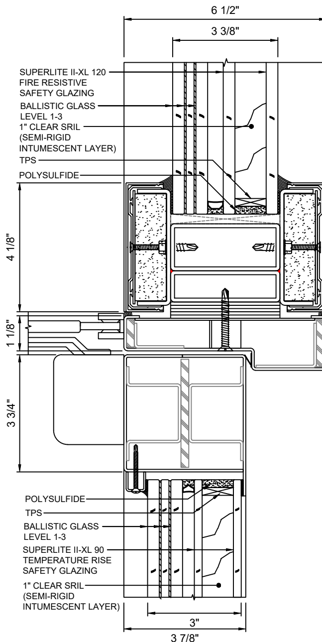
G 13 DOOR TOP RAIL - STANDARD WITH SUPERLITE II-XL 120 & SUPERLITE II-XL 90 WITH LEVEL 1-3 BALLISTIC GLASS
