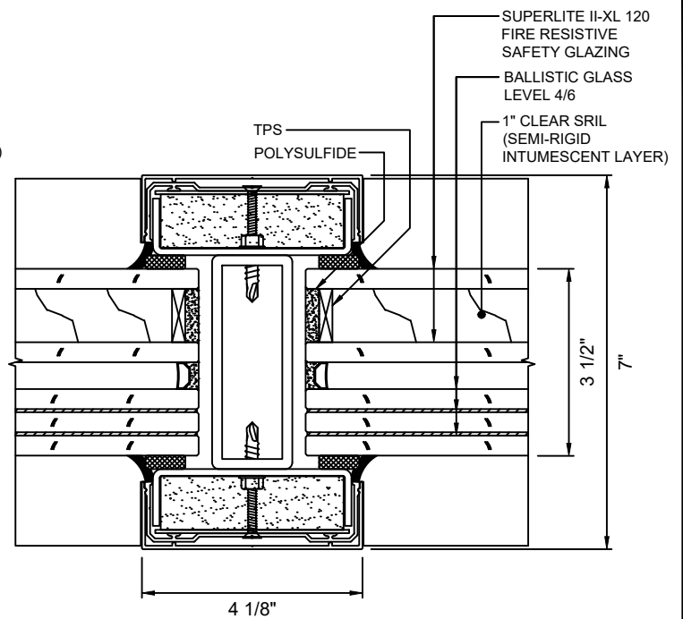
B 11 VERTICAL MULLION DETAIL WITH SUPERLITE II-XL 120 WITH LEVEL 4/6 BALLISTIC GLASS
