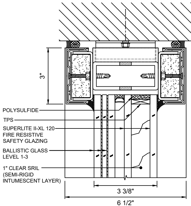
A 3 HEAD DETAIL WITH SUPERLITE II-XL 120 WITH LEVEL 1-3 BALLISTIC GLASS
