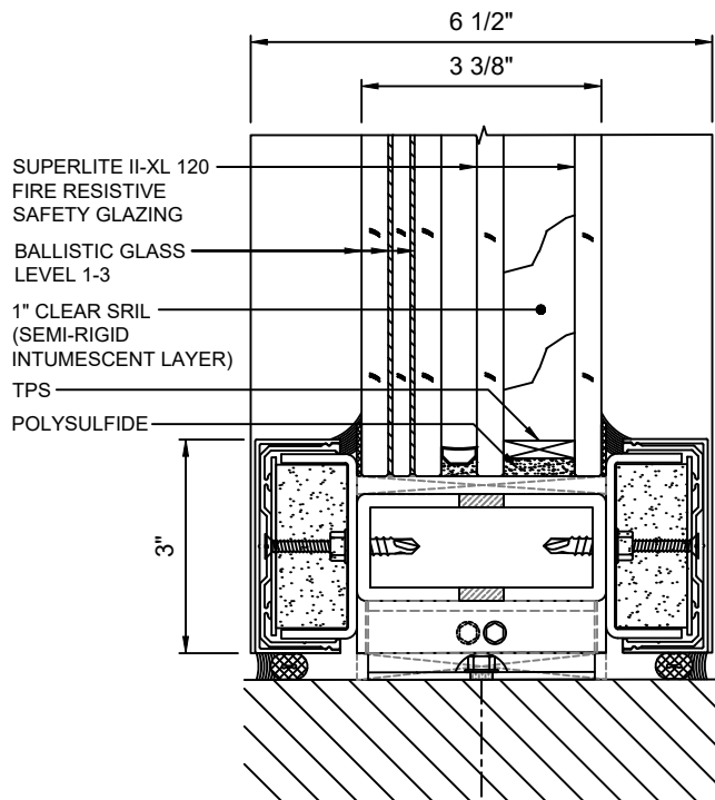
A 7 SILL DETAIL WITH SUPERLITE II-XL 120 WITH LEVEL 1-3 BALLISTIC GLASS
