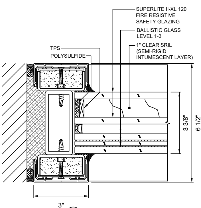
A 9 JAMB DETAIL WITH SUPERLITE II-XL 120 WITH LEVEL 1-3 BALLISTIC GLASS
