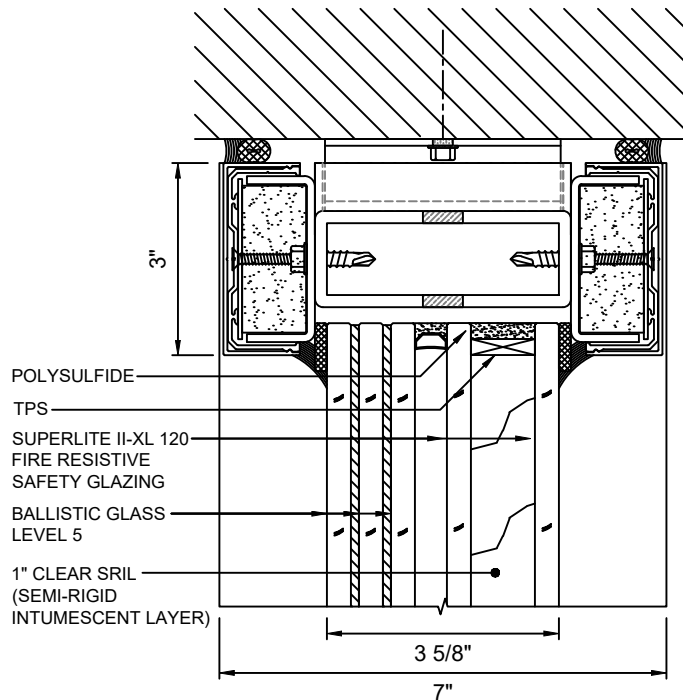
C 3 HEAD DETAIL WITH SUPERLITE II-XL 120 WITH LEVEL 5 BALLISTIC GLASS
