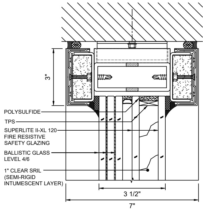
B 3 HEAD DETAIL WITH SUPERLITE II-XL 120 WITH LEVEL 4/6 BALLISTIC GLASS
