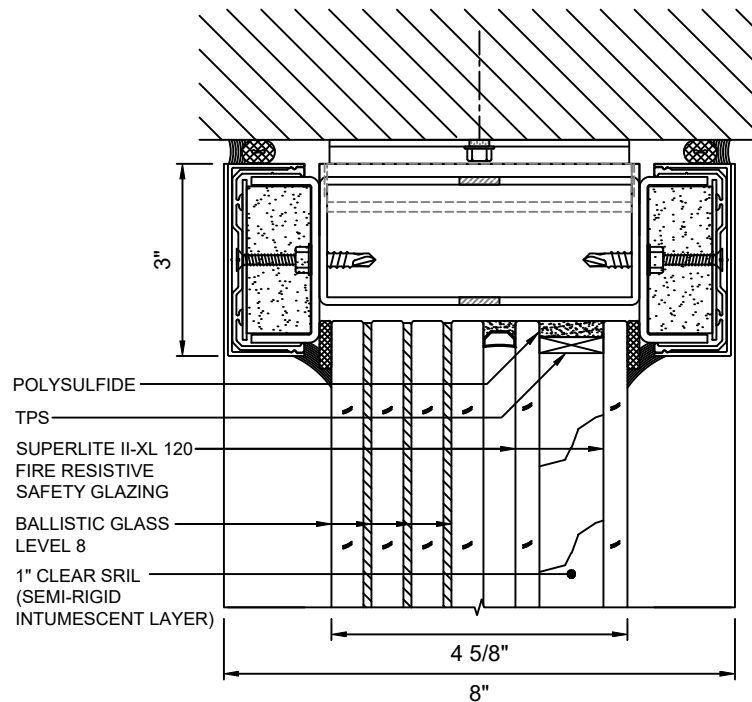
(E) 4 HEAD DETAIL WITH SUPERLITE II-XL 120 WITH LEVEL 8 BALLISTIC GLASS
