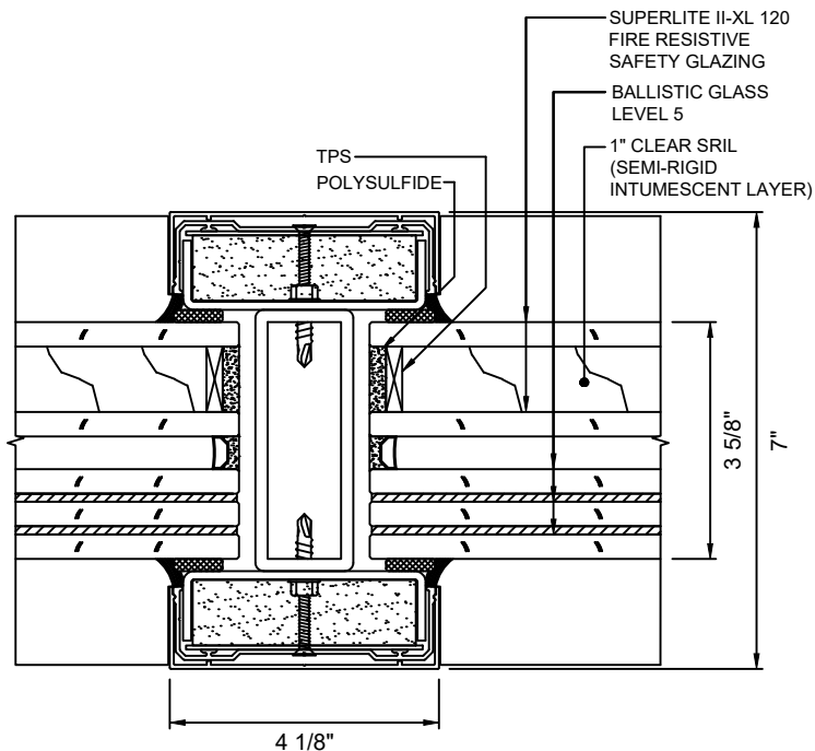
C 11 VERTICAL MULLION DETAIL WITH SUPERLITE II-XL 120 WITH LEVEL 5 BALLISTIC GLASS
