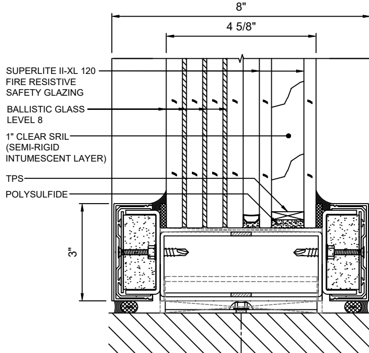
E 8 SILL DETAIL WITH SUPERLITE II-XL 120 WITH LEVEL 8 BALLISTIC GLASS
