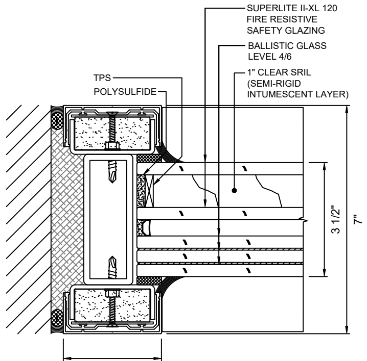
B 9 JAMB DETAIL WITH SUPERLITE II-XL 120 WITH LEVEL 4/6 BALLISTIC GLASS
