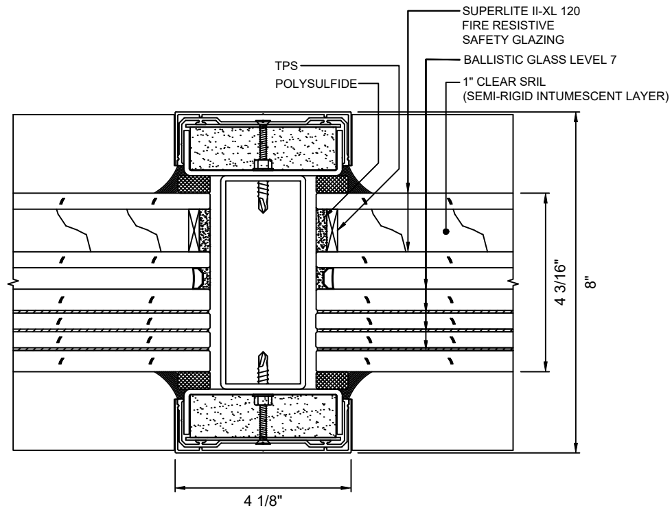
D 12 VERTICAL MULLION DETAIL WITH SUPERLITE II-XL 120 WITH LEVEL 7 BALLISTIC GLASS
