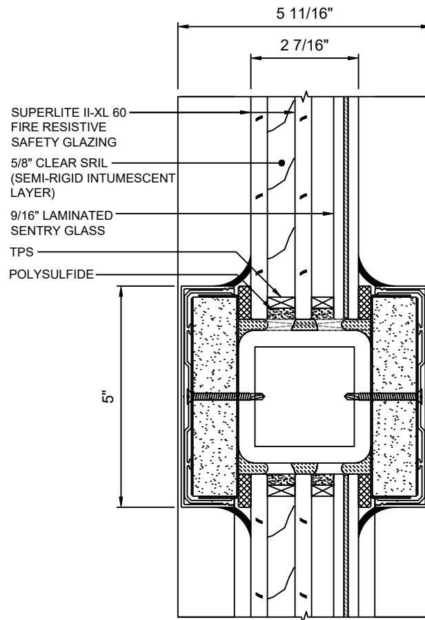
A 4 HORIZONTAL MULLION WITH SUPERLITE II-XL 60
