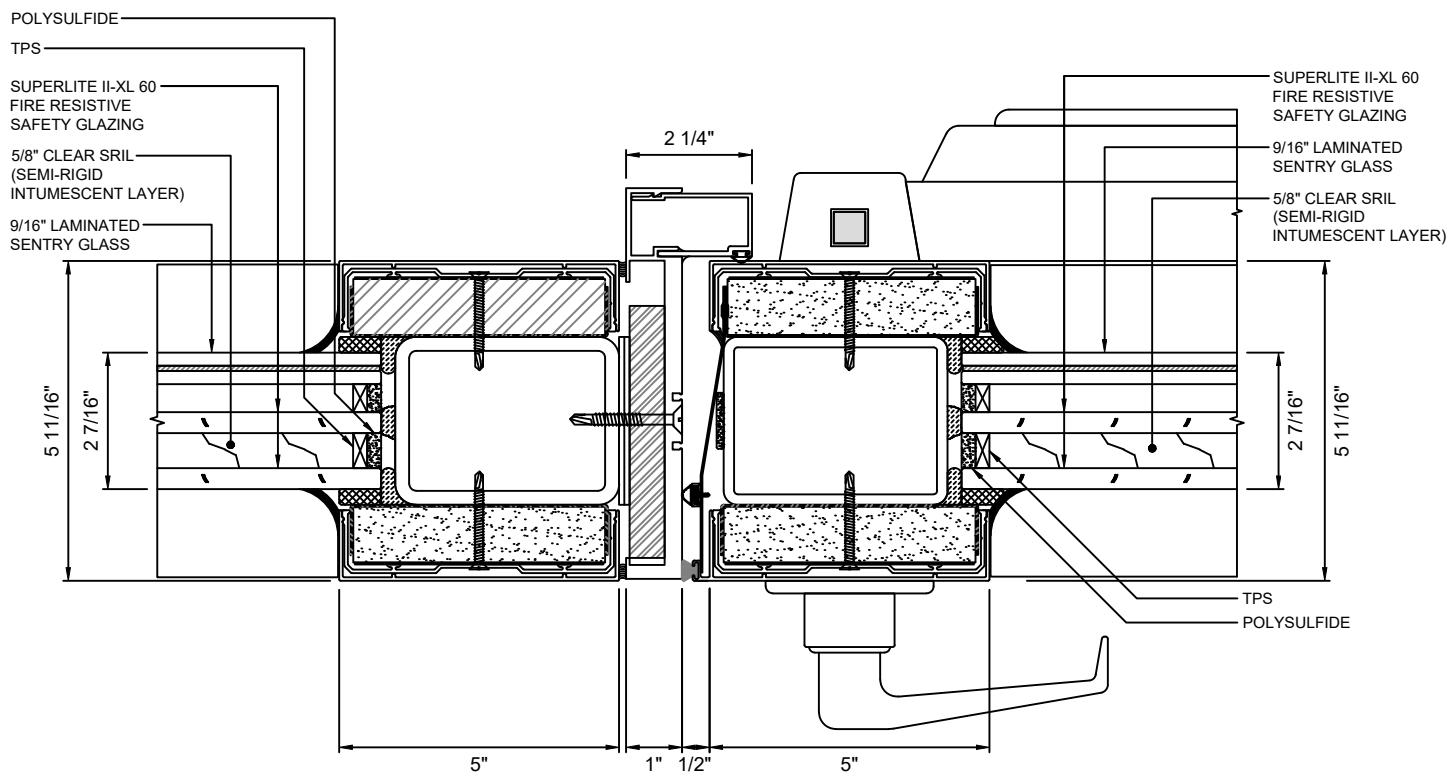
(A) 10 DOOR JAMB AT LOCK WITH SUPERLITE II-XL 60
