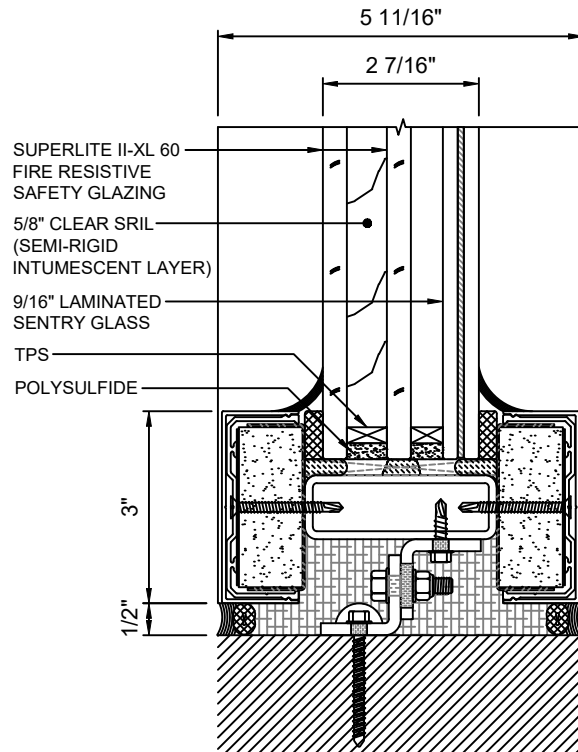
A SILL DETAIL 5 WITH SUPERLITE II-XL 60
