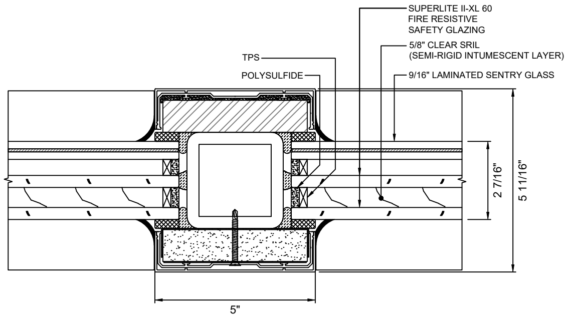
(A) 7 VERTICAL MULLION DETAIL WITH SUPERLITE II-XL 60
