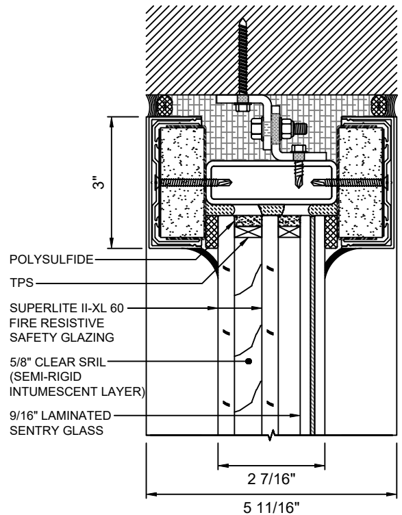
A HEAD DETAIL 3 WITH SUPERLITE II-XL 60
