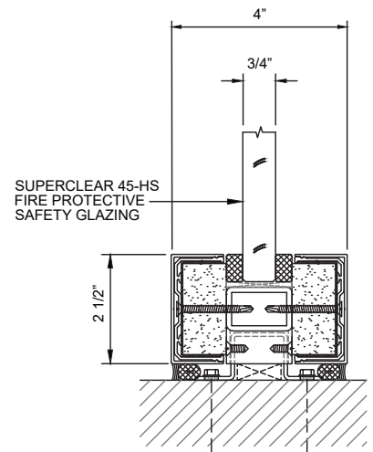
SILL DETAIL
