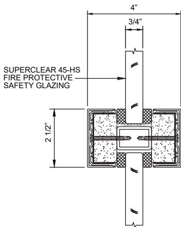
HORIZONTAL MULLION DETAIL
